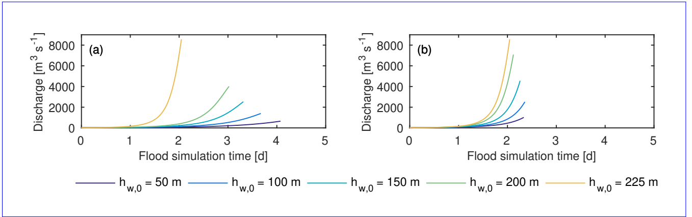
Figure 6. Demonstration of the impact of floating ice on outburst flood hydrographs for an ice dam height of 250 m (year 50 in the glacier simulations). The glacier geometry and basin shape (box) are the same in all simulations. In (a), the initial water height, h_{w,0} , is varied and there is no floating ice in the basin. The initial water heights are the same in (b) except that enough floating ice is added to force the ice dam flotation. For h_{w,0} = 225 \text{ m} , the water level is equal to initially be at flotation depth so there is no remnant ice and the curves in (a) and (b) are the same. Note that the modeled hydrographs do not include the rapidly falling limb of the floods because the outburst flood model is not capable of handling open channel flow, which occurs when the basin water level drops below the conduit roof.
