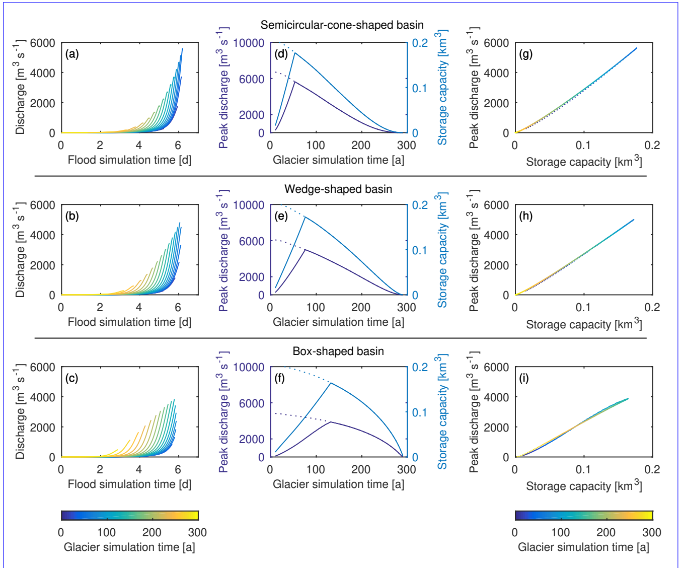
Figure 7. Comparison of annual outburst floods for semicircular-cone-, wedge-, and box-shaped basins for the simulations in which the basin is initially at flotation depth . Left panels (a,b,c): annual outburst flood hydrographs when the basin is initially filled with ice. Middle panels (d,e,f): peak discharge and storage capacity over time. The fork in the early years of the simulations represents ice-filled (solid line) and ice-free (dotted line) scenarios. Right panels (g,h,i): Peak discharge vs. storage capacity for the ice-filled scenario. We refer to the timescale of the glacier flow model as “glacier simulation time” and the timescale of the outburst flood model as “flood simulation time”.
