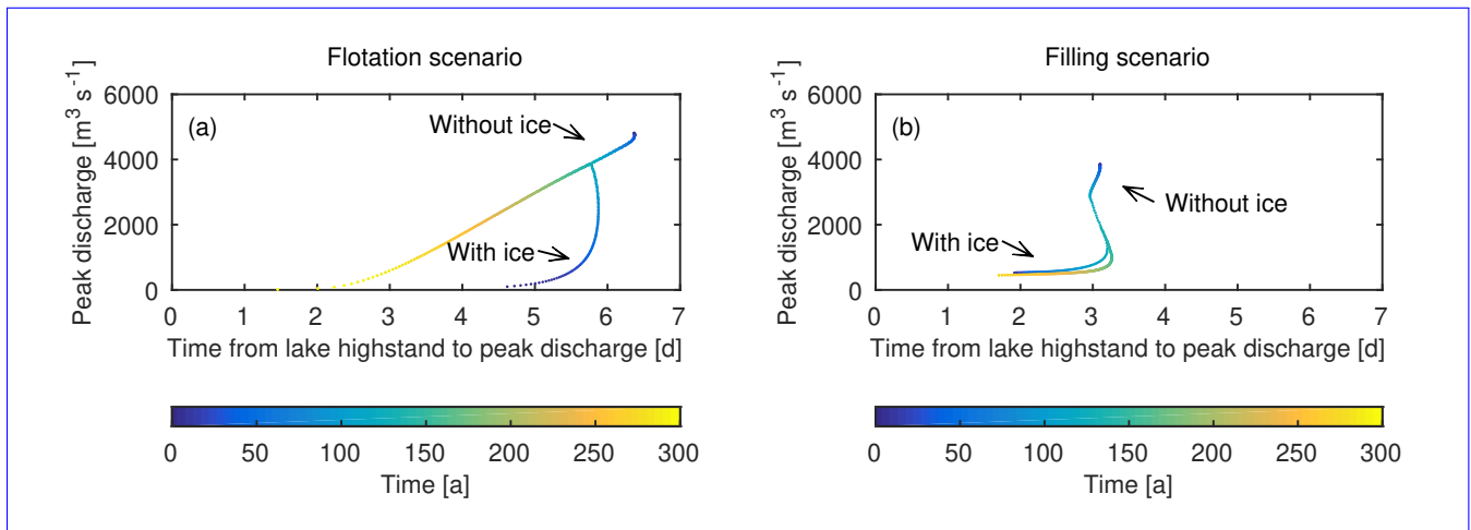
Figure 11. Comparison of peak discharge and time from lake highstand to peak discharge for the box-shaped basin under the (a) flotation and (b) filling scenarios.
