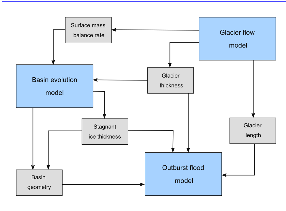
Figure 4. Information flow between the glacier flow, basin evolution, and outburst flood models.
