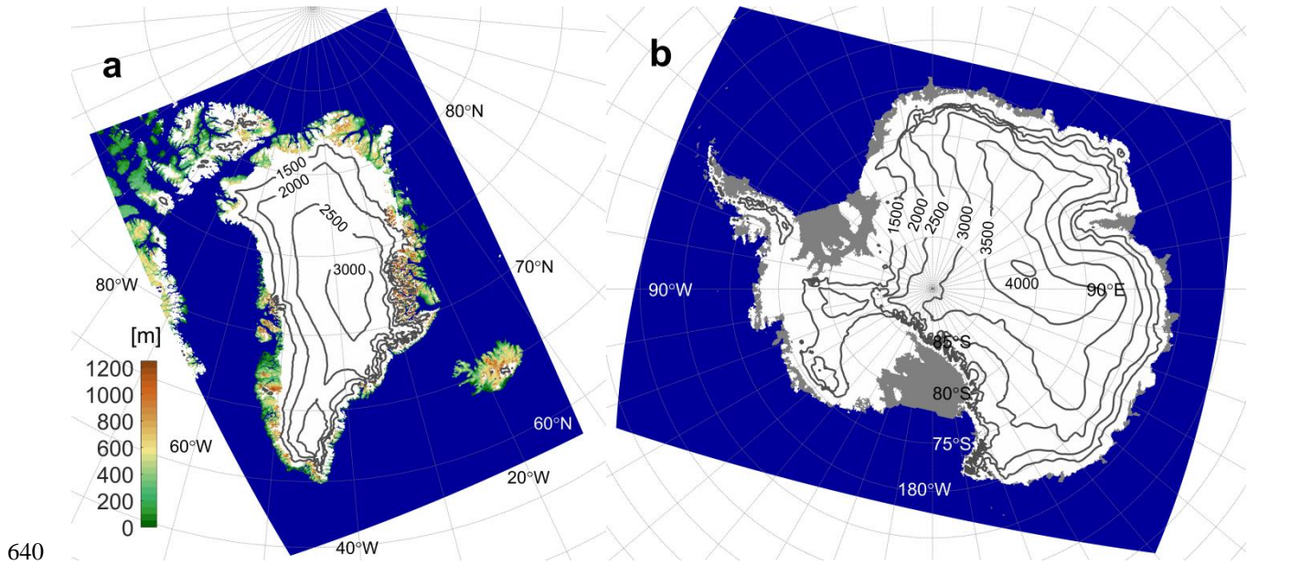
Figure 1. Topography for the two model domains. Sea points are given in blue, non-glacial land grid points are given in green and brown, Antarctic ice shelves are given in grey while glacial points are given in white with surface elevation contour lines added. The Greenland domain (a) has a model resolution of about 5.5 km (0.05°) while the Antarctica domain (b) has a model resolution of about 12.5 km (0.11°).
