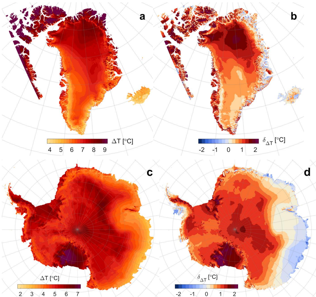
660 Figure 5. Change in 2 m temperature for Greenland for 2081–2100 relative to 1991–2010 for the EC-Earth v3 SSP5-8.5 scenario (a). Difference in the change in 2 m temperature for EC-Earth3 SSP5-8.5 relative to EC-Earth2 RCP8.5 (b). Change in 2 m temperature for Antarctica for 2071–2100 relative to 1971–2000 for the SSP5-8.5 scenario (c). Difference in the change in 2 m temperature for SSP5-8.5 relative to RCP8.5 (d). Note that the colorbar limits in panels a and c differ.
