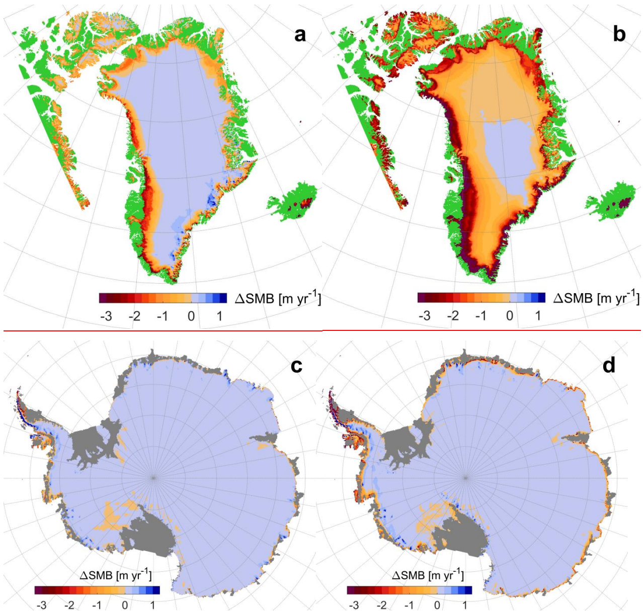
Figure 7. Changes in surface mass balance for Greenland for the period 2081–2100 relative to 1991 to 2010 for the EC-Earth2 driven run using RCP8.5 (a) and the EC-Earth3 driven run using SSP5-8.5 (b). Changes in surface mass balance for Antarctica for the period 2071–2100 relative to 1971 to 2000 for the EC-Earth2 driven run using RCP8.5 (c) and the EC-Earth3 driven run using SSP5-8.5 (d). Units are meter water equivalent per year. Green color represents non-glacial land grid points and grey color represents Antarctic ice shelves (cf. Figure 1).
