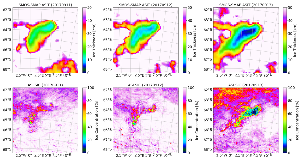
Figure 3. SMOS-SMAP ASIT (top row) and ASI SIC (bottom row) retrieval of the days leading up to the 2017 Weddell Sea Polynya: 11–13 September 2017.
