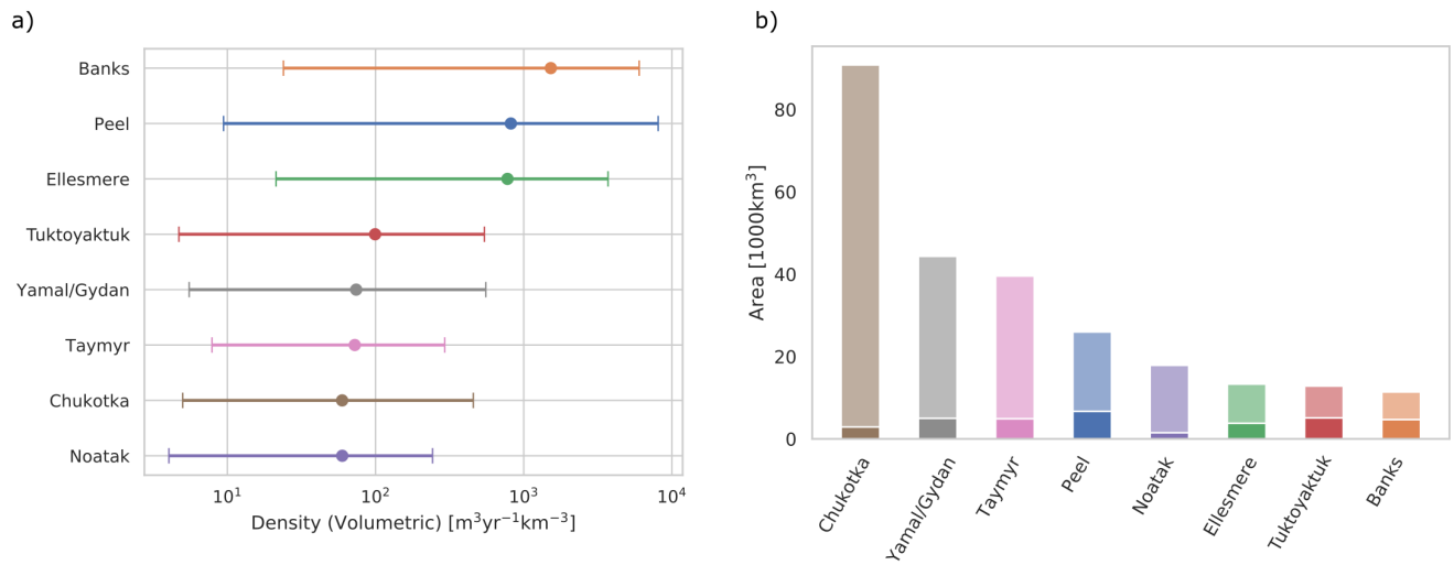
Figure 8. Volumetric change rate densities and density related to study site size for each study site. a) shows the computed RTS volumetric change rate densities using a 10 km by 10 km grid with the empty grid cells removed. The vertical bars indicate the range in the computed densities. (b) shows the study site size in transparent with the fraction of tiles with RTS present in solid (b).
