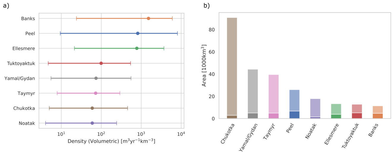
Figure 8. Volumetric change rate densities, a) , and density related to study site size, b) , for each study site. a) shows the computed RTS volumetric change rate densities using a 10 km by 10 km grid with the empty grid cells removed. The vertical bars indicate the range in the computed densities. (b) shows the study site size in-transparent with the fraction of tiles with RTS present in- represented by the solid (b) color.
