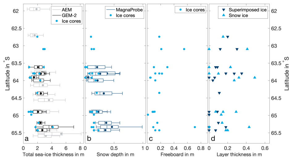
75 Figure 2: Ice and snow properties versus latitude: a. Total sea ice thickness (SIT, sea-ice thickness plus snow depth) derived from airborne EM sounding (AEM, grey), ground-based EM sounding (GEM-2, black) and ice cores (light blue); b. Snow depth measured with the MagnaProbe along GEM transects (dark blue) and measured at the ice-coring sites (light blue); c. Freeboard measured at the ice-coring sites (light blue); and d. Thicknesses of superimposed ice (dark blue triangles) and snow ice (light blue triangles) from all ice cores. Boxes are the first and third quartiles; whiskers the 10 th and 90 th percentile. Circles indicate means, horizontal lines in the box's medians. 80
