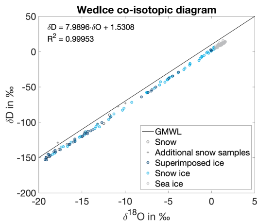
20 Figure C1: Oxygen isotope ( \delta^{18}\text{O} )-hydrogen isotope ( \delta\text{D} )-diagram for all WedIce samples differentiated by ice type. The Global Meteoric Water Line (GMWL; Craig (1961)) is given for comparison. During some ice stations additional snow samples have been taken next to the ice core sampling sites which were also analyzed for isotopes and are added here with crosses (+).
