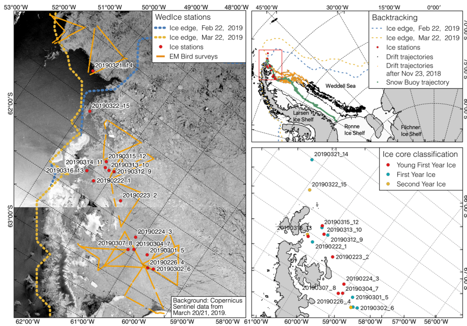
Figure 1: (left) Overview map of all sampled ice stations (red dots) and helicopter-borne electromagnetic induction sounding surveys (HEM, yellow lines). The ice station names are composed of the respective date and a consecutive station number. The dashed lines indicate the ice edge at the first day (February 22, 2019, blue) and last day (March 22, 2019, yellow) of our study. Background: Copernicus Sentinel-1 SAR images from March 20/21, 2019. (upper right) Back trajectories (black dots) of the sampled ice stations (red dots) during WedIce. The green line denotes the drift trajectory of the Snow Buoy 2018S59 deployed in February 2018 off the Ronne Shelf Ice. (lower right) Ice-age classification of all sampled ice cores: Second Year Ice (yellow), First Year Ice (blue), Young First Year Ice (red).
