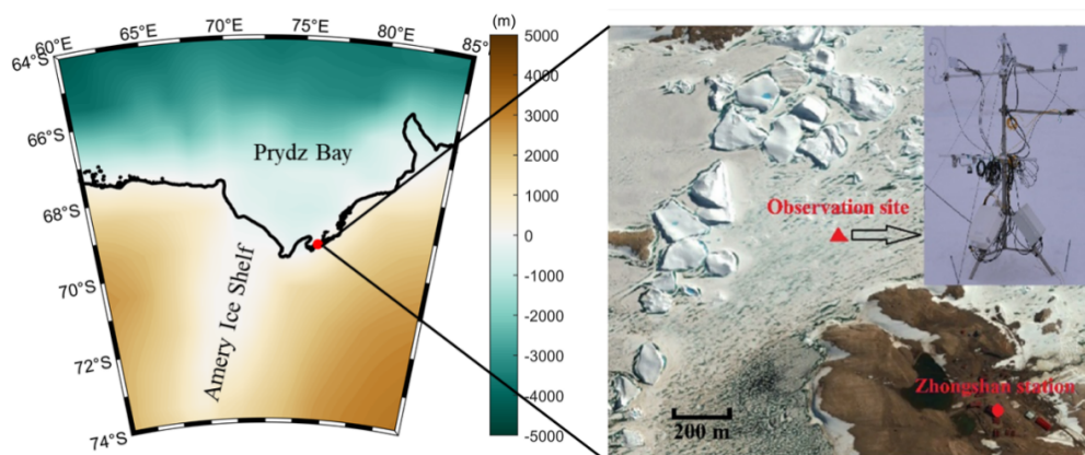
111 Figure 1 Location of landfast sea ice surface measurements near Zhongshan Station. The solid 112 triangle denotes the observation site, the solid circle marks Zhongshan Station. The color on the left
