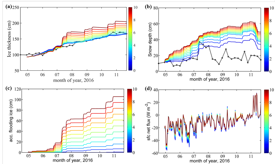
Figure 56 Time series of the simulated (a) sea ice thickness, (b) snow depth, (c) accumulated flooding ice, and (d) net surface heat flux in the n experiments of SEN 23 . The black solid point lines show the in situ observations (Obs). The 11 colored lines denote the 11 sensitivity experiments. When n = 0 , precipitation is from the in situ observation. When n = 10 , precipitation is from ERA5.
