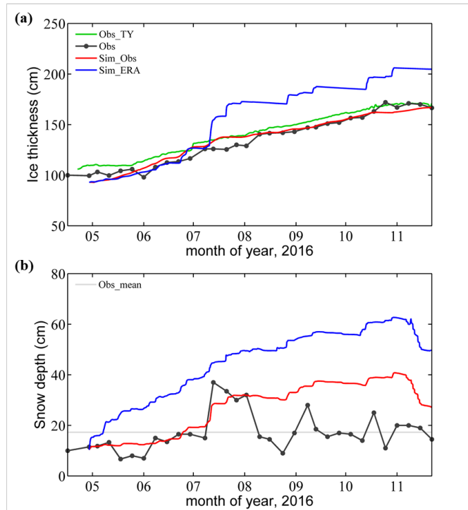
265 Figure 3 Time series of (a) sea ice thickness and (b) snow depth during the freezing season. Black 266 solid lines with black points show the observations from the drill hole (Obs). Green solid lines show 267 the ice thickness derived from the TY buoy (Obs_TY). Red solid lines show the simulation results 268 under in situ atmospheric forcing (Sim_Obs), and blue solid lines are simulation results under ERA5 269 forcing (Sim_ERA). In (b), the gray solid line shows the seasonal mean snow depth observation 270 (Obs_mean).
