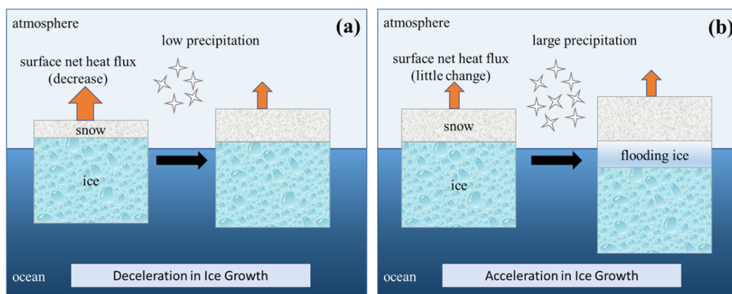
Figure 78 Schematic diagram for (a) low precipitation and (b) large precipitation events illustrating the precipitation effect on sea ice growth. The orange arrows represent surface net heat flux, and different colored boxes indicate the layer of snow, flooding ice, and sea ice.
