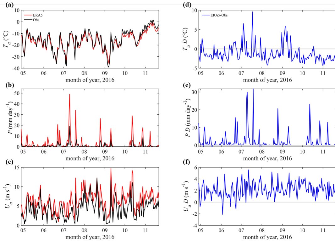
Figure 2 Time series of daily (a) surface air temperature, (b) precipitation rate, and (c) wind speed (10 m above the surface). The ERA5 reanalysis data are indicated as red lines. Observations are marked by black lines. (d-f) show the difference (marked by 'D') between ERA5 and the observation (ERA5-observation). The differences are marked by blue lines. The gray lines denote the zero line.
