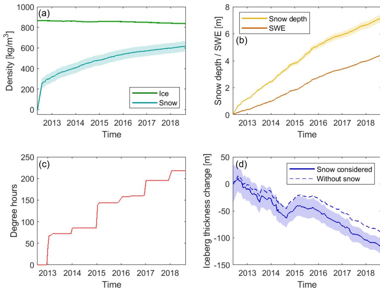
405 Figure 8: Evolution of the B30 iceberg properties: a) Ice density and snow density, b) Snow water equivalent (SWE) and snow depth accumulation on the B30 iceberg, c) Degree hours that the B30 iceberg experienced, and d) Thickness change of the B30 iceberg with snow accumulation taken into consideration or without. Uncertainties are plotted as shaded areas.
