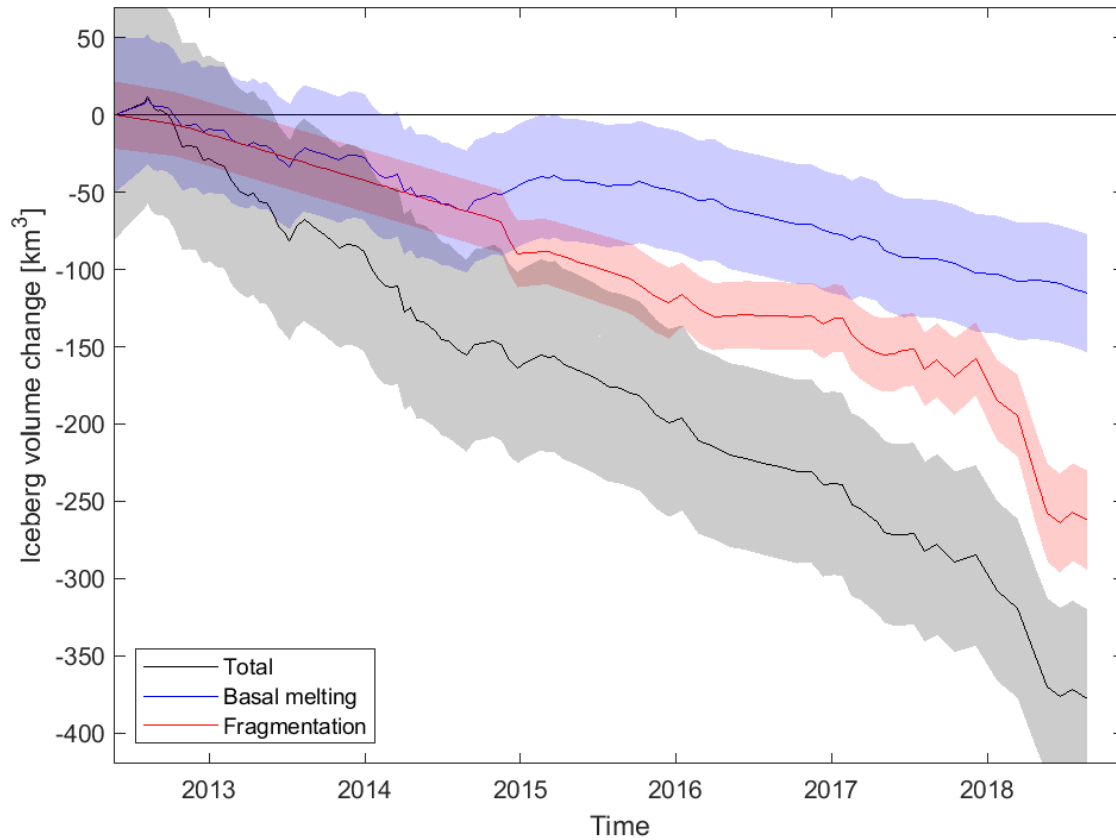
470 Figure 9: Volume change of the B30 iceberg divided into loss due to basal melting (thickness change, blue) and due to fragmentation (area change, red), as well as total volume loss (black).
