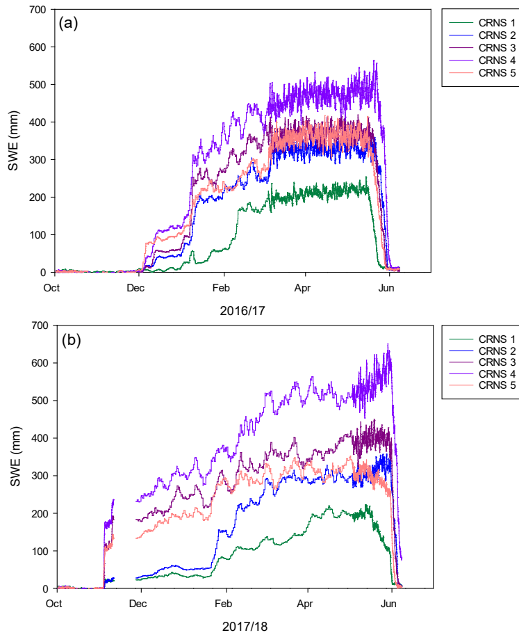
Figure 8. Change in SWE at TVC from each individual-CRNS throughout the (a) 2016/17, and (b) 2017/18 winter season. The locations of CRNS 1 to 5 are shown in Fig. 3. CRNS 1 and 5 are located at the edges of the shrub patch, and CRNS 2 to 4 are located in the centre of the patch. The sudden noisiness starting on March 4, 2017 in the 2016/17 season and May 3, 2018 in the 2017/18 season is due to the change in frequency of the sampling rate. This change in frequency occurred when we switched the CRNS system from winter power conservation mode, which had four, one-hour interval recordings per day, to standard power mode which had 24, one-hour interval recordings per day.
