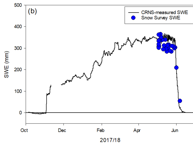
Figure 7. Continuous measurement of a snowdrift at TVC in the (a) 2016/17 and (b) 2017/18 winter season. CRNS-SWE-measured SWE was averaged from the 5 CRNS and values were calculated using Eq. (4).
