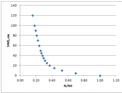
565 Figure A1. Grounded in-situ CRNS measurement approximation relative to SWE and N/N_0 .
