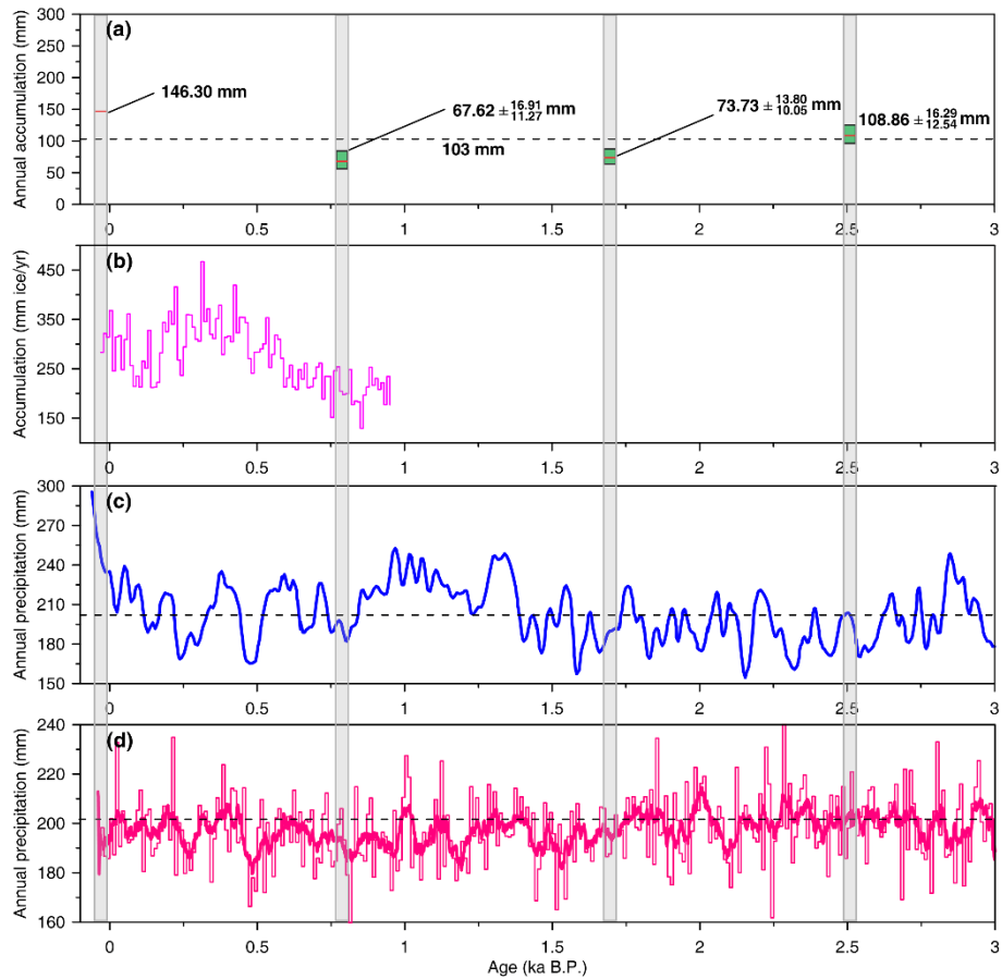
Figure 4. Our reconstructed annual accumulation for each of the four sections sampled (a) and its comparison with (b) snow accumulation reconstruction based on the Guliya ice core (Thompson et al., 550 2006), (c) precipitation reconstruction with 50-year smoothing in the northeastern TP (Yang et al., 2014), and (d) the TraCE-21 ka model results for the region (34-36°N, 80-82°E) (Collins et al., 2006). The dotted lines in (a) and (d) represent the average annual accumulation over the Holocene. The dotted line in (c) represent average annual accumulation over the past 3.0 ka. The thin and thick red lines in (d) represent 10-year and 50-year moving average respectively.
