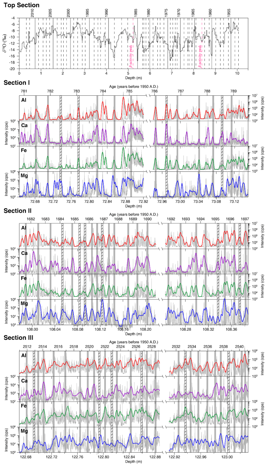
Figure 2. Annual layer counting for the Top Section, Section I, II, and III (top to bottom). The annual layers of the Top Section are identified based on the seasonality of \delta^{18}\text{O} and two \beta -activity peaks (An
