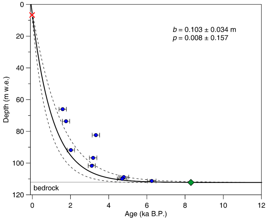
515 Figure 3. The depth-age relationship of the Chongce Core 2 based on the two-parameter model. The dashed lines represent the 1\sigma confidence interval of the two-parameter model fit (solid line). The red cross stands for the \beta activity peak in 1963 A.D., the blue dots the calibrated ^{14}\text{C} ages with 1\sigma error bar, green diamond for bedrock age estimate from the Chongce Core 4 (Hou et al., 2018; Zhang et al., 2018).
