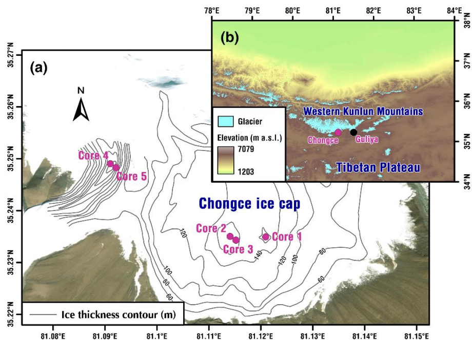
Figure 1. (a) Satellite image of the Chongce ice cap with location of the ice-core drilling sites (deep 500 rose dots). Ice thickness contours were superimposed on the image of the glacier. (b) Topographic map of the northwestern TP. The satellite imagery map is available at: https://www.mapsofworld.com/satellite-map/world.html . The topographic data were extracted using the Shuttle Radar Topography Mission (SRTM) 90 m DEM digital elevation database, available at:
