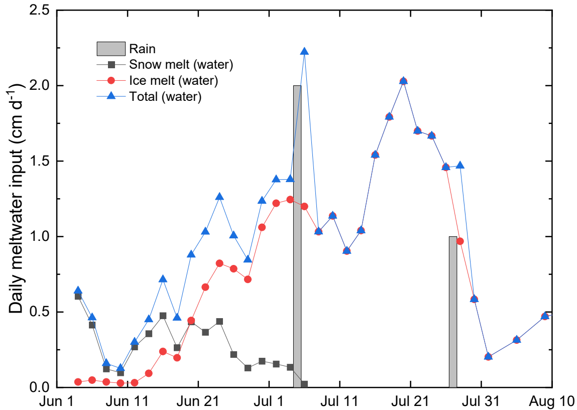
Figure 2. Time series of freshwater meltwater input from snow melt, surface ice melt, and rain.
