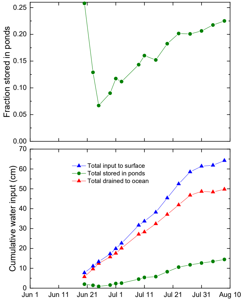
145 Figure 4. Time series of the fraction of surface water input stored in ponds (top), and cumulative surface water input, storage in ponds ( P_v ), and drained to ocean.
