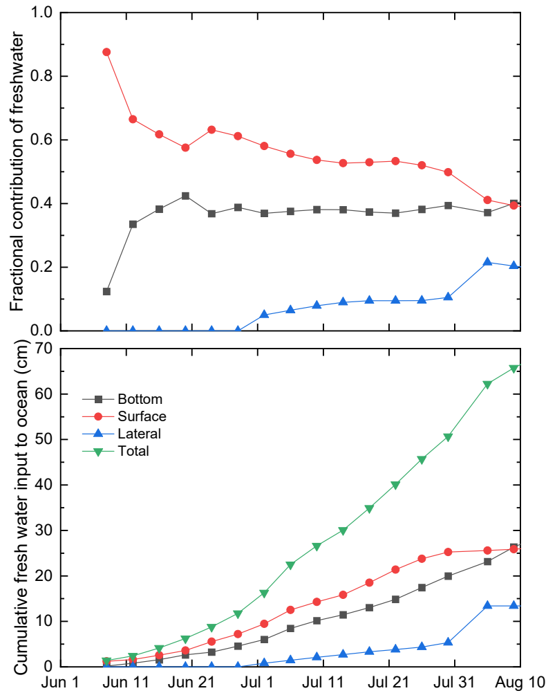
Figure 8. Upper ocean freshwater meltwater budget. Time series of fresh input to the ocean with contributions from lateral melting, bottom melting, and surface melting. The total input is also plotted. The melt contributions have been adjusted by the ice concentration.
