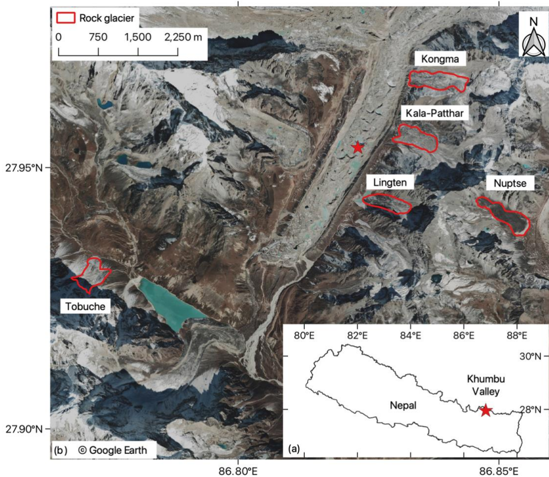
80 Figure 1: (a) Location of the study site; (b) Google Earth images (taken in 2019) showing the spatial distribution of the active rock glaciers (RG) outlined in red. The RGs are delineated by Jones et al. (2018).
