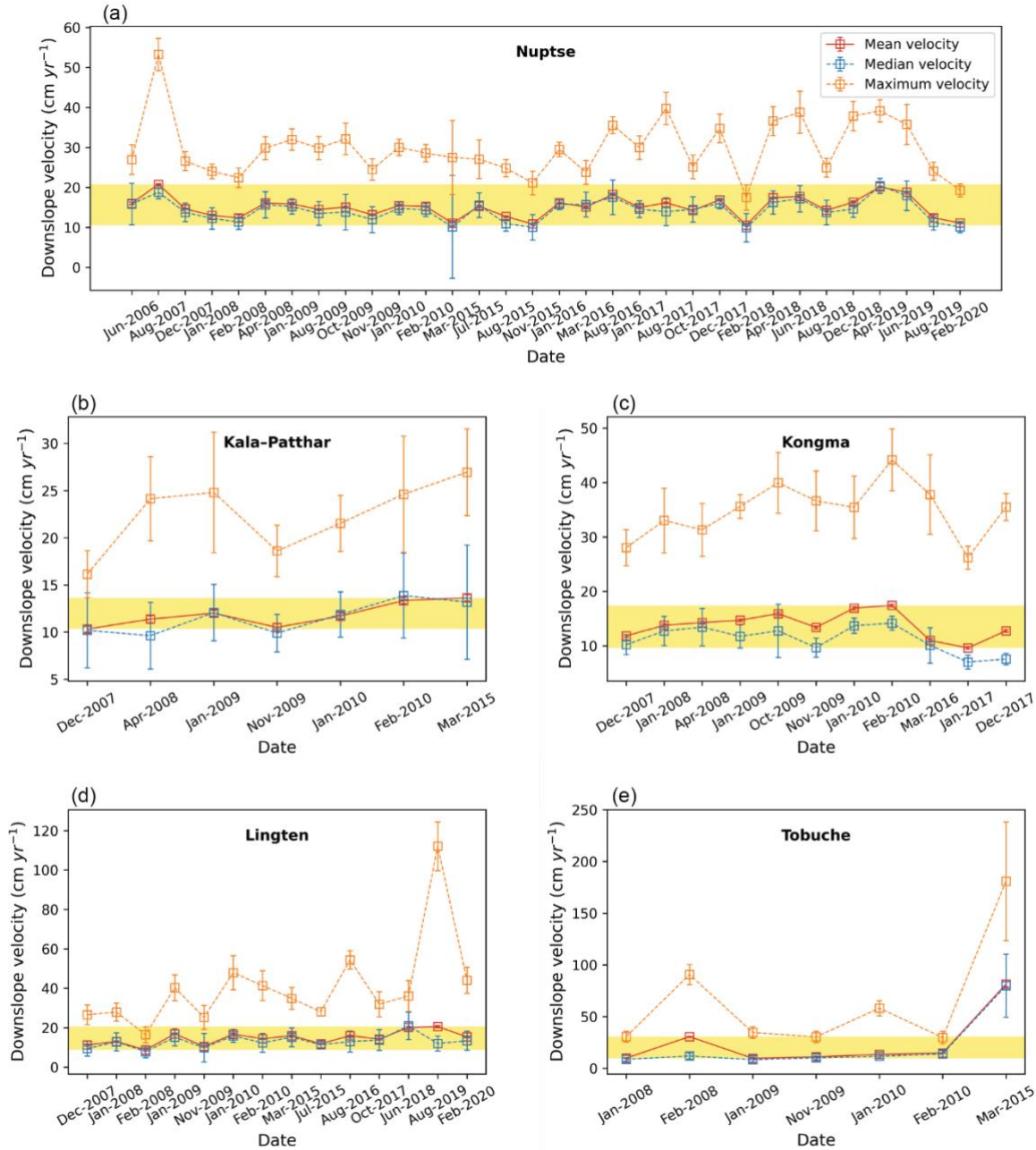
Figure 7: Time series of the InSAR-derived downslope velocities of the rock glaciers. The spatial mean velocities and uncertainties during each period are shown (red squares and error bars) as well as the median (blue) and maximum (orange) velocities. The yellow bands highlight the range of the mean velocities which were used as model constraints for estimating ice fractions.
