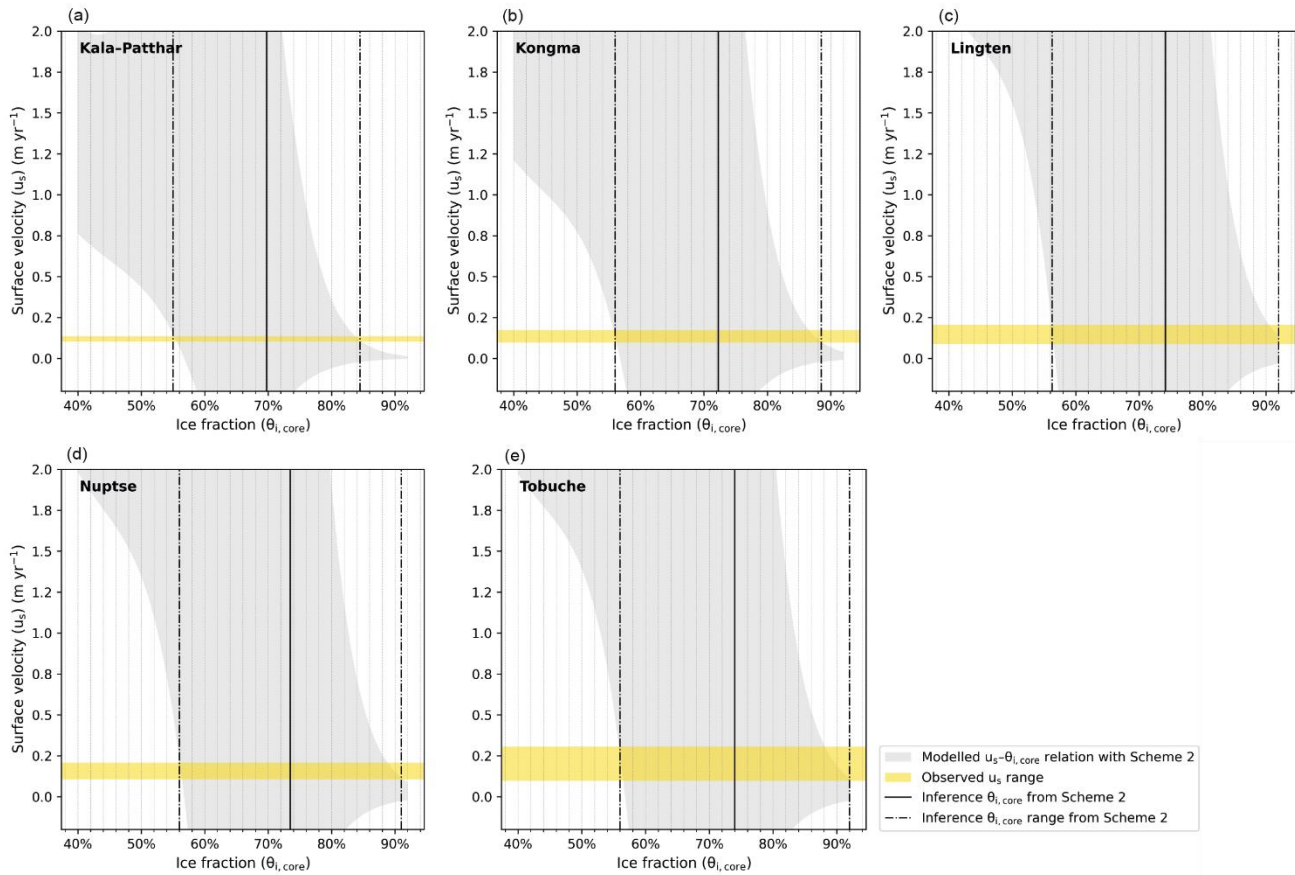
385 Figure 9: Modelled relationships between the ice fraction ( \theta_{i,core} ) and the surface velocity ( u_s ) of 95% confidence intervals for the five RGs in Khumbu Valley with model parameterisation Scheme 2 (grey shaded areas). The ranges of the InSAR-derived velocities (yellow bands) are used as the velocity constraints for inferring ice contents from the modelled relationships. The upper and lower boundaries of the estimated ice contents are within the range outlined by the dash-dotted black lines and the solid black lines show the mean values representing the inference ice contents.
