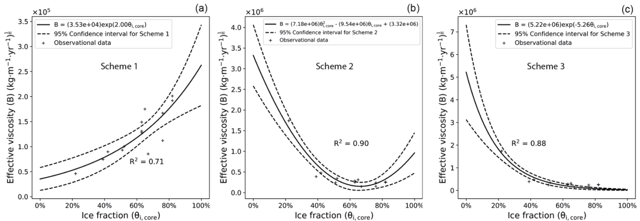
310 Figure 4: (a)–(c) Relationships between the ice fraction ( \theta_{i,core} ) and the effective viscosity ( B ) estimated from the three regression equations and parameterisation schemes (Eq. 15, 16, and 17, respectively). The observational data are derived from the GPR and DGPS measurements by in-Monnier and Kinnard (2015b & 2016) .
