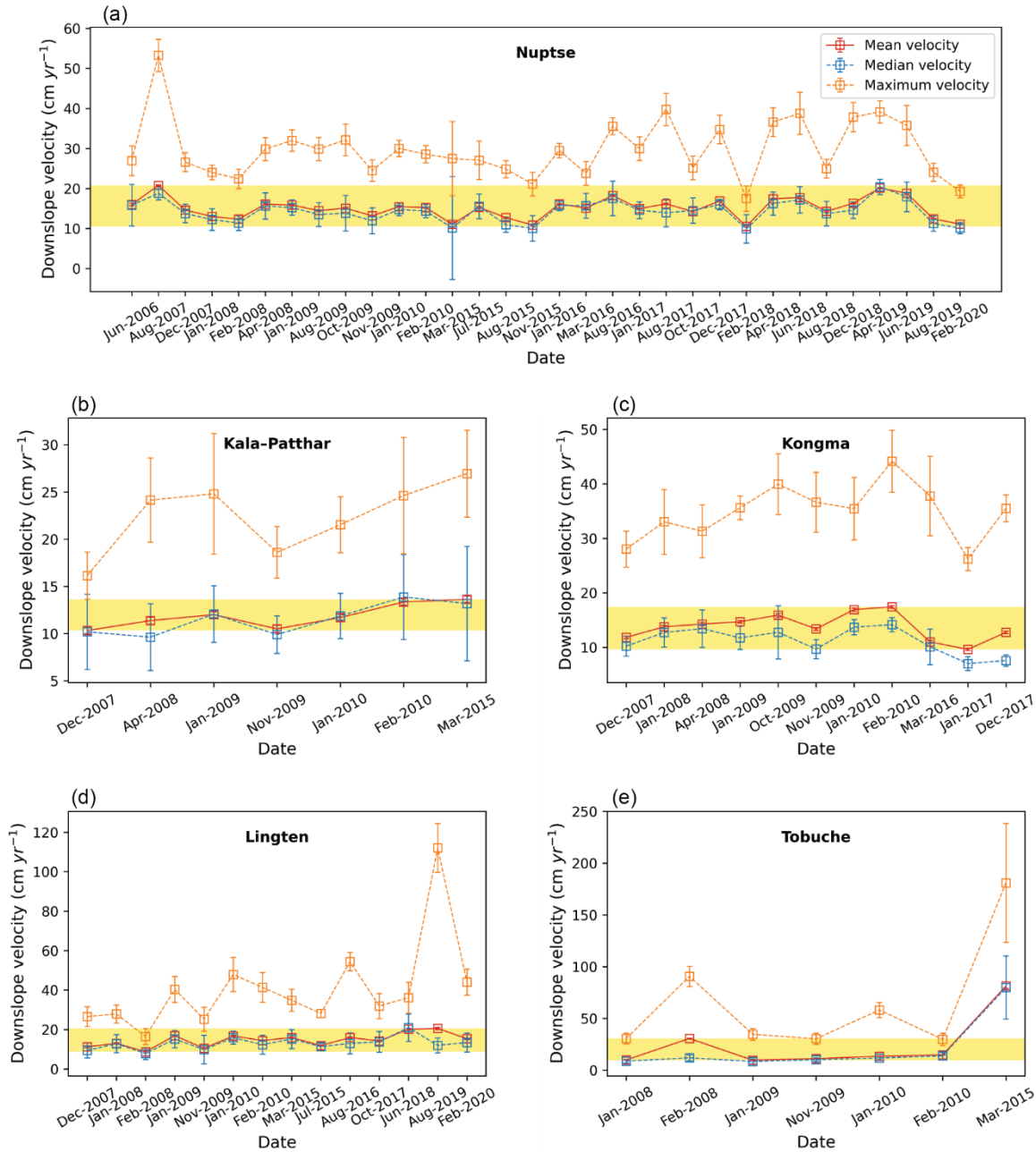
365 Figure 7: Time series of the InSAR-derived downslope velocities of the rock glaciers landforms. The spatial mean velocities and uncertainties during each period are shown (red squares and error bars) as well as the median (blue) and maximum (orange)
