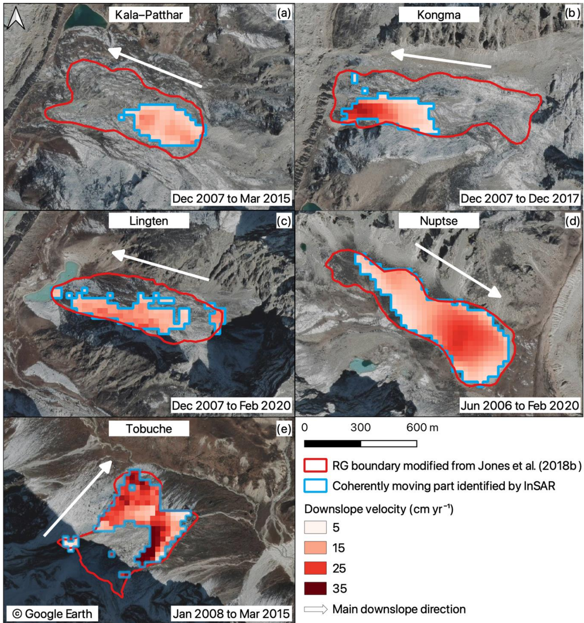
370 Figure 8: Velocity field maps show the average velocities of the coherently moving parts of the five rock glaciers (blue outlines) in the study area. The boundaries of the rock glaciers landforms delineated in Jones et al. (2018b) are plotted in red. The transparent areas between the red and blue boundaries are due to low coherence or low velocity during the observational periods.
