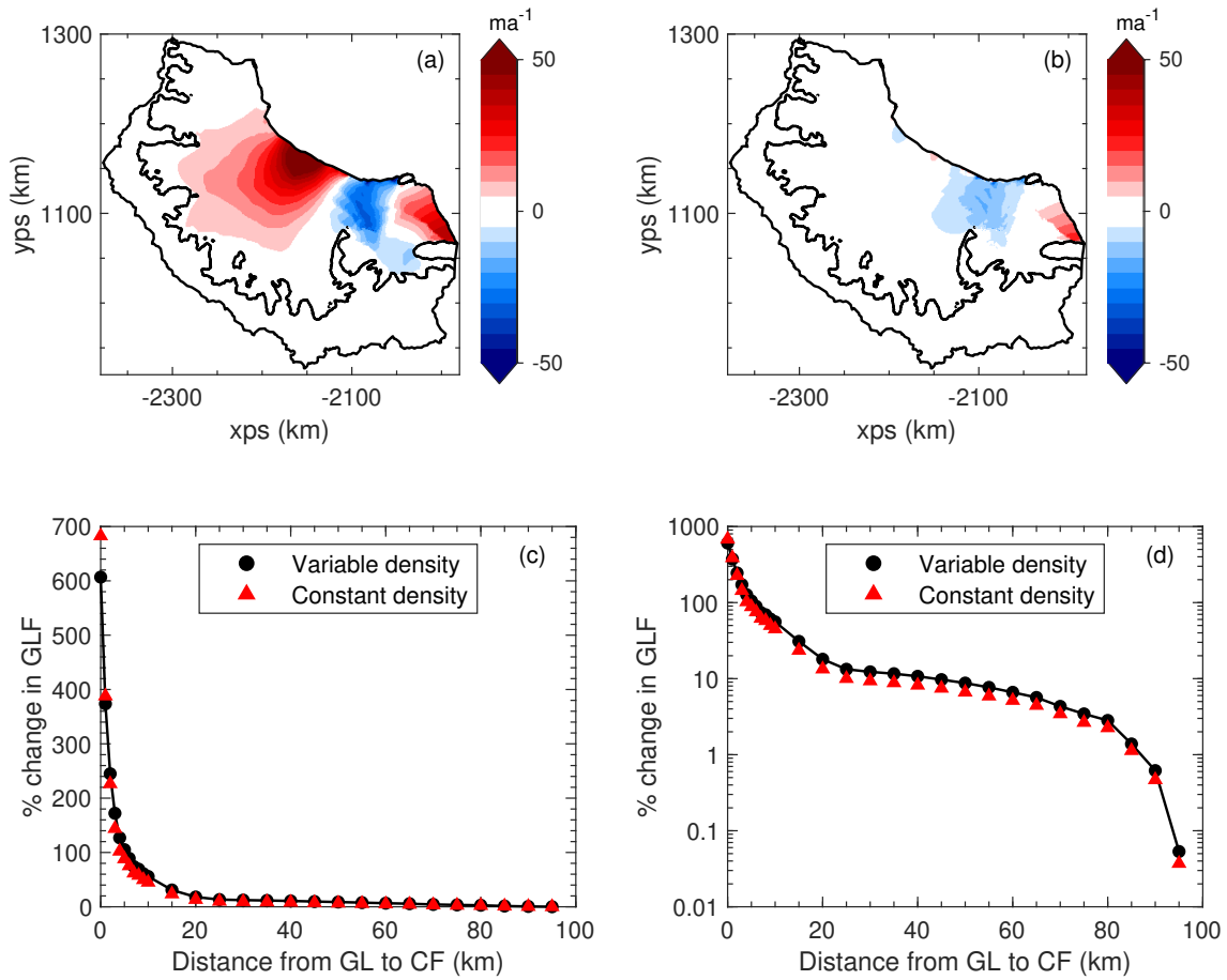
Figure D2. The results of calving experiments using a constant ice density of 917 \text{ kgm}^{-3} . (a) shows the modelled response to the calving of the A68 iceberg using the constant density setup, whilst (b) shows the difference between the constant ice density response and the variable ice density response to the A68 calving. (c) and (d) show the instantaneous grounding line flux response to the idealised calving experiments for the variable ice density setup (black, the same data as in Fig. 4a and b) and the constant ice density setup (red).
