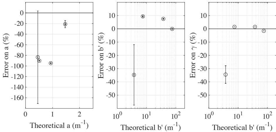
Figure 7: Validation of IOPs measurements using reference media. The reference media were 4 solutions of polystyrene microspheres in distilled water. Microspheres concentrations were chosen for the theoretical a and b' ranges to cover sea ice typical values. Detecting fibrs 1 and 7 were taken out for optimized results.
