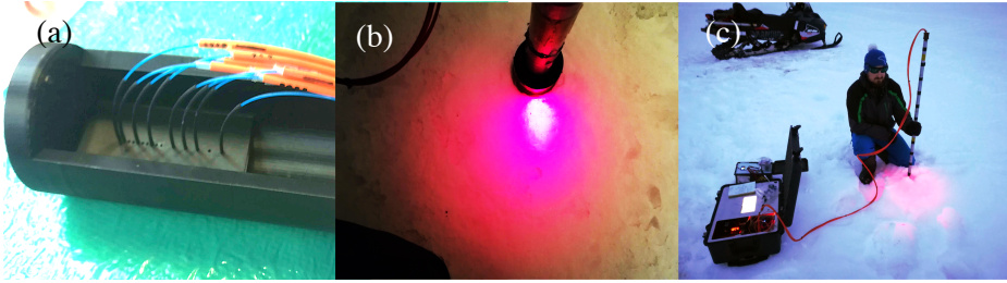
Figure 2: (a) Probe head interior. Source and detecting fibres were held in place with heat shrink tubes and glue. Fibres bend radii are meant to respect the minimum long-term limit of 40 mm. (b) Probe head inserted in a 2" auger hole drilled in sea ice. (c) Probe operated on sea ice close to Qikiqtarjuaq Island on the coast of Baffin Bay.
