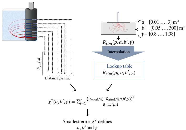
395 Figure 4: Illustration of the inversion algorithm used to retrieve inherent optical properties of sea ice.
