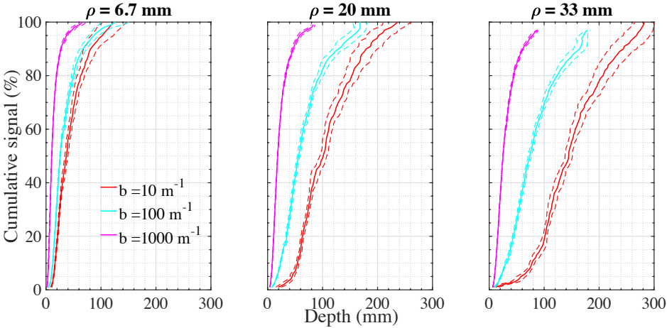
490 Figure 6: Estimation of the depth of signal origin for our probe geometry simulated by Monte Carlo. The cumulative signal R(z, r)/R_{zmax}(r) vs absorptive plate depth z at different lateral distances \rho was evaluated for three b typical of sea ice, \alpha=0.1 \text{ m}^{-1} and g=0.94 . We ran 40 simulations of 10^6 photons for every z when b=10 \text{ m}^{-1} and 100 \text{ m}^{-1} and 10 simulations of 10^6 photons for every z when b=1000 \text{ m}^{-1} . The standard deviation on simulations was used to evaluate uncertainties.
