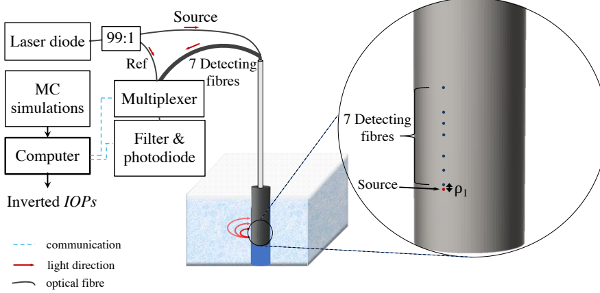
Figure 1: Experimental setup schematic. The two-inch probe was designed to fit an auger hole drilled through the ice and to measure sideward on the edge of the hole. A laser diode emitted at \lambda=633 \pm 2 nm with full-width half-maximum of 1.4 nm and optical power of 300 mW. A 99:1 fibre optic coupler divided optical power between a leg used to guide light up to the probe head where injection into sea ice occurred and the reference leg. Detecting optical fibres at distances \rho_{1-7} collected backscattered laser light (curved red arrows). An optical multiplexer selected the fibre to be read by a photodiode. A reflective bandpass filter centred at \lambda=633 nm with full-width half-maximum of 5 nm was placed before the photodiode to reject sunlight. A single-board computer with an easy-to-operate touch screen controlled the multiplexer, obtained \Phi readings from the photodiode and did a field inversion on b' .
