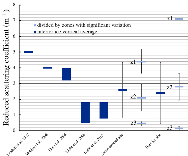
620 Figure 10: Comparison of the vertical averages of b' measured in situ at both sampling sites to vertical averages of b' published over the past for polar interior sea ice using various methods. For our measurements, the average reduced scattering coefficients b' is also divided by zones. Zones are separated at depths where we observed significant changes in scattering properties. The error bars represent the standard deviation for the given depth interval.
