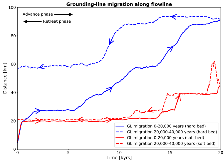
Figure 11. Grounding line migration along a flowline (A-A' in Fig. 1) for the soft and hard bed simulations for the advanced (solid lines) and retreat phase (dashed lines).
