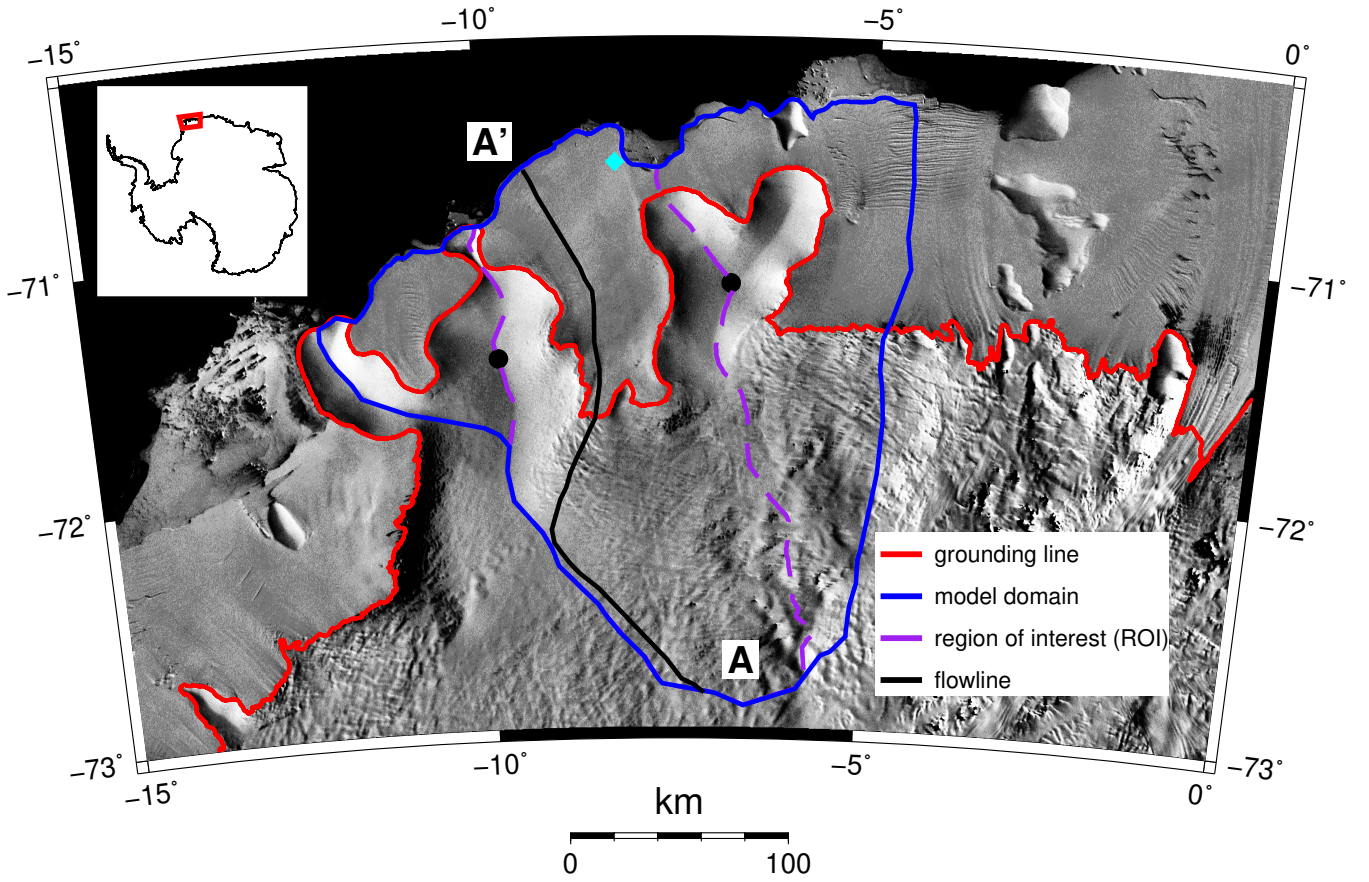
Figure 1. Overview of the Ekström Ice Shelf catchment with present day grounding line (Bindshadler et al., 2011) and model domain. Cyan square shows location of Neumayer Station III. Filled black circles indicate location of ice rises. Flowline (A-A') is shown in Fig. 10. Background is the MODIS Mosaic of Antarctica (Scambos et al., 2007).
