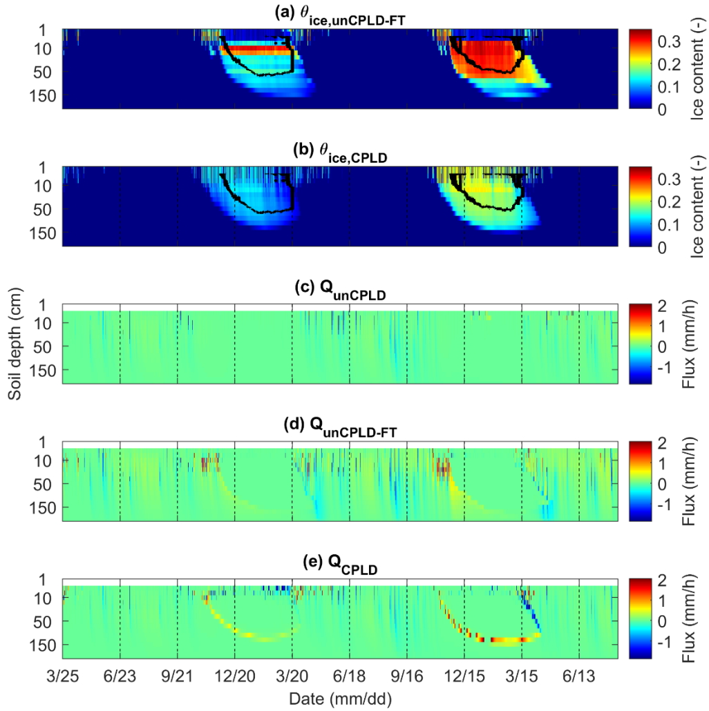
880 Figure 8. Soil ice content from (a) unCPLD-FT and (b) CPLD model simulations with freezing front propagation derived from the measured soil temperature; and vertical water flux (positive value indicates upward water flow) from (c) unCPLD, (d) unCPLD-FT and (e) CPLD model simulations. Note that soil ice content is not represented in the unCPLD model and the fluxes of top 2 cm soil layers were not reported to highlight fluxes of the lower layers.
