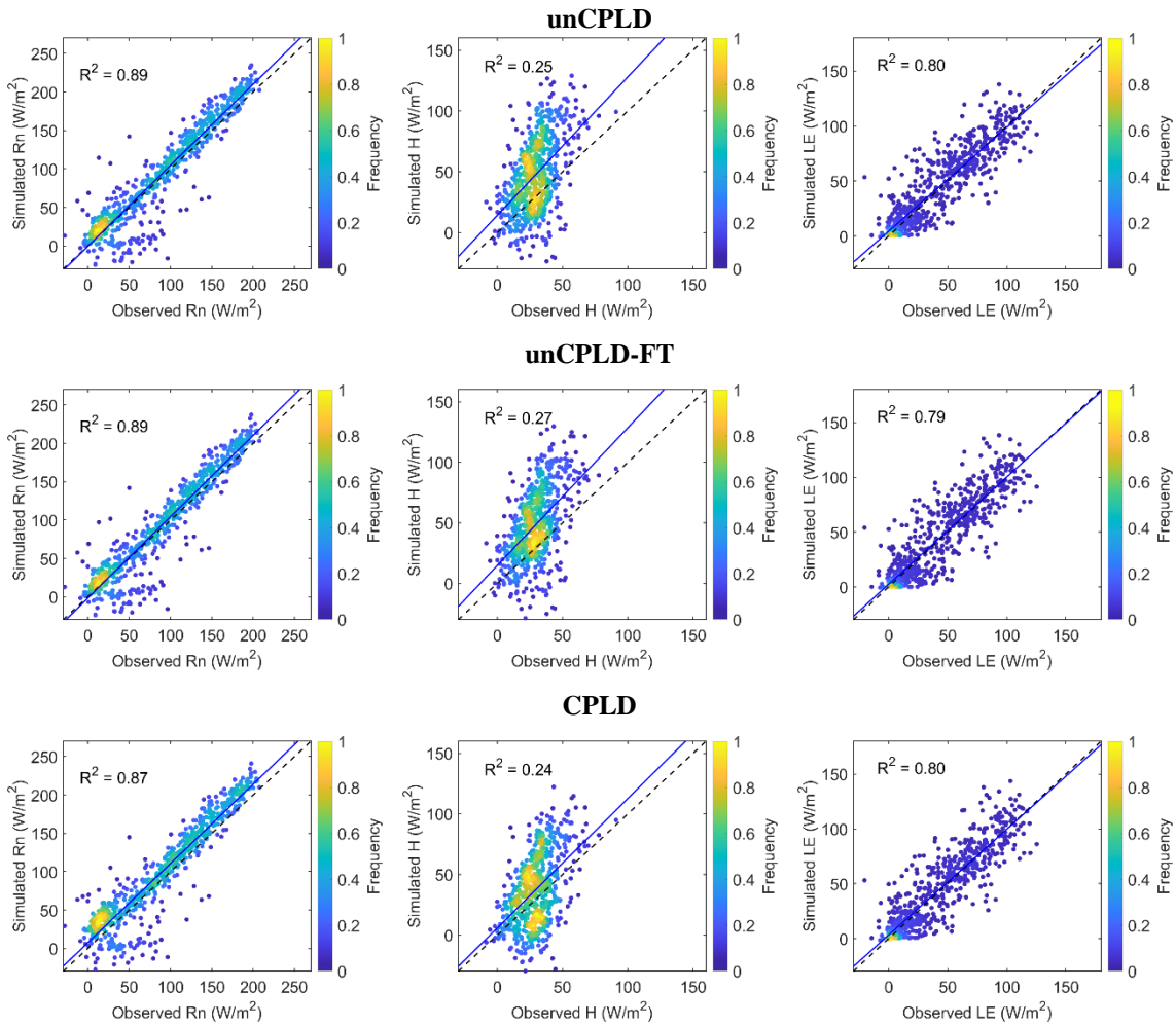
855 Figure 5. Scatter plots of observed and model simulated daily average surface fluxes (net radiation: Rn, latent heat: LE and sensible heat flux: H) using the original (uncoupled) T&C (unCPLD), T&C with consideration of FT process (unCPLD-FT) and coupled T&C and STEMMUS (CPLD) model, with the color indicating the frequency of surface flux values.
