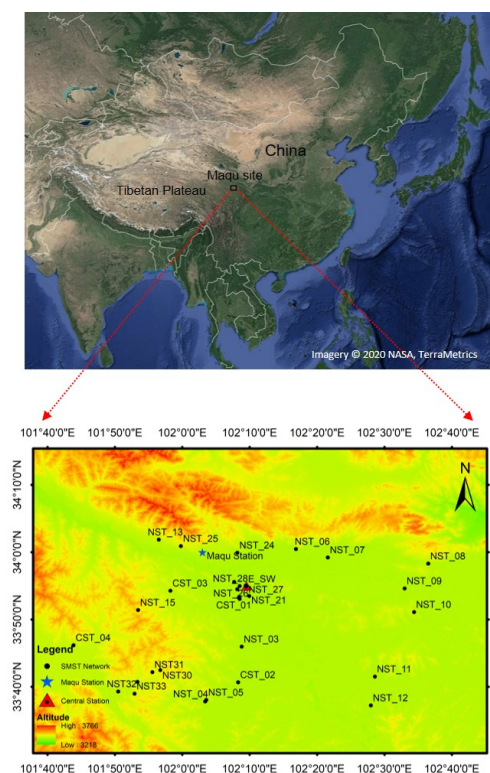
Fig. 1. Figure 1. Geographical location of Maqu soil moisture/temperature (SMST) monitoring network and the Centre station.
