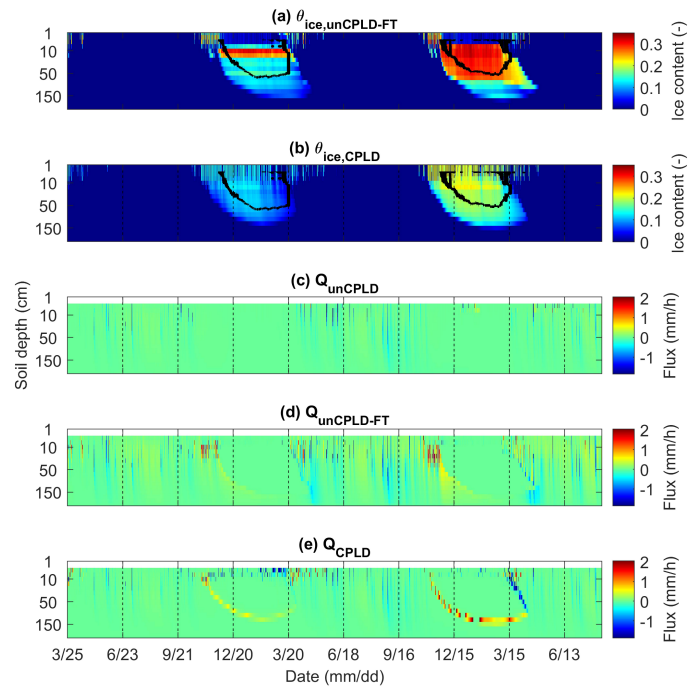
Fig. 5. Figure 8. Soil ice content from (a) unCPLD-FT and (b) CPLD model simulations with freezing front propagation; and vertical water flux from (c) unCPLD, (d) unCPLD-FT and (e) CPLD model simulations.
