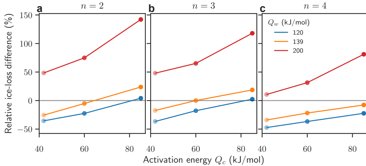
Figure 9. Effect of the flow exponent and activation energies on flow-driven ice loss after 100 years under 2°C of warming: Relative difference in flow-driven ice discharge for n = 2 (a), n = 3 (b) and n = 4 (c) for different combinations of the flow exponent n and activation energies Q_c and Q_w . The reference is always a simulation performed with standard parameters n = 3 , Q_c = 60 kJ/mol and Q_w = 139 kJ/mol.
