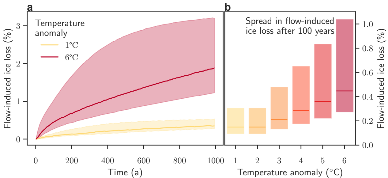
Figure 8. Effect of temperature forcing and activation energy on flow-driven ice (a) Time evolution of ice loss under warming of 1^{\circ}\text{C} and 6^{\circ}\text{C} . For warming of \Delta T = 1^{\circ}\text{C} the conceptual ice sheet loses 0.35% of ice after 1000 yr for standard parameters (solid, yellow line). Variations in the activation energies Q lead to variations in ice loss on the same order of magnitude (shaded area). For a warming of \Delta T = 6^{\circ}\text{C} the conceptual ice sheet loses 1.89% of ice after 1000 yr for standard parameters (solid, red line). The variations in ice loss due to different parameters for the activation energy Q (shaded area) are strongly asymmetrical and, in particular during the first 300 years, high compared to the total amount of ice loss. (b) Uncertainty in flow induced ice loss after 100 years of simulation time over all combinations of Q_w , Q_c and temperature anomalies \Delta T . The flow exponent n = 3 is kept fixed for all simulations.
