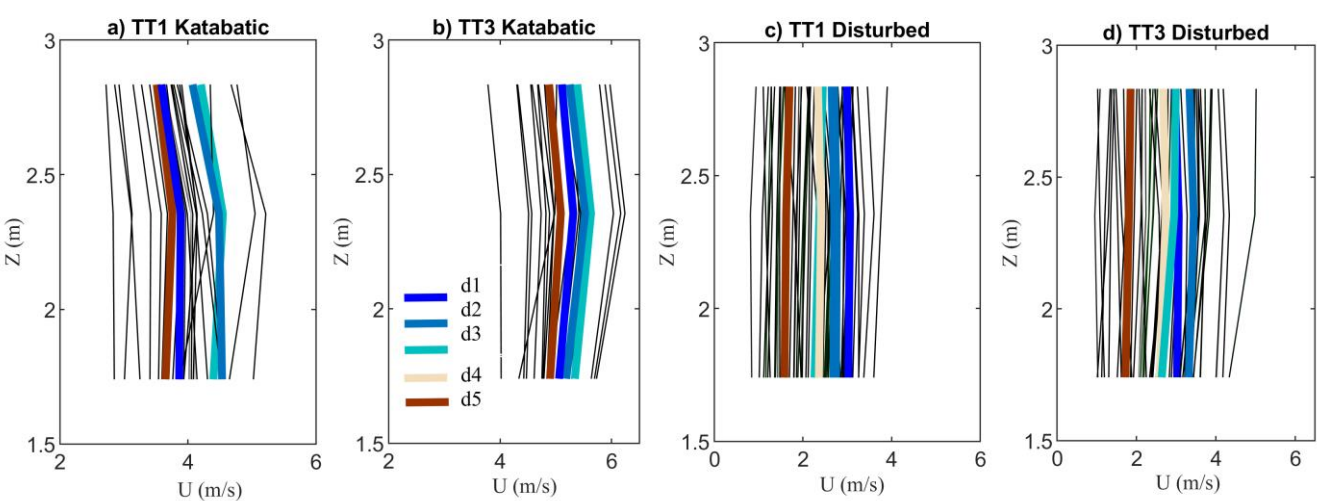
220 Figure 4: Profiles of 30 minutes and daily (bold) averages of wind speed ( U ) measured during pure katabatic flow and during disturbed flow conditions at transect stations TT1 and TT3. Note that only 30-minute averaged data was considered as pure katabatic if data showed katabatic flow during the entire 30 minutes periods. Colours of bold lines indicate different measurement days.
