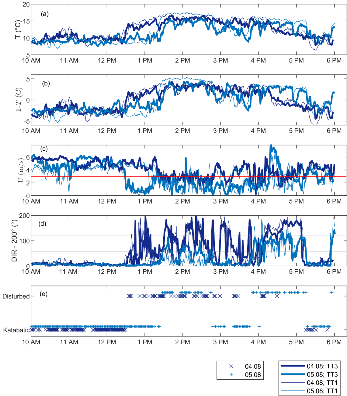
210 Figure 3: 1-minute averages of a) air temperature, b) air temperature anomalies, c) wind velocity, d) wind direction deviation from the prevailing katabatic wind direction ( 200^{\circ} ) for stations TT1 and TT3 and e) of classification of katabatic and disturbed flow based on station TT3. The solid line indicates the lower limit of 3 m/s for katabatic flow classification in c) and the lower
