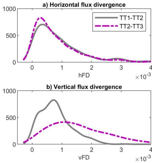
Figure 13: Kernel distribution of streamwise horizontal (hFD) and vertical (vDF) heat flux divergence shown only for disturbed conditions and the 60° wind sector (260°-320°).
