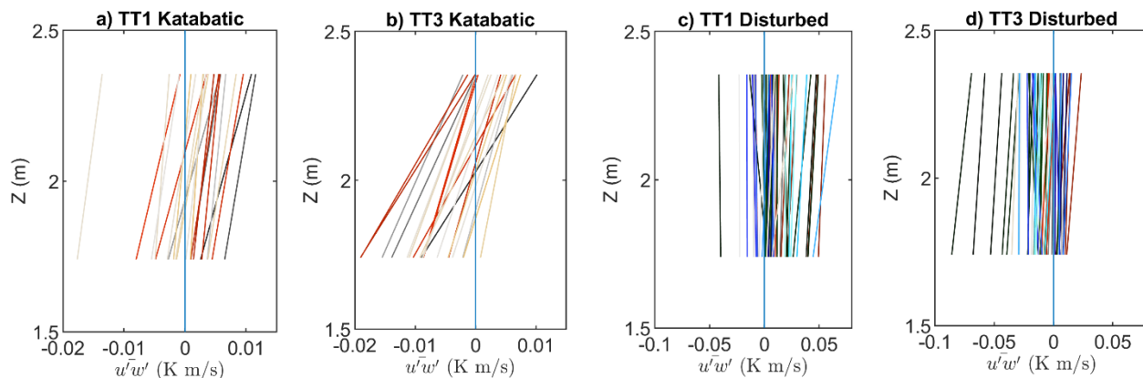
280 Figure 6: Profiles of 30 minutes averages of wind speed ( U ) streamwise momentum flux ( \overline{u'w'} ) measured during pure katabatic flow and during disturbed flow conditions at transect stations TT1 and TT3. Note that only 30-minute averaged data was considered as pure katabatic if data showed katabatic flow during the entire 30 minutes periods. Colours indicate different measurement days (grey=day1, red=day 2; green=day3; blue=day 4; brown=day5).
