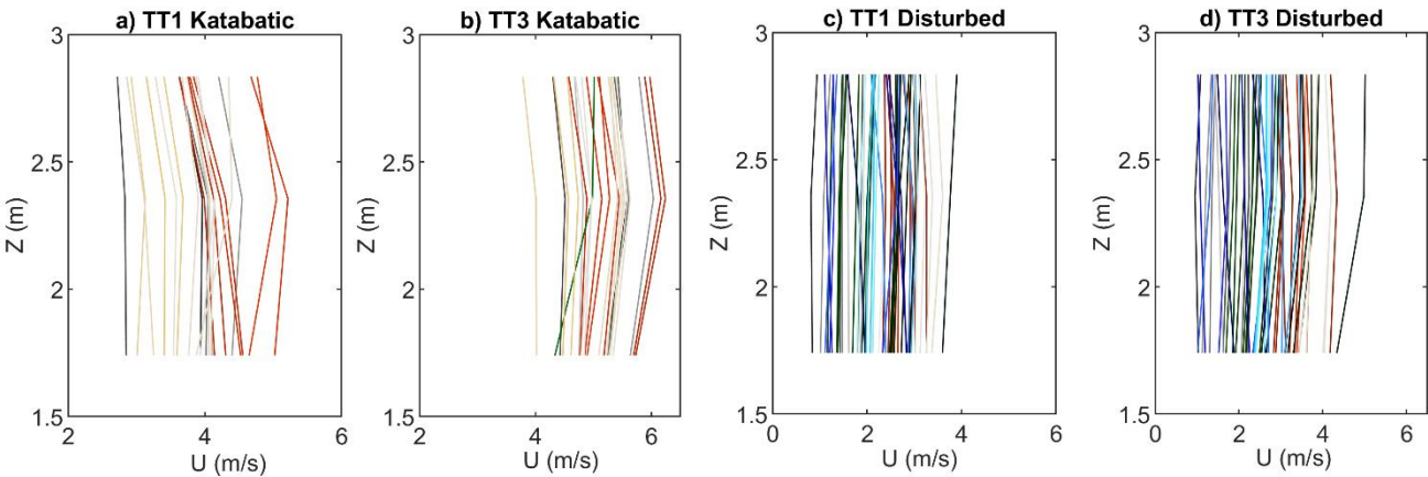
225 Figure 4: 30-minutes averaged profiles of wind speed for katabatic (a, b) and disturbed (c, d) conditions during five days in August 2018 obtained from the mobile wind tower and station TT3. Note that data was only considered as pure katabatic with mean wind speeds larger than 3 m/s. Due to long averaging tim of 30 minutes the classification is different to the 1-minute classification. Colours indicate different measurement days (grey=day1, red=day 2; green=day3; blue=day 4; brown=day5).
