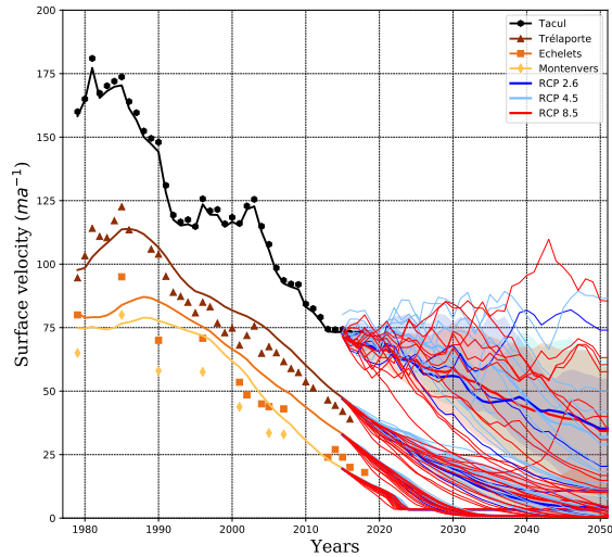
Figure 5. Surface velocity and surface elevation for all prognostic simulations. Hindcasts at the 4 profiles are shown by black (Tacul), brown (Trélaporte), orange (Echelets) and yellow (Montenvers) curves and the symbols are the corresponding observations. Forecasts are shown in dark blue (RCP 2.6), blue (RCP 4.5) and red (RCP 8.5), with the average forecasts represented by thick curves with 1\sigma uncertainty bands (colored area). Dashed lines indicate the bedrock elevation for the 4 profiles.
