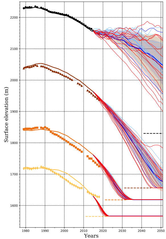
Figure 5. Surface velocity and surface elevation for all prognostic simulations. Hindcasts at the 4 profiles are shown by black (Tacul), brown (Trélaporte), orange (Echelets) and yellow (Montenvers) curves and the symbols are the corresponding observations. Forecasts are shown in dark blue (RCP 2.6), blue (RCP 4.5) and red (RCP 8.5), with the average forecasts represented by thick curves with 1\sigma uncertainty bands (colored area). Dashed lines indicate the bedrock elevation for the 4 profiles.
