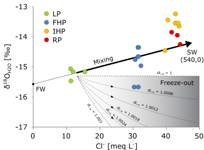
695 Figure 11 \text{Cl}^- concentration and \delta^{18}\text{O}_{\text{H}_2\text{O}} of pingo spring water samples. The thick black model line is drawn by assuming that the LP samples result from mixing of seawater and a freshwater endmember with a zero \text{Cl}^- concentration. The range of possible \delta^{18}\text{O}_{\text{H}_2\text{O}} -values following freeze-out (Eq. 8) from water with an initial composition alike LP is illustrated with the shaded area. Here, \text{Cl}^- is assumed to be
