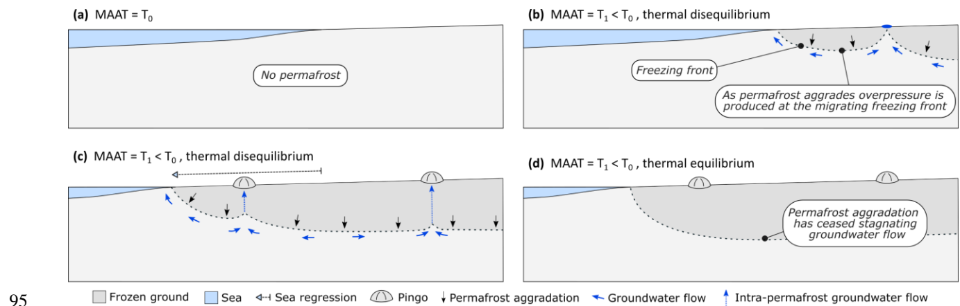
Figure 1 Conceptual model of pingo formation driven by permafrost aggradation in a low-permeable system. (a) No permafrost is present. (b) and (c) A negative shift in the surface energy balance results in permafrost aggradation. Freezing pressure is induced at the freezing front and this results in hydraulic head gradients. At some distance inland, higher advective heat transfer, associated with higher groundwater velocities, prevents the ground from freezing and groundwater flows to the surface where a pingo forms at the spring. (d) The ground is in thermal equilibrium with the MAAT, permafrost aggradation has stagnated, and groundwater flow to the pingos has ceased.
