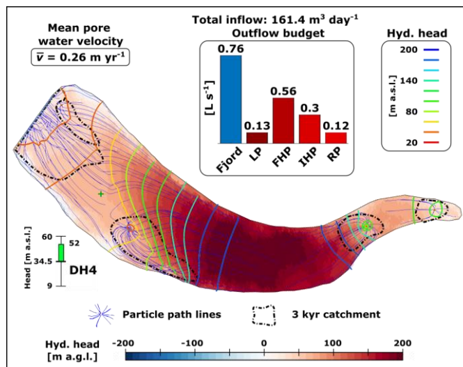
Figure 10 Groundwater model simulation representing additional pressure sources. Recharge is distributed uniformly with a rate of 1 mm yr -1 . This figure uses the same structure and legend as in Figure 8.
