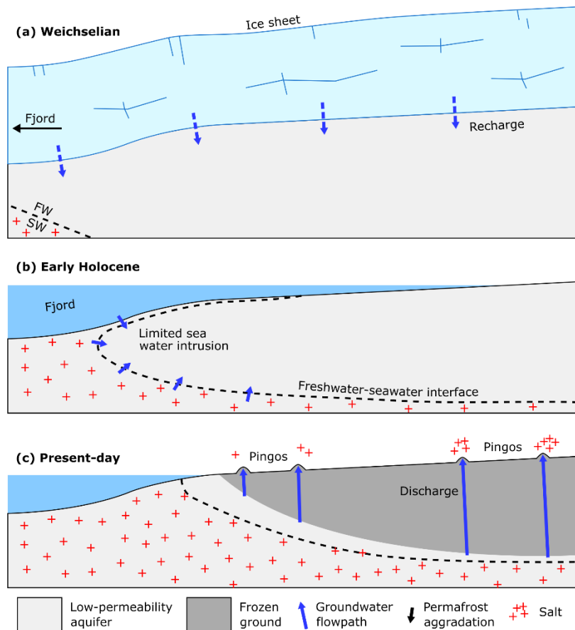
725 Figure 12 Possible interpretation of hydrochemical trends observed in pingo spring waters. (a) Subglacial melting from the Weichselian ice sheet recharged the groundwater system with freshwater. (b) Although covered by the sea during Early Holocene, low-permeability rocks limited infiltration of sea water and the fresh groundwater body persisted. (c) Due to the shallower permafrost depth towards the sea, spring water sampled in this direction holds a lower concentration of sea water (salt).
