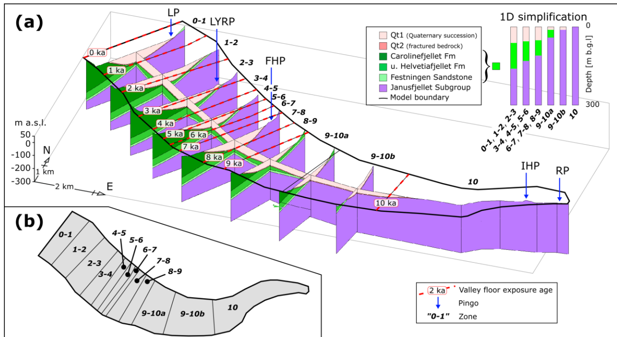
300 Figure 5 (a) 3D geological model of the subsurface below the valley floor in Adventdalen and vertical 1D simplifications (inset in upper 305 right corner) below zones of the model area. The former determines the hydrogeological properties in the groundwater model (Table 3), whereas the latter determines the geothermal properties in the 1DHT model (Table 2). The domain of the 1DHT model extends to 1000 m b.g.l. (not shown). Deeper than 300 m b.g.l., geothermal properties were defined as for Janusfjellet Subgroup. The sea retreat reconstruction was inferred from absolute datings (Table 1) and is illustrated by valley floor exposure isochrones (red dashed lines). Pingos are indicated with blue arrows. (b) Vertical view of the model area showing the zonation. The aforementioned isochrones defined the zone names so that the valley floor exposure age of a zone is apparent from its name (i.e., zone 0-1 became sub-aerially exposed between 1 and 0 ka, zone 1-2 between 2 and 1 ka, etc.).
