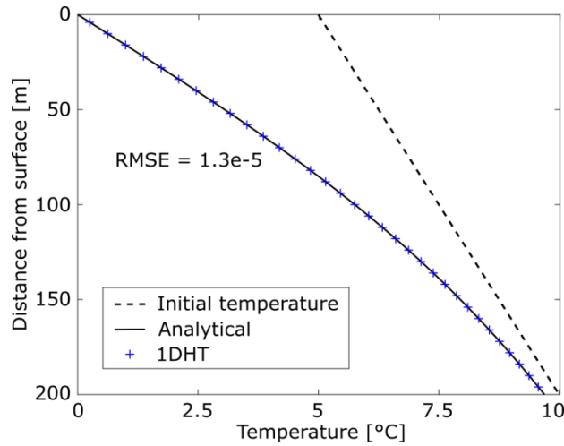
75 Figure S3 Comparison of the ground temperature distribution at t = 1000 yr calculated analytically (Eq. S6) and as simulated by the 1DHT model.
