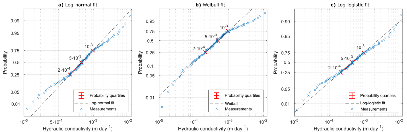
Figure S5-S4 Weibull-Log-normal (a), Weibull (b) and log-logistic (c) fits fit to the measured hydraulic conductivities of Carolinefjellet and Helvetiafjellet formations. Original data from the Longyearbyen CO 2 Laboratory Project (Olausson et al., 2020, and references therein). The log-logistic fit shows the best correlation with the measured values and the values used in the groundwater model were thus defined by the quartiles predicted by this fit. Note that the two other fits both predict the same quartiles.
