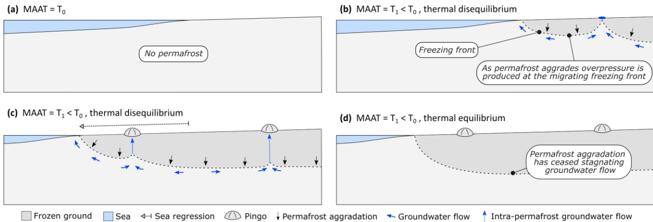
100 Figure 1 Conceptual model of pingo formation driven by permafrost aggradation in a low-permeable system. (a) No permafrost is present. (b) and (c) A negative shift in the surface energy balance results in permafrost aggradation. Freezing pressure is induced at the freezing front and this result ing ing in hydraulic head gradients. At some distance inland, higher advective heat transfer, associated with higher groundwater and where a spring (or pingo) forms at the spring. spring (d) The ground is in thermal equilibrium with the MAAT, permafrost aggradation has stagnated, and groundwater flow to the pingos has ceased.
