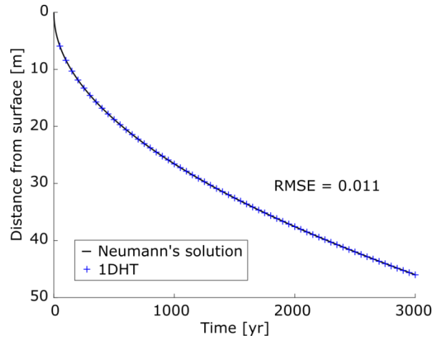
55 Figure S2 Freezing front depth with time in a body of water under Neumann conditions (see text) as calculated by the numerical 1DHT model and the analytical Neumann's solution.
