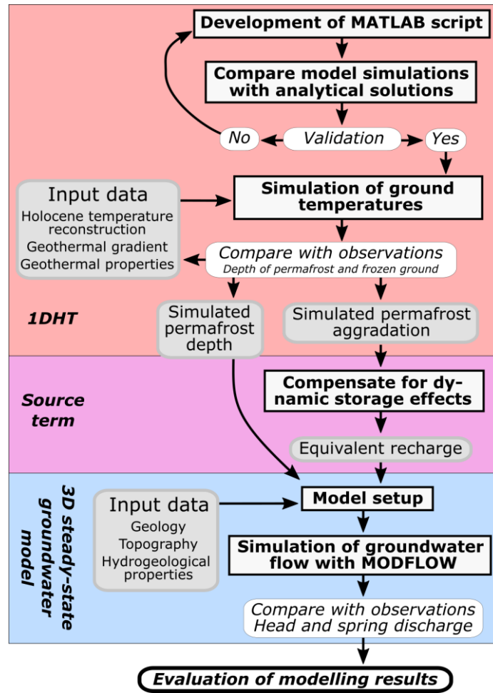
235 Figure 4 Schematic overview of the inner workings of the decoupled heat and groundwater model. Model setup, calculations and algorithms are indicated with sharp corners and bold text. Validation and comparison of simulations and observations are indicated with round corners and italics. Input and output data are indicated with rounded corners, grey background and normal text.
