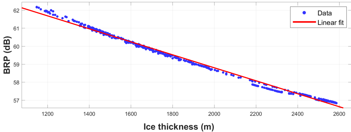
Figure 2. Example of the ice-attenuation correction for a window of PASIN radar data (BBAS line B01: SL2 in Fig.7). The red best fit line is a log of normalized power representing the BRP dependency to ice thickness.
