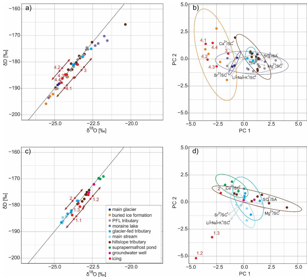
825 Figure 8. Isotopic and hydrochemical results for the Duke watershed. Panels (a) and (b) show icings and sources within the proglacial field; panels (c) and (d) show icings and sources within the alpine meadow. Panels (a) and (c) show results from stable water isotope analysis. The straight dashed line represents the Local Meteoric Water Line. Red arrows define the range within which samples from parent sources are considered to plot close to the icing sample. For samples from Icing 4, only arrows for the most depleted and the less depleted samples are included for readability. Panels (b) and (d) show results of hydrochemical analysis, and the ellipse illustrates the 95% confidence interval.
