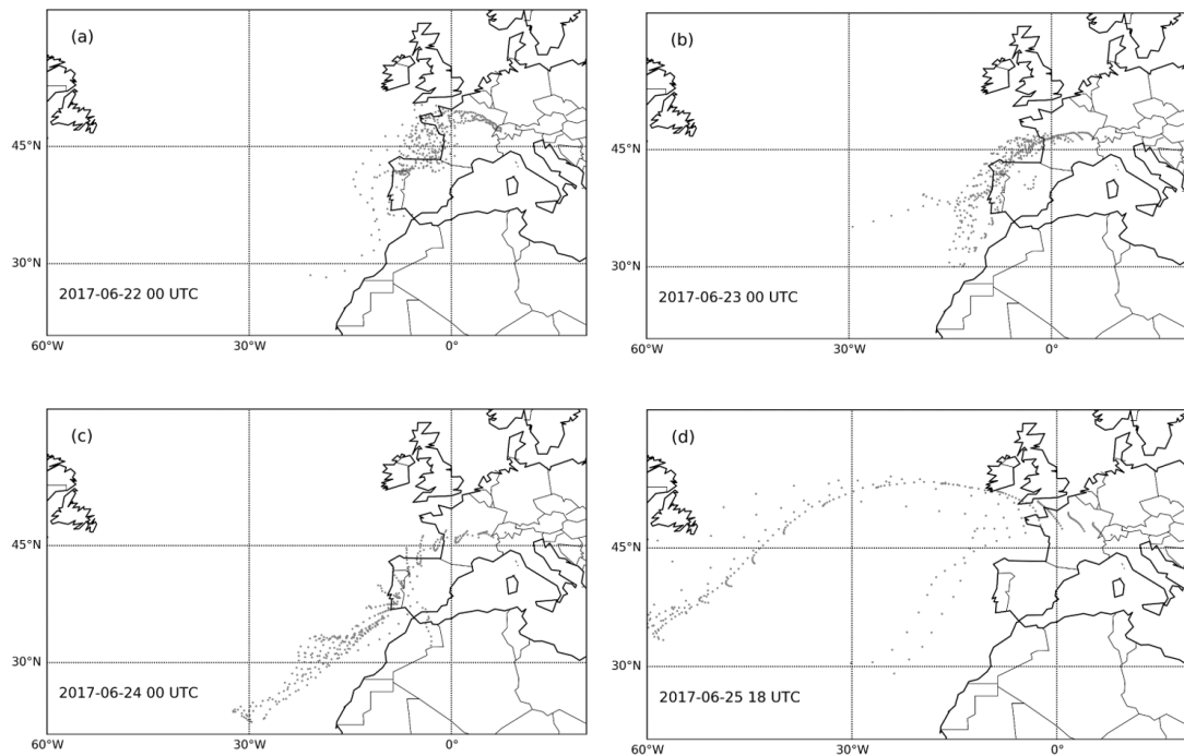
Fig. 1. Figure 4: 5-day air mass backward trajectories starting from the Jungfraujoch site at 00 UTC on 22nd to 24th June 2017. For 25th June starting time is 18 UTC.
