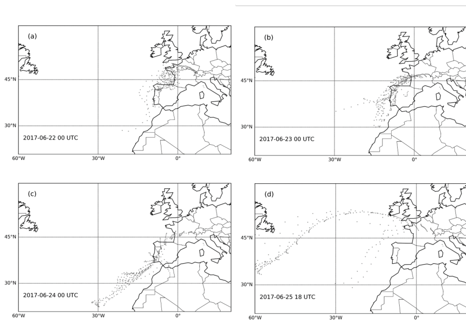
Fig. 1. Figure 4: 5-day air mass backward trajectories starting from the Jungfrauoch site at 00 UTC on 22nd to 24th June 2017. For 25th June starting time is 18 UTC.
