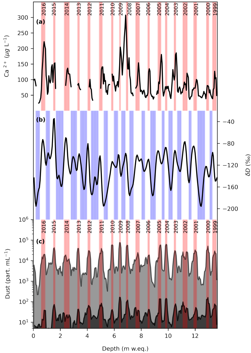
Figure 2. Dating of the Nevado Illimani firn core by annual layer counting (ALC) based on different proxies discussed in the text: (a) ionic Calcium, (b) \delta D , and (c) total and giant dust particles concentrations (light and dark gray, respectively, both are in logarithmic scale). Red and blue shaded vertical bands correspond respectively to the dry and wet season for each calendar year. All data are reported as 3-point running average of data re-sampled at 0.05 mw.eq.
