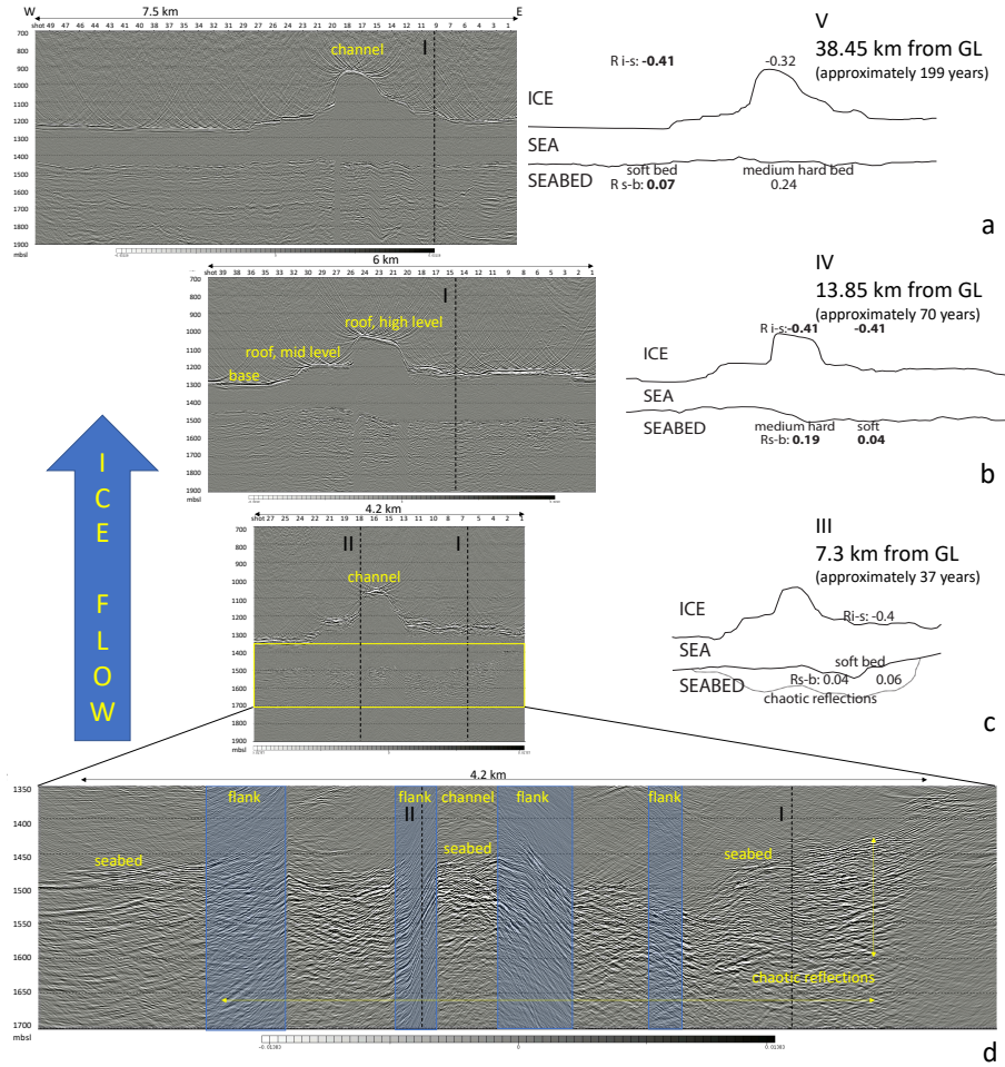
Figure 3. Profiles III, IV and V, and their schematic diagram , diagrams showing the development of the basal channel, and a zoom of the seabed of profile III . The calculated reflection coefficients (bold represents calibrated shots) are shown at their position in the diagram diagrams . The ice flow sequence is from bottom to top. The crossing-crossings of the profile profiles I is and II are marked by the black dashed lines. The distance from the GL and the time lap for the ice to reach this distance is mentioned on the right side. The three profiles have been aligned across-flow with respect to the most westerly flow line of Figure 1a. (a) The most downstream profile V, with the high-level roof of the channel marked. (b) Profile IV, for clarity the high and mid-level roof of the channel as well as the base are marked. (c) The most upstream profile III. The yellow frame marks a zoom of the seabed shown in (d) . The sedimentary sequence with chaotic reflections is marked in the schematic diagram by the dashed line. (d) The seabed of profile III showing the extend of the sedimentary sequence with chaotic reflections, also marked by the yellow arrows. The shaded rectangles mark the flanks of the basal channel where the depth conversion and morphology of the seabed break down.
