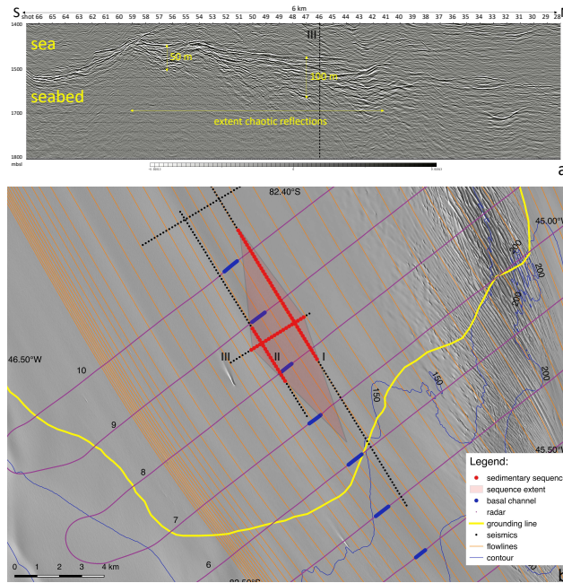
Figure 4. The extent of the sedimentary sequence with chaotic reflections at profile II (a) and its lateral extent over profiles I, II and III (b). (a) The seabed of profile II with the ice flow from left to right. The sedimentary sequence is marked by the yellow double headed arrows, the horizontal arrow marking the lateral extent and the two vertical arrows marking the thicknesses at two cavities. The crossing with profile III is marked by the black dashed line. (b) The seismic (black dots) and radar survey (purple lines) of the GL area showing the seismic shots (red dots) that recorded the sedimentary sequence with chaotic reflections on profiles I, II and III. The red shaded area marks the outer boundaries of the sedimentary sequence by using linear interpolation. The grounding line is marked in yellow. The basal and subglacial channel are marked by the blue dots. The background is a shaded version of the 8 m Reference Elevation Model of Antarctica (REMA, Howat et al. 2019).
