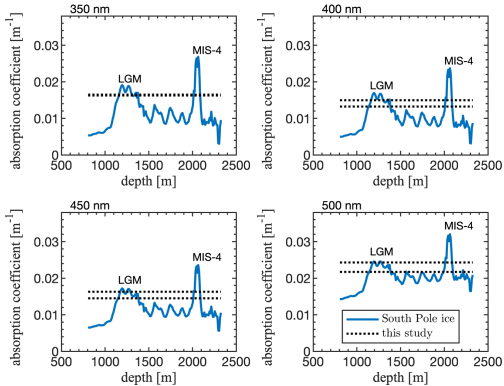
Fig. 11: Depth profiles of South Pole ice absorptivity at four wavelengths obtained from Eq. 26 and Table 3 of Ackermann et al. (2006). The 1% K -1 temperature dependence of pure ice absorptivity (Woschnagg and Price, 2001) is removed for comparison with this study's lower (Layer B) and upper (Layer A) absorption coefficient estimate at each wavelength (dashed lines). Values reported in this study are consistent with South Pole values at depths corresponding to the Last Glacial Maximum and Marine Isotope Stage 4 when atmospheric dust concentrations peaked in both hemispheres. Note that South Pole age does not map to ice near the Greenland Ice Sheet margin. Rather, Southern Hemisphere dust concentrations during these periods are consistent with Northern Hemisphere dust concentrations during warm interglacial periods and/or periods with low aeolian activity (Muhs, 2013; Reeh et al., 2002).
