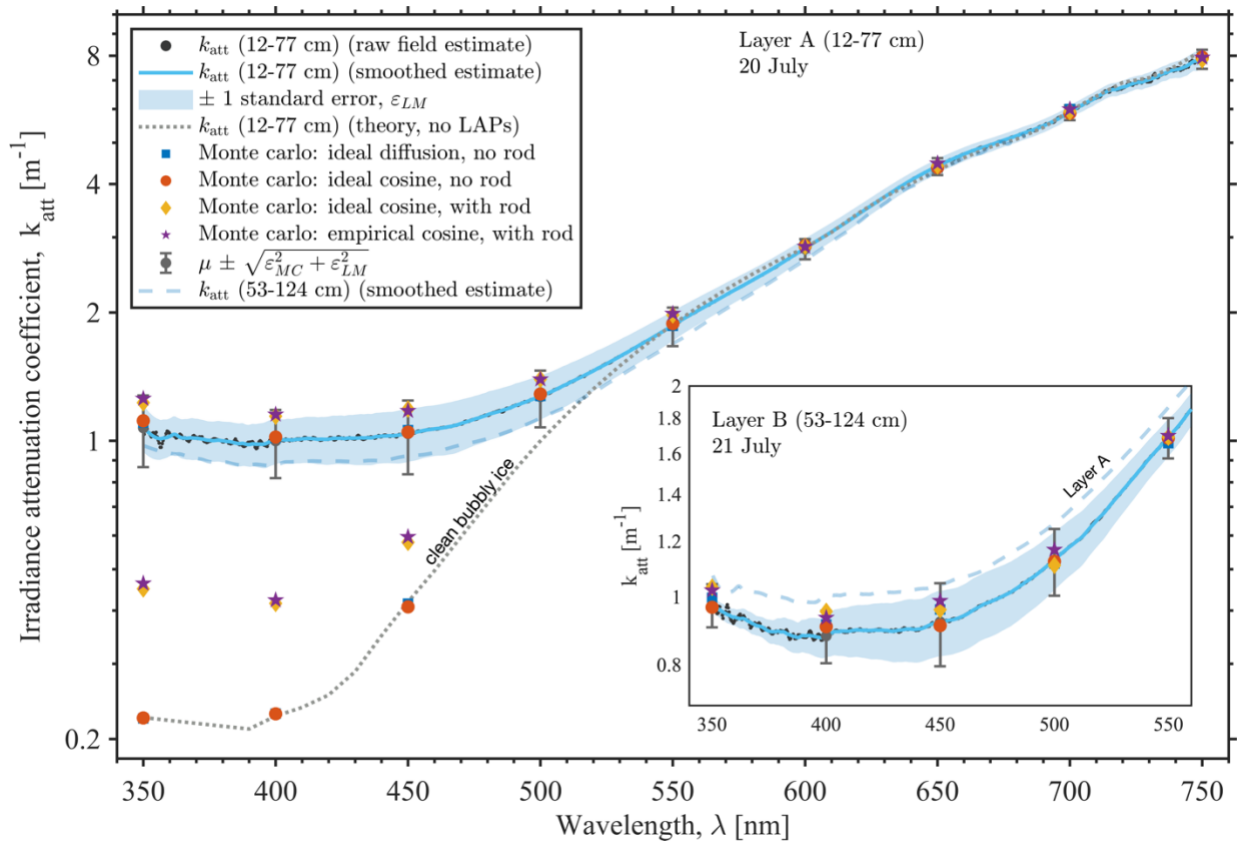
Fig. 6: Visible and near-UV attenuation coefficient k_{\text{att}} spectra from measurements of light transmission in bare glacier ice collected on 20 July 2018 at 12–77 cm depth below the ice sheet surface. Field estimates are compared with asymptotic two-stream theory for optically clean bubbly ice (continuous dotted line) and with values at nine wavelengths from four simulations with a 3-dimensional Monte Carlo radiative transfer model (solid symbols). Monte Carlo values for clean bubbly ice are shown for 350, 400, and 450 nm to demonstrate detector interference at these wavelengths; values at wavelengths >550 nm converge with field spectra and are omitted for clarity. Two measures of uncertainty are shown: 1) statistical linear model uncertainty \varepsilon_{LM} (shaded uncertainty bounds; \pm 1 standard error in the linear regression) and, 2) \varepsilon_{LM} combined with systematic uncertainty \varepsilon_{MC} due to detector interference estimated with Monte Carlo (error bars; \mu \pm \varepsilon ). The same comparison for the 21 July experiment (inset) suggests detector interference is lower and within statistical uncertainty at wavelengths >400 nm.
