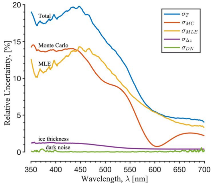
Fig. 9: Uncertainty budget for reported asymptotic attenuation coefficient k_{\text{att}} values for Layer A (12–77 cm) (20 July experiment). Systematic uncertainties examined include spectrometer sensitivity to dark noise, ice thickness (detector position) measurement uncertainty, the non-ideal angular response of the irradiance sensor, and scattering and absorption interference by the polyvinyl chloride detector rod (estimated with Monte Carlo simulation). These systematics are summed in quadrature with statistical uncertainty represented by one standard error in the Maximum Likelihood Estimate (MLE) linear regression fits. Values for Layer B (53–124 cm) (not shown) are qualitatively similar but <14\% in the region of maximum uncertainty.
