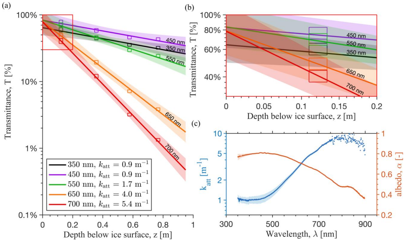
870 Fig. 5: (a) Sample linear regressions between measured transmittance (indicated by rectangles with width and height proportional to measurement uncertainty in both variables) and depth for five representative wavelengths spanning the measured spectral range. The slope of each line is the attenuation coefficient k_{\text{att}} . Shaded bounds are \pm 95\% confidence intervals from a two-sided t-distribution. (b) Red box inset in (a) shows the y-axis intercept of each regression is less than 100%, indicating the magnitude of deviation from Bouguer's law near the surface. (c) Spectral k_{\text{att}} (blue dots with shaded uncertainty; left axis) and spectral albedo (red dots with shaded uncertainty; right axis). Beyond \sim 700 nm, in-ice transmitted irradiance is too low to reliably estimate k_{\text{att}} (see Fig. 4a and Fig. 2c), as indicated by the increased scatter in k_{\text{att}} values. 875
