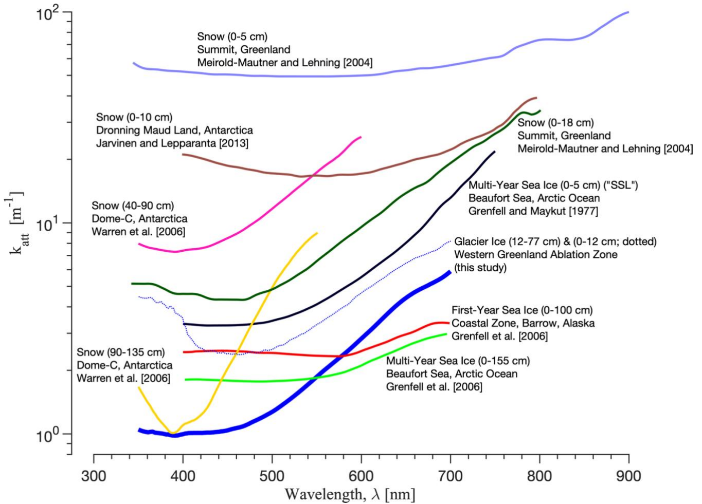
915 Fig. 10: Attenuation coefficient spectra for seven distinct ice structures (from lower left clockwise): interior of clean, dry snowpack ( r_{\text{eff}} \approx 10^{-5} m) near Dome-C in Antarctica for two depth regions (90–135 cm and 40–90 cm) (Warren et al., 2006), near-surface (0– 10 cm) dry snowpack ( r_{\text{eff}} \approx 10^{-3} m) in Dronning Maud Land, Antarctica (Järvinen and Leppäranta, 2013), near-surface (0–5 cm) and interior (0–18 cm) dry snowpack ( r_{\text{eff}} \approx 10^{-4} m) near Summit, Greenland (Meirolid-Mautner and Lehning, 2004), surface 920 scattering layer (SSL; 0–5 cm) of multi-year sea ice in the Arctic Ocean (Grenfell and Maykut, 1977), interior of ablating glacier ice in Greenland (this study) (12–77 cm in solid line; 0–12 cm in dotted line), interior of first-year sea ice in the coastal zone near Barrow, Alaska (Grenfell et al., 2006), and interior of multi-year sea ice in the Arctic Ocean (Grenfell et al., 2006). Differences in attenuation magnitude at each wavelength are mostly controlled by structural differences that control scattering, whereas spectral differences are mostly controlled by differences in type and concentration of absorbing impurities.
