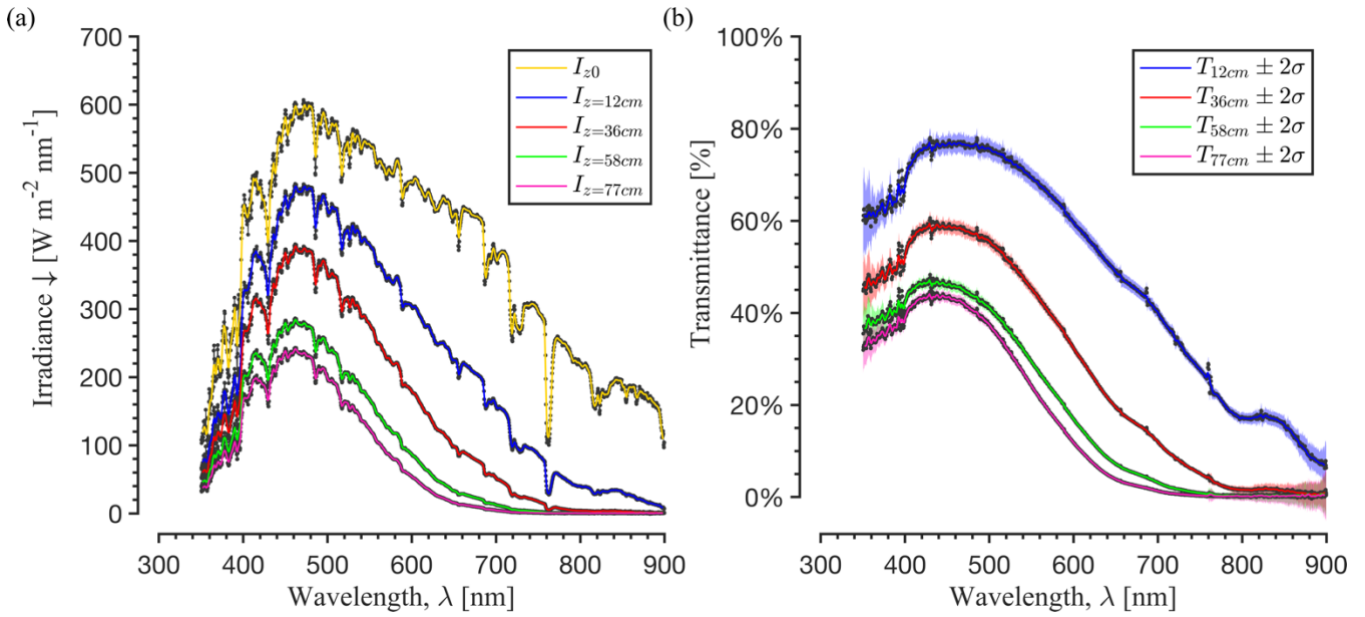
Fig. 4: (a) Field spectra of surface downwelling ( z = z_0 ) and in-ice irradiance at four depths below the ice surface collected on 20 July 2018 between 13:45 and 14:35 local time in the western Greenland ablation zone (67.15 °N, 50.02 °W). Raw data were recorded at 1 Hz frequency for 30 seconds, yielding 30 irradiance profiles at each depth. Shown here are 30-second averages at \sim 0.35 nm spectral resolution for each depth (black dots), and 1-nm interpolated values smoothed with a 3-nm centred moving mean filter for clarity (continuous lines). (b) Transmittance at each depth, with 30-second averages (black dots), 1-nm interpolated values (continuous lines), and shaded bounds ( \pm 2\sigma ) representing propagated measurement uncertainty deduced from the standard deviations of the 1 Hz raw data ( N=30 for each value).
