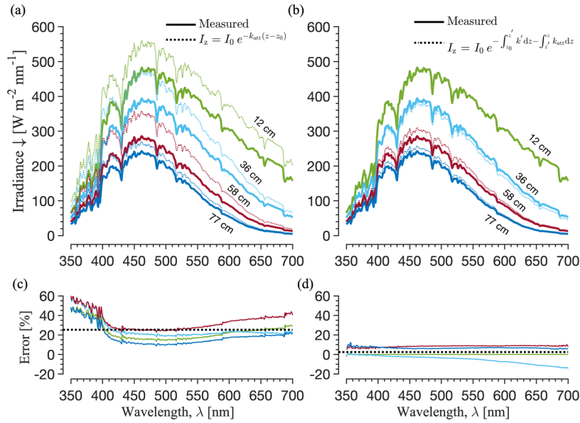
Fig. 8: Measured in-ice irradiance compared with: (a) Bouguer's law (Eq. 7) with no modification, and (b) the piece-wise Bouguer law (Eq. 16). The error structure (c–d) provides insight into the near-surface attenuation processes: relative errors (%) are positive (model under-predicts attenuation) at all wavelengths but are highest in the near-UV, lowest in the blue, and increase monotonically into the red end of the visible spectrum. (d) errors are small, and generally decrease monotonically with increasing wavelength. Taken together, near-surface attenuation enhancement is on the order 10–60%.
