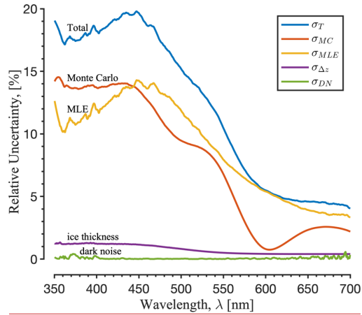
095 100 Fig. 9: Uncertainty budget for reported asymptotic attenuation coefficient k_{att} values for Layer A (12–77 cm) (20 July experiment). Systematic uncertainties examined include spectrometer sensitivity to dark noise, ice thickness (detector position) measurement uncertainty, the non-ideal angular response of the irradiance sensor, and scattering and absorption interference by the polyvinyl chloride detector rod (estimated with Monte Carlo simulation). These systematics are summed in quadrature with statistical uncertainty represented by one standard error in the Maximum Likelihood Estimate (MLE) linear regression fits. Values for Layer B (53–124 cm) (not shown) are qualitatively similar but <14% in the region of maximum uncertainty.
