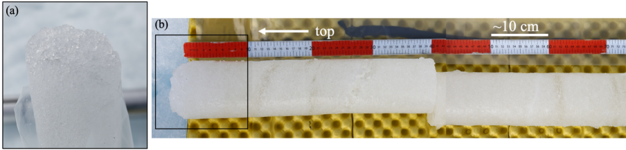
Fig. 3: Photographs of an ice core collected at the field site. (a) The upper few centimetres of ice is semi-granular, with ~4 cm of unrecovered granular ice not shown. (b) The 122 cm ice core was broken into three segments corresponding to depths of 4–45 cm, 45–74 cm, and 74–122 cm below the ice surface (the far right of the image in (b) is at 74 cm). The density of these segments is 801 \text{ kg m}^{-3} , 884 \text{ kg m}^{-3} , and 888 \text{ kg m}^{-3} , respectively. Below ~10 cm, the bubbly ice appears foliated, reflecting variations in bubble density and size distribution that affect scattering. Black box in (b) is approximately the image area in (a).
