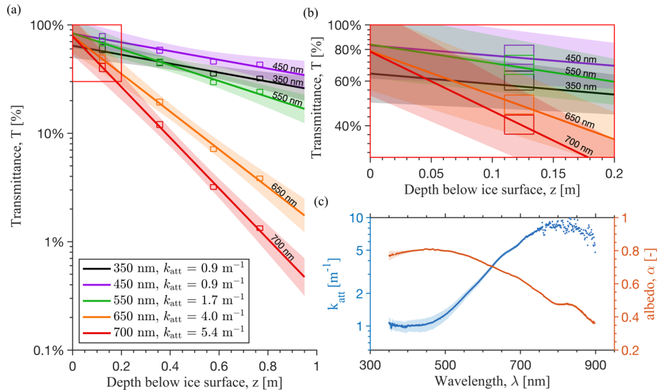
Fig. 5: (a) Sample linear regressions between measured transmittance (indicated by rectangles with width and height proportional to measurement uncertainty in both variables) and depth for five representative wavelengths spanning the measured spectral range. The slope of each line is the attenuation coefficient k_{att} . Shaded bounds are \pm 95\% confidence intervals from a two-sided t-distribution. (b) Red box inset in (a) shows the y-axis intercept of each regression is less than 100%, indicating the magnitude of deviation from Bouguer's law near the surface. (c) Spectral k_{att} (blue dots with shaded uncertainty; left axis) and spectral albedo (red dots with shaded uncertainty; right axis). Beyond \sim 700 nm, in-ice transmitted irradiance is too low to reliably estimate k_{att} (see Fig. 4a and Fig. 2c), as indicated by the increased scatter in k_{att} values.
