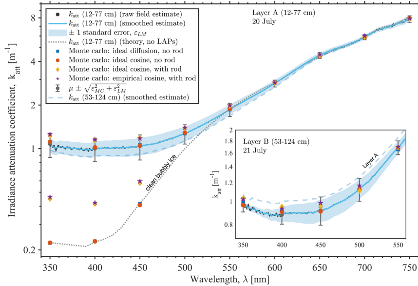
1065 Fig. 6: Visible and near-UV attenuation coefficient k_{\text{att}} spectra from measurements of light transmission in bare glacier ice collected 1070 on 20 July 2018 at 12–77 cm depth below the ice sheet surface. Field estimates are compared with asymptotic two-stream theory for optically clean bubbly ice (continuous dotted line) and with values at nine wavelengths from four simulations with a 3-dimensional Monte Carlo radiative transfer model (solid symbols). Monte Carlo values for clean bubbly ice are shown for 350, 400, and 450 nm to demonstrate detector interference at these wavelengths; values at wavelengths >550 nm converge with field spectra and are omitted for clarity. Two measures of uncertainty are shown: 1) statistical linear model uncertainty \varepsilon_{LM} (shaded uncertainty bounds; \pm 1 standard error in the linear regression) and, 2) \varepsilon_{LM} combined with systematic uncertainty \varepsilon_{MC} due to detector interference estimated with Monte Carlo (error bars; \mu \pm \varepsilon ). The same comparison for the 21 July experiment (inset) suggests detector interference is lower and within statistical uncertainty at wavelengths >400 nm.
