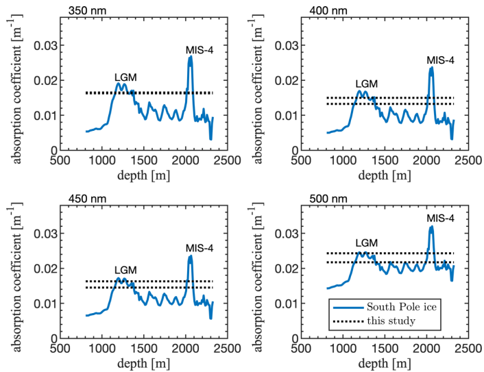
1115 Fig. 11: Depth profiles of South Pole ice absorptivity at four wavelengths obtained from Eq. 26 and Table 3 of Ackermann et al. (2006). The 1% \text{K}^{-1} temperature dependence of pure ice absorptivity (Woschnagg and Price, 2001) is removed for comparison with this study's lower (Layer B) and upper (Layer A) absorption coefficient estimate at each wavelength (dashed lines). Values reported in this study are consistent with South Pole values at depths corresponding to the Last Glacial Maximum and Marine Isotope Stage 4 when atmospheric dust concentrations peaked in both hemispheres. Note that South Pole age does not map to ice near the Greenland Ice Sheet margin. Rather, Southern Hemisphere dust concentrations during these periods are consistent with Northern Hemisphere dust concentrations during warm interglacial periods and/or periods with low aeolian activity (Muhs, 2013; Reeh et al., 2002). 1120
