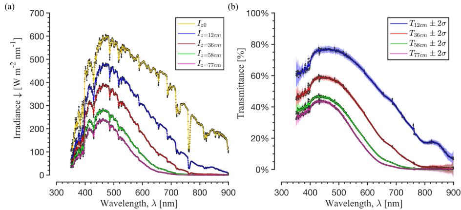
040 Fig. 4: (a) Field spectra of surface downwelling ( z = z_0 ) and in-ice irradiance at four depths below the ice surface collected on 20 045 July 2018 between 13:45 and 14:35 local time in the western Greenland ablation zone (67.15 °N, 50.02 °W). Raw data were recorded at 1 Hz frequency for 30 seconds, yielding 30 irradiance profiles at each depth. Shown here are 30-second averages at ~0.35 nm spectral resolution for each depth (black dots), and 1-nm interpolated values smoothed with a 3-nm centred moving mean filter for clarity (continuous lines). (b) Transmittance at each depth, with 30-second averages (black dots), 1-nm interpolated values (continuous lines), and shaded bounds ( \pm 2\sigma ) representing propagated measurement uncertainty deduced from the standard deviations of the 1 Hz raw data ( N=30 for each value).
