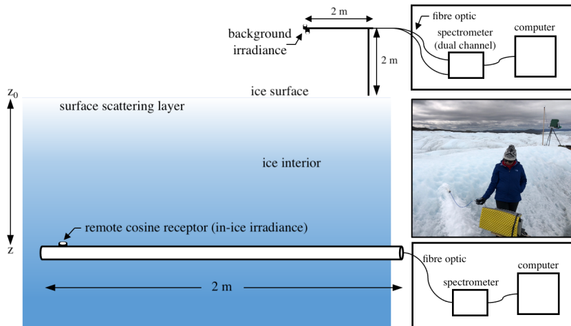
Fig. 1: The irradiance sensor is comprised of a remote cosine receptor and fibre optic light guide fitted inside an insulated white PVC tube of 2 m length. Holes are drilled level and horizontal into the ice, the tube is inserted, and drill shavings are packed around the hole to prevent stray reflections. The cosine receptor collects the downwelling light, guides it to the fibre optic cable that transmits the light to an Ocean Optics® JAZ spectrometer, and a computer running the Ocean Optics® Ocean View software records the spectra. Background downwelling surface spectra are recorded on a 2 m mast drilled into the ice approximately 3 m to the northwest of the in-ice measurement location (see photo background). This photograph was taken on 21 July 2018 at ~13:22 local time (UTC-3).
