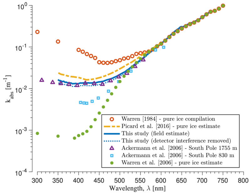
1125 Fig. 12: Estimates of ice absorption coefficient k_{\text{abs}} , obtained from five distinct sources: laboratory-grown pure ice (Grenfell and Perovich, 1981; Perovich and Govoni, 1991), as compiled in Warren (1984), snow in Antarctica, contaminated by trace concentrations of light absorbing particles (LAPs) (Picard et al., 2016), glacial ice in Greenland with unknown concentration of LAPs (this study), compressed glacial ice at 1755 m depth and 830 m depth in the Antarctic Ice Sheet contaminated by dust deposited 1130 during the late Pleistocene and Early Holocene, respectively (Ackermann et al., 2006), and snow in Antarctica with the effect of LAPs removed (pure ice estimate) (Warren et al., 2006). Values from this study with the detector interference subtracted are shown as dotted blue line.
