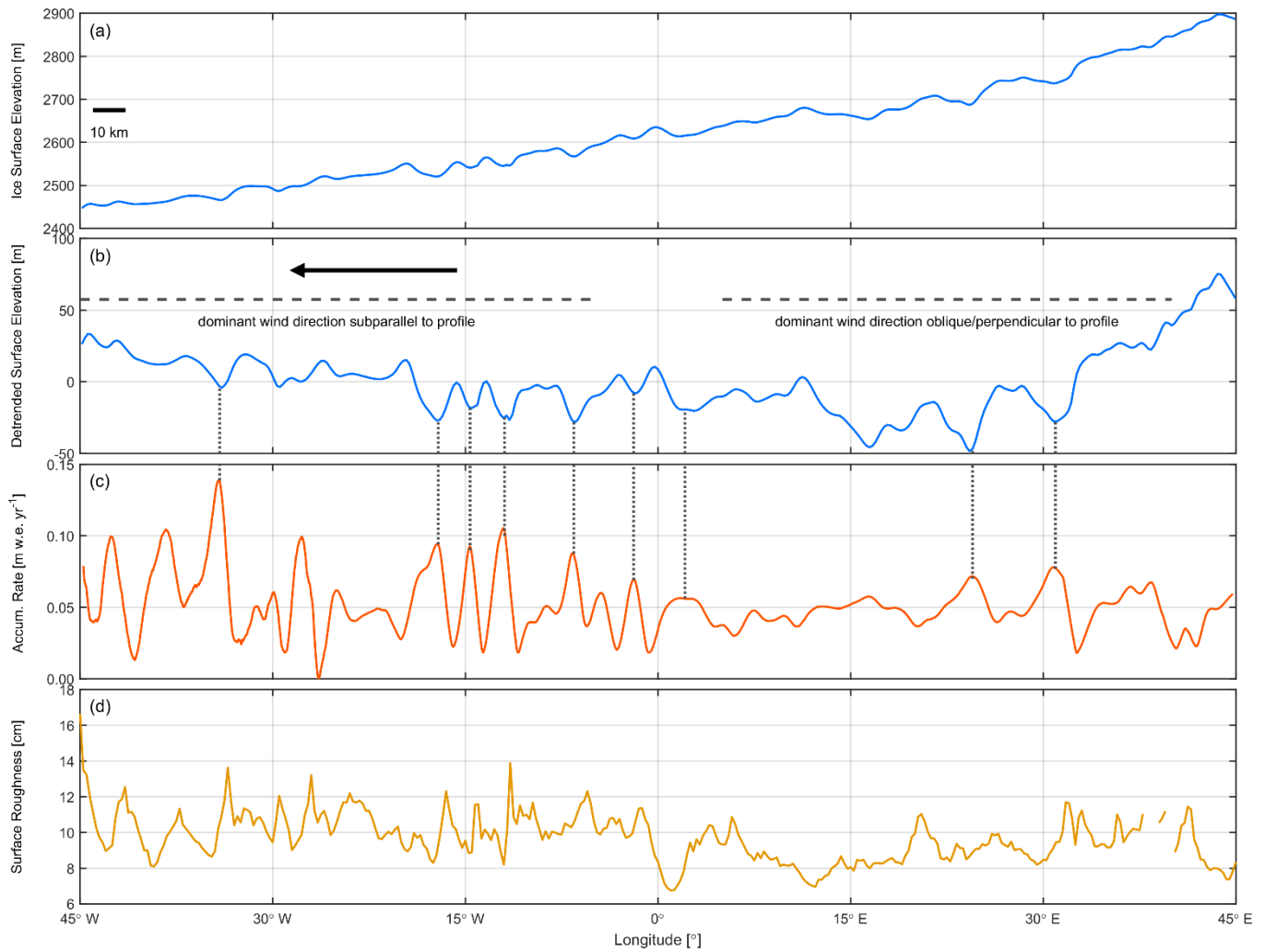
745 Figure A2: a) Ice surface elevation at 88° S between 45° W and 45° E from ATM laser altimetry. b) Ice surface elevation with linear trend removed. c) Snow accumulation rate. Several prominent peaks that spatially correlate with topographic depressions are marked by grey dashed lines. d) ATM derived ice surface roughness.
