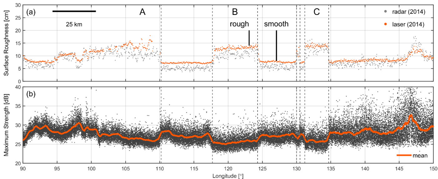
480 Figure 9: a) Surface roughness from 2014 ATM laser and CReSIS Ku-band radar data over roughness features “A”, “B”, and “C” (Fig. 4b). Vertical black lines mark the locations of radar waveforms over smooth and rough surfaces shown in Fig. A4. b) Maximum of relative return signal strength from 2014 snow radar data. Red line is a running mean calculated over 350 radar traces (~2 km), which is similar in size to the 1.65 km CryoSat-2 footprint in low resolution mode (LRM) over smooth surfaces (Scagliola, 2013). The strength of the surface return is around 3 dB weaker over rough areas compared to smooth areas.
