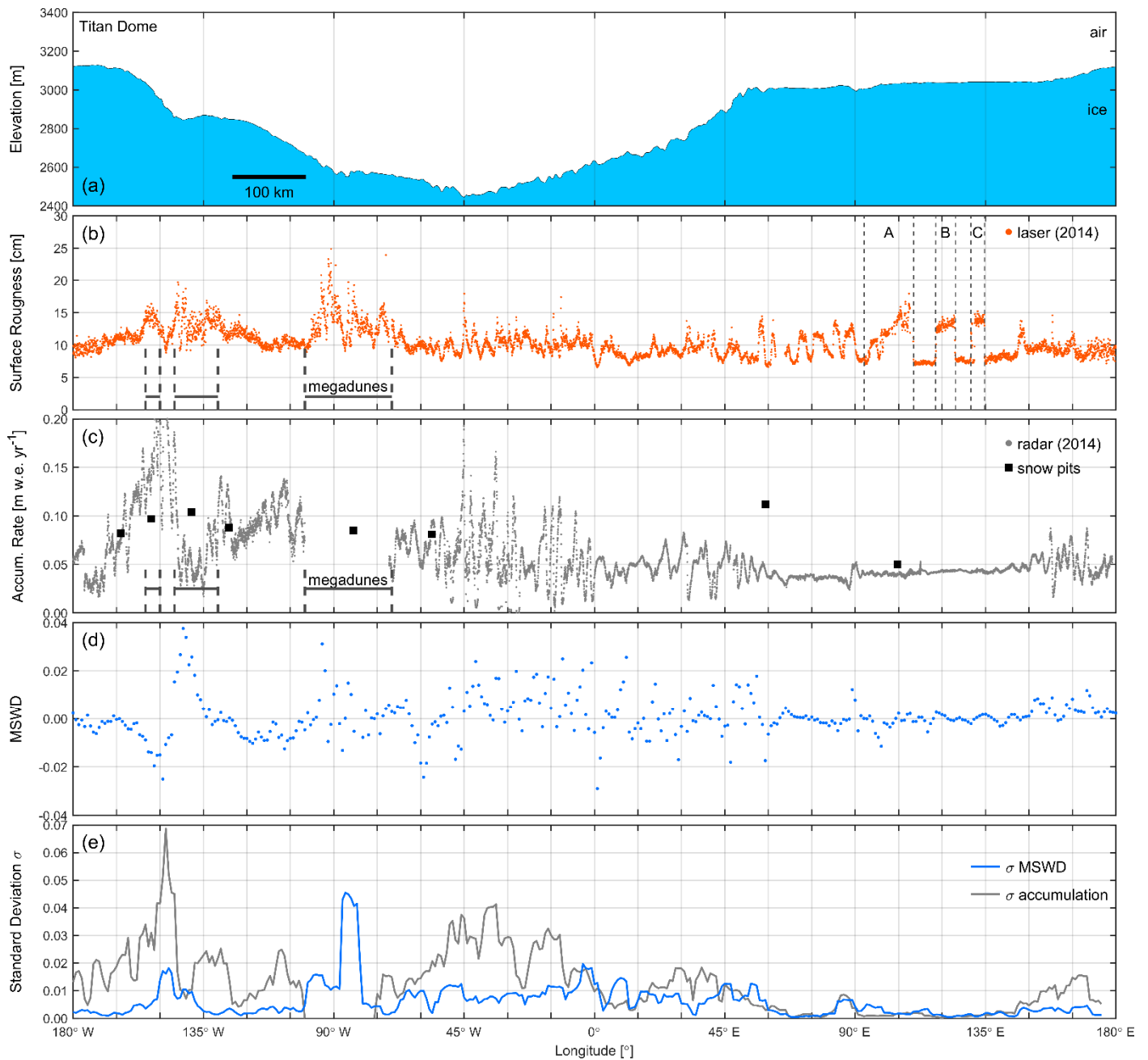
370 Figure 6: a) Ice surface elevation around 88° S from ATM laser altimetry. b) Surface roughness from ATM laser altimetry. c) Snow accumulation rate derived from 2014 snow radar data and tied to MERRA-2. A 14 minute disk failure of the snow and Ku-band radars in 2014 resulted in a data gap over the megadunes and therefore the accumulation rate. Squares indicate accumulation measurements from snow pit data within 10 km of 88° S (Favier et al., 2013; Taylor, 1971). d) Mean Slope in the mean Wind Direction (MSWD) in one degree longitude bins (4 km). e) Standard deviation \sigma of the MSWD and snow accumulation rate estimated over 20 km long segments.
