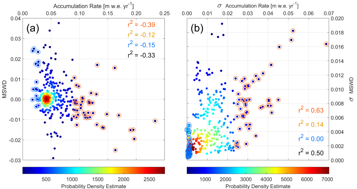
405 Figure 7: a) Mean Slope in the mean Wind Direction (MSWD) versus snow accumulation rate around 88° S in one degree longitude bins (4 km). Since monochrome scatter plots can be misleading we have used color coding to indicate regions with higher point density. Higher probability density estimates, calculated using a kernel estimate, are shown in warmer colors and indicate regions with higher point density. The probability density estimate is for visual clarity only and is not used for analysis or interpretation. Pearson's correlation coefficient r^2 = -0.33 for the entire data set. b) Same for the standard deviation \sigma of the MSWD and snow accumulation rate with r^2 = 0.50 . \sigma is estimated over 20-km-long moving windows. Data points below \mu - \sigma are indicated with blue circles and r^2 s are listed in blue.
