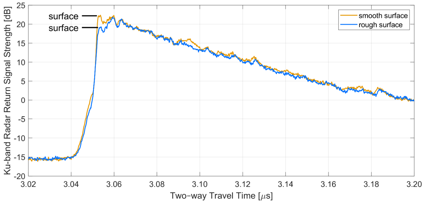
760 Figure A4: Relative Ku-band radar return signal strength over smooth and rough surfaces. 100 traces were stacked for the averaged waveforms. For location see Fig. 9. The difference between the radar waveforms indicates that radar altimeters are potentially prone to elevation errors when threshold or leading edge trackers are being used for range retrieval.
