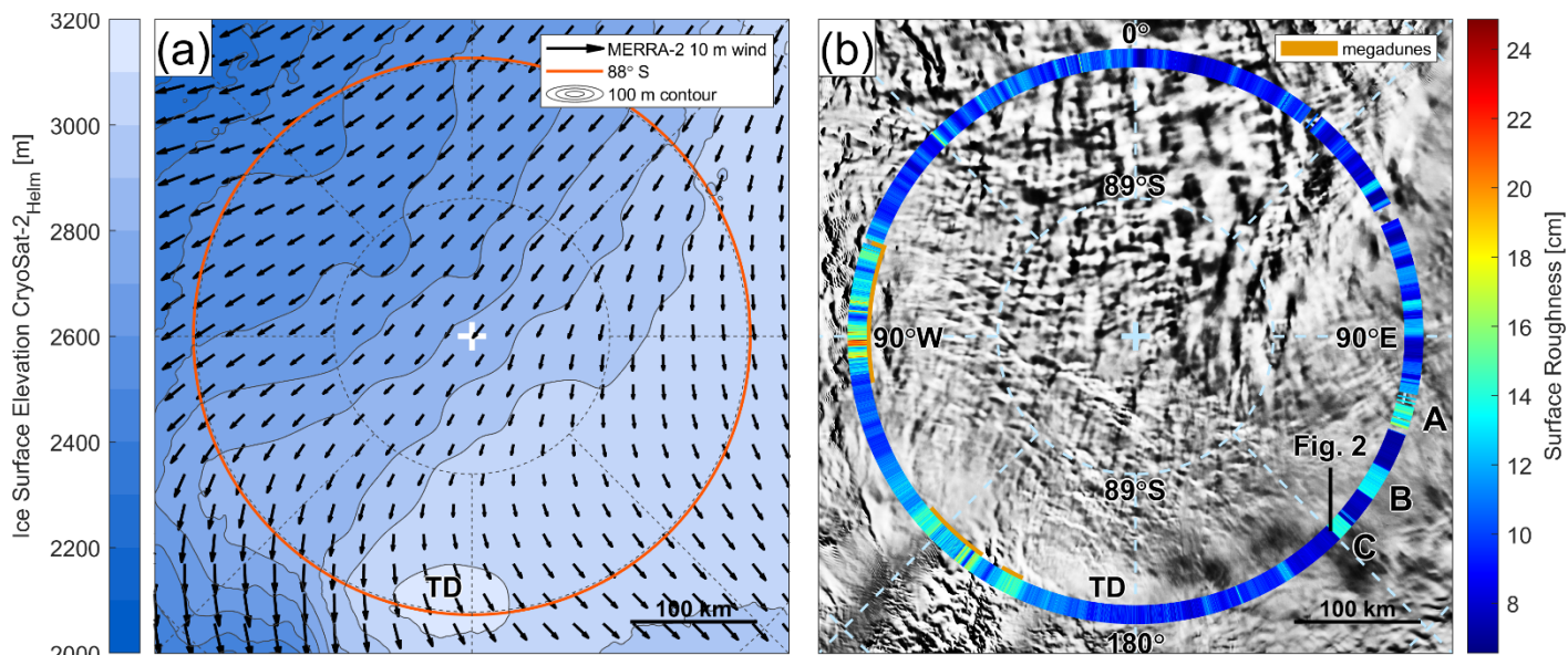
175 Figure 3: a) Ice surface elevation from CryoSat-2 (Helm et al., 2014) and 26 year 10 m average wind speed from MERRA-2 (e.g., Gelaro et al., 2017). Red line marks location of 88S° airborne geophysical data collection. TD is Titan Dome. b) Ice surface roughness from 2014 ATM data (Studinger, 2014, updated 2018). Background image is MODIS Mosaic of Antarctica 2013 – 2014 (Haran et al., 2014) using MODIS data between 11/2013 and 03/2014. Locations of megadune fields are marked in orange and roughness features A, B, and C refer to Fig. 4b.
