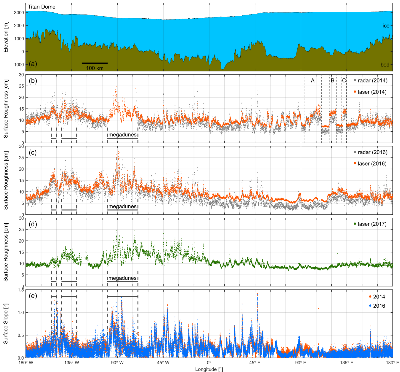
250 Figure 4: a) Ice surface elevation from 2014 ATM data (Studinger, 2014, updated 2018) and bedrock topography from 2014 CReSIS Multichannel Coherent Radar Depth Sounder (MCoRDS) data (Leuschen et al., 2010, updated 2018). b) Surface roughness from 2014 ATM laser and snow radar data. A 14 minute disk failure of the snow radar in 2014 resulted in a data gap over the megadunes. c) Same for 2016. d) Surface roughness from 2017 UAF laser data e) Surface slope from 2014 and 2016 ATM ICESSE data using only the nadir
