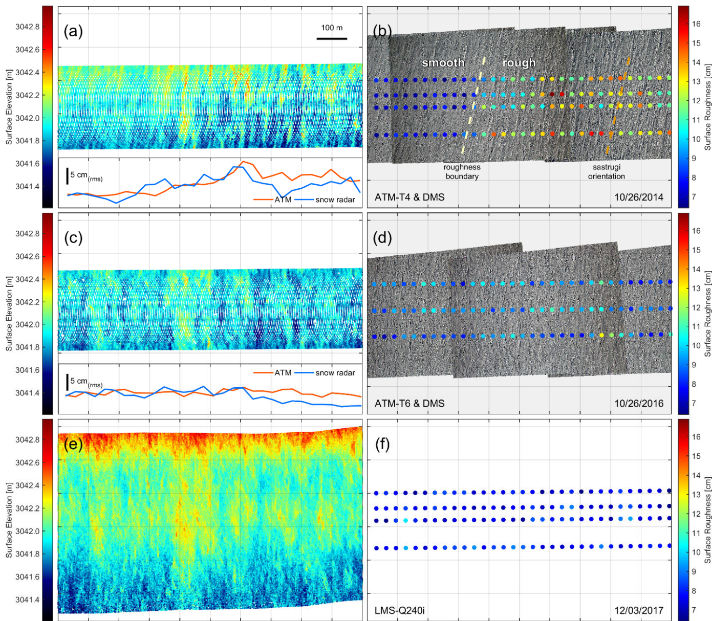
300 Figure 5: Laser spot elevation measurements and DMS imagery over roughness feature "C" (Fig. 4b). The center of all map panels is at 88.97^\circ S/ 135^\circ E. All panels cover the exact same area on the ground and are shown in a local coordinate system parallel to the aircraft trajectory. Panels a), c) and e) show laser spot elevation measurements in 2014, 2016 and 2017. Inset plots in a) and c) show surface roughness from ATM and snow radar at the center of the scan/nadir position. Panels a) and c) show small (cm level) semi-circular elevation biases that are a result of occasional variations in scan azimuth speed (Yi et al., 2015). The peak-to-peak amplitude of these biases is an order of magnitude smaller than the ice surface topography. Panels b), d) and f) show corresponding DMS imagery (b) and d) only) and surface roughness from laser altimetry in 2014, 2016, and 2016. The darkening towards the edge of the DMS frames in b) and d) is caused by vignetting from the lens and not related to geophysical changes. ATM roughness is from ICESN data and the UAF Riegler data from 2017 has been calculated in the same way as ATM ICESN data to make them compatible. A distinct change in roughness can be seen in 2014 that is visible in both, the laser derived surface roughness, and the length of the shadows in DMS imagery (b). The roughness doubles over a distance of \sim 200 m (a). The orientation of the boundary is parallel to the dominant sastrugi orientation (b). In 2016 and 2017 the distinct change in roughness seems to have been smoothed out. 305
