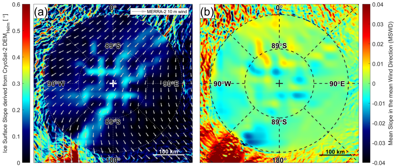
740 Figure A1: a) Ice surface slope in degrees derived from CryoSat-2 (Helm et al., 2014) and 26 year 10 m wind average from MERRA-2 (e.g., Gelaro et al., 2017). b) Mean Slope in the mean Wind Direction (MSWD).
