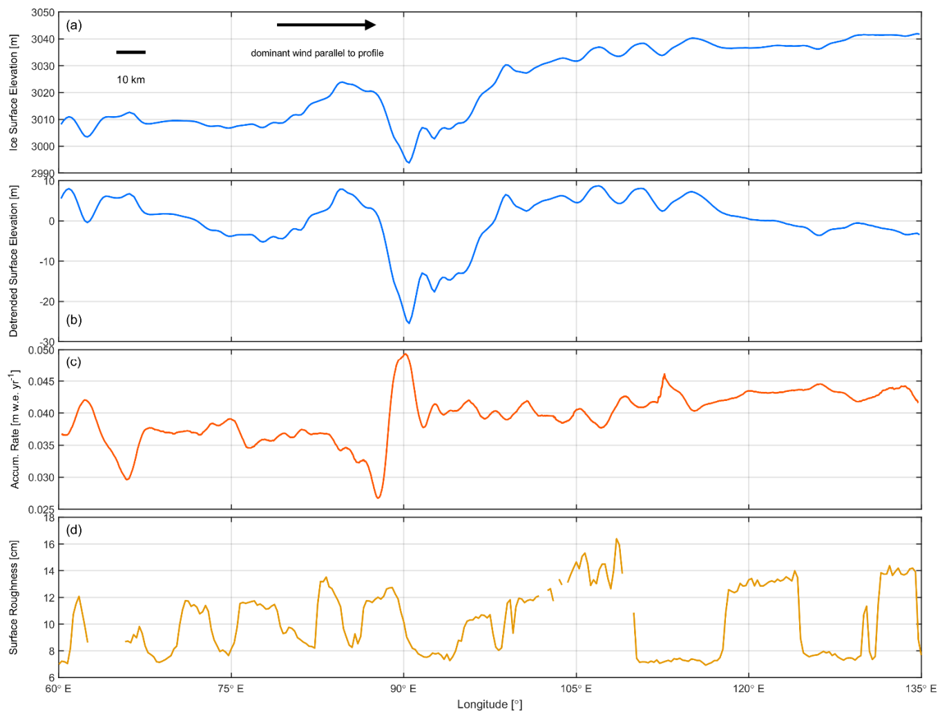
755 Figure A3: a) Ice surface elevation between 60° E and 135°E from ATM laser altimetry. The dominant wind direction from MERRA-2 is parallel to the profile segment. b) Ice surface elevation with linear trend removed. c) Snow accumulation rate were the pronounced peak at 90° E corresponds to the topographic depression in the ice surface. d) ATM derived ice surface roughness.
