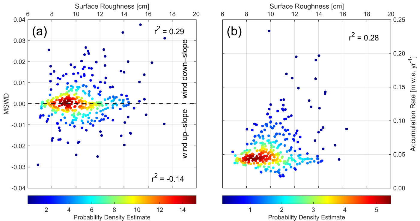
450 Figure 8: a) ATM derived surface roughness versus Mean Slope in the mean Wind Direction (MSWD) around 88° S in one degree longitude bins (4 km). Color indicates the probability density estimate of nearby points using a kernel density estimate. Pearson's correlation coefficients r^2 are calculated for up-slope winds (MSWD < 0) and down-slope winds (MSWD > 0). b) Same for surface roughness versus accumulation rate.
