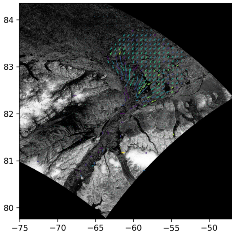
Fig. 1. Ice motion results using feature tracking method.
