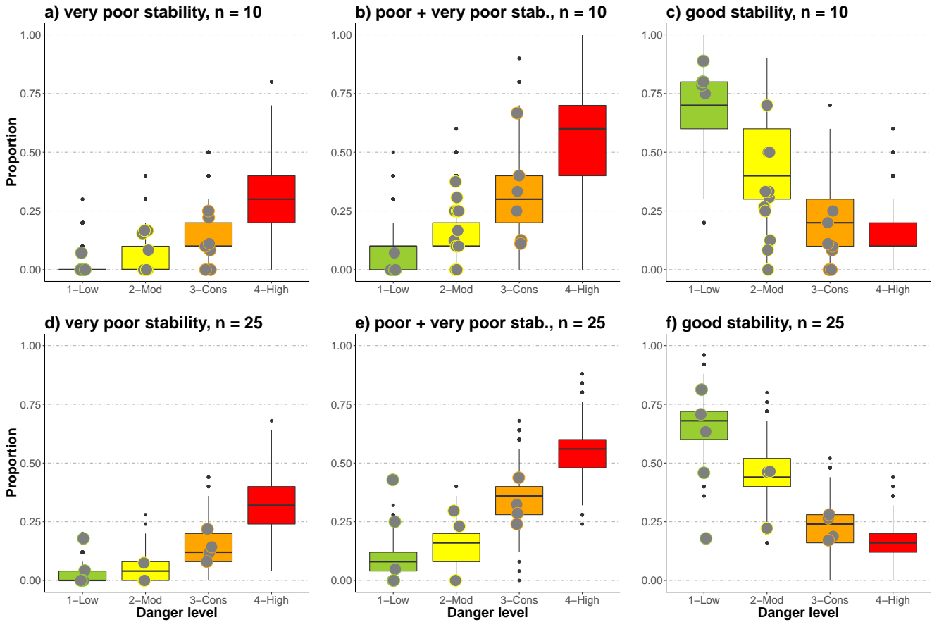
Figure 9. Comparison of observed (points, N = 41 ) and boot-strap sampled distributions (boxes) for the proportion of very poor (a, d), very poor and poor combined (b, e) and good stability tests (c, f), for two settings of the number n of tests drawn. When 7 to 15 RB tests were observed on the same day and within the same region, these are shown together with sampled distributions using n = 10 . When more than 16 tests were collected, these are shown together with sampled distributions using n = 25 . For n = 10 and good stability, the observed distributions were significantly different than the sampled distributions at 2-Moderate and 3-Considerable ( p < 0.05 , Wilcoxon rank sum test).
