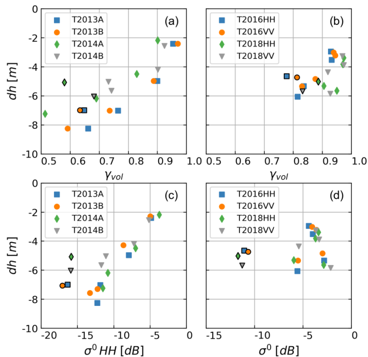
Figure 5. Relations between the elevation difference ( dh ) TDM - REMA and volumetric coherence (a, b), respectively the backscatter coefficient (c, d) for the snow pit sites P1 to P5. The framed points refer to P5.
