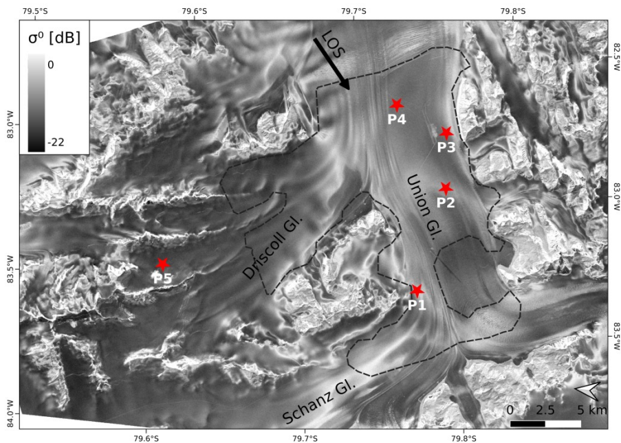
415 Figure 3. Section of TDM backscatter image, HH polarization, 6 May 2013. LOS (line of sight) indicates the radar look direction. The outline encloses the LGA.
