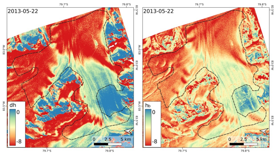
505 Figure 7. Elevation difference ( dh ) TDM DEM – REMA and elevation bias ( h_{bInV} ) by inversion of \gamma_{Vol} for the TDM scene 22 May 2013. The outline encloses the LGA.
