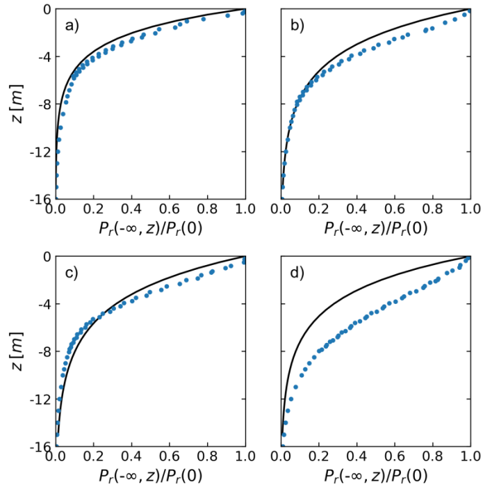
700 Figure A1. Fraction of X-band HH-polarized power scattered back from the snow/firn volume below the depth z . Points: RT model computations for individual layers. Curve: Model for exponential extinction. Input parameters refer to Union Glacier Pit 2 (a), Pit 3 (b), Pit 4 (c) and Pit 5 (d).
