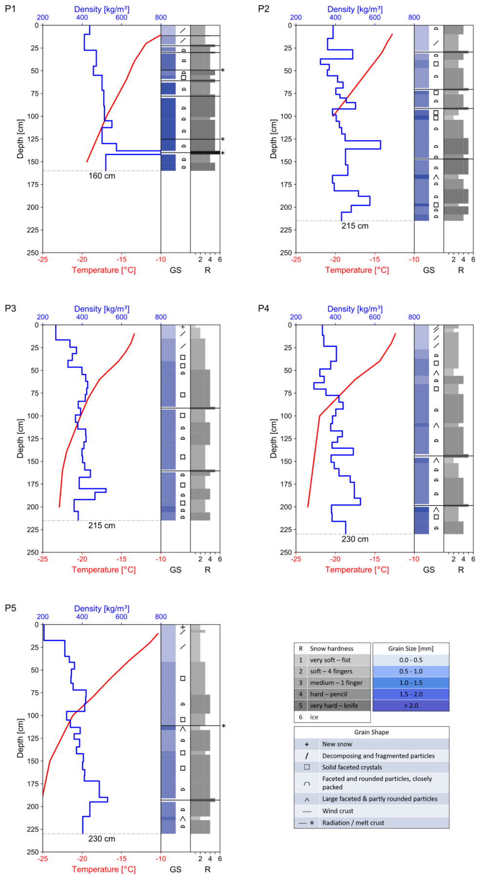
Figure 2. Vertical profiles of snow temperature, density, grain size (GS), grain shape and hand hardness (R) for snow pits P1 to P5 on Union Glacier, December 2016. The grain size refers to the maximum axis length of the prevailing snow grains.
