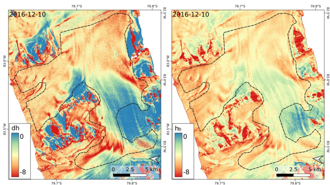
Figure 8. Elevation difference ( dh ) TDM DEM – REMA and elevation bias ( h_{bInV} ) by inversion of \gamma_{Vol} for the TDM scene 10 December 2016, based on HH and VV polarized data.
