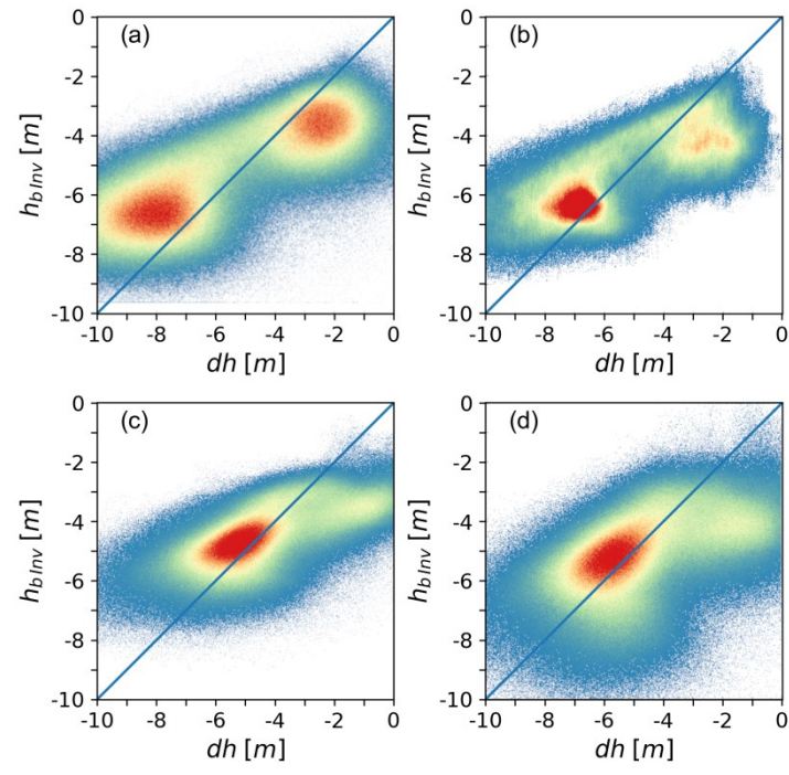
550 Figure 11. Scatterplot of the elevation difference TDM DEM minus REMA ( dh ) vs. the computed elevation by inversion of \gamma_{Vol}(h_{binv}) on Union Glacier LGA. (a) TDM scene 22 May 2013; (b) mean of the T2013 and T2014 scenes; (c) 10 December 2016 and (d) 10 January 2018, mean values of VV and HH channels. The line shows the 1:1 correspondence. The colour code represents the 2D data density.
