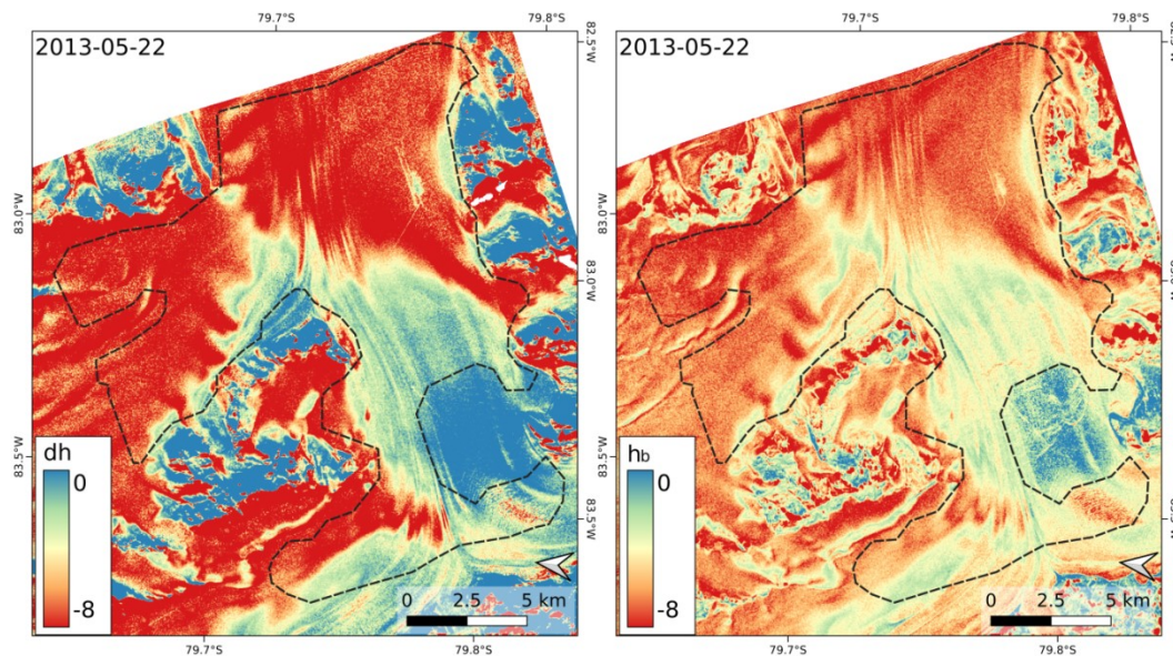
Figure 79. Elevation difference ( dh ) TDM DEM – REMA and elevation bias ( h_{bInv} ) by inversion of \gamma_{Vol} for the TDM scene 22 May 2013 ( \theta_i = 38.6^\circ ). The outline encloses the LGA.
