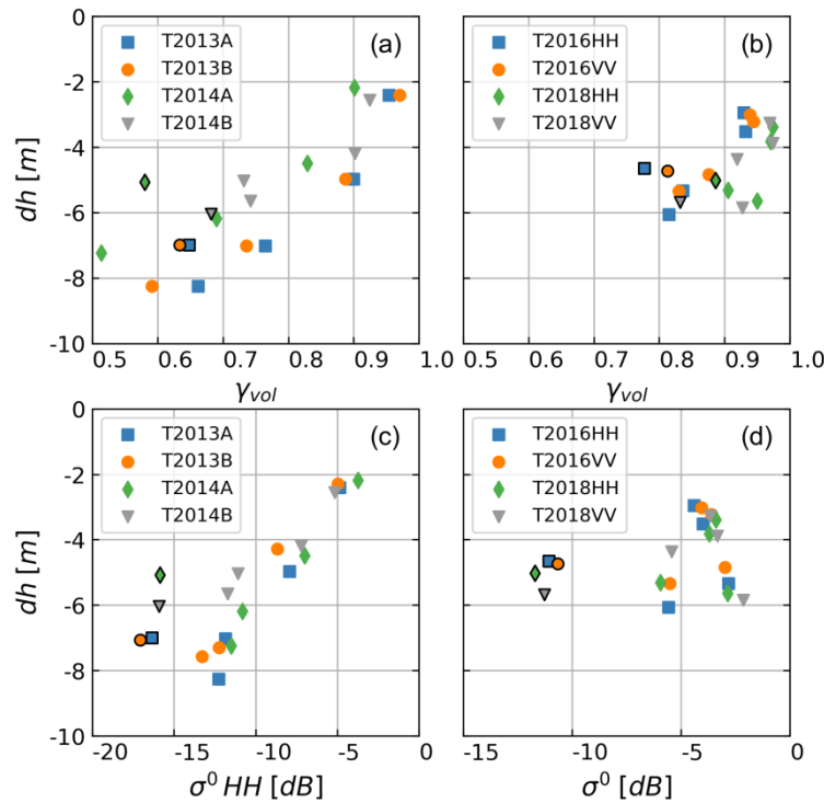
Figure 57. Relations between the elevation difference ( dh ) TDM - REMA and volumetric coherence (a); (b), respectively the backscatter coefficient (c); (d) for the snow pit sites P1 to P5. The framed points refer to P5. Incidence angle in the swath centre: (a) and (c) \theta_i = 37.5^\circ to 40.9^\circ , (b) and (d) \theta_i = 21.6^\circ and 22.1^\circ .
