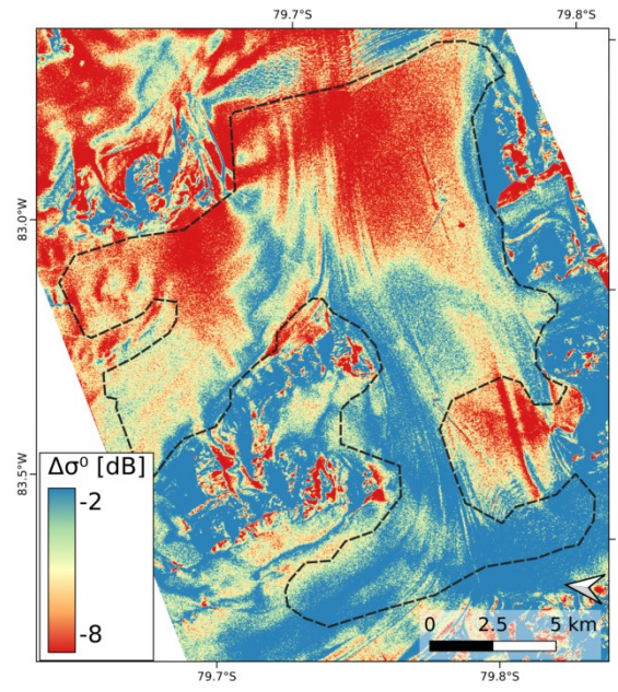
Figure 5. Difference of the HH-polarized backscatter coefficients between the TDM images from 6 May 2013 ( \theta_i = 40.9^\circ ) and 10 December 2016 ( \theta_i = 21.6^\circ ), \sigma_{HH}^{\circ 2013} \text{ minus } \sigma_{HH}^{\circ 2016} [dB].
