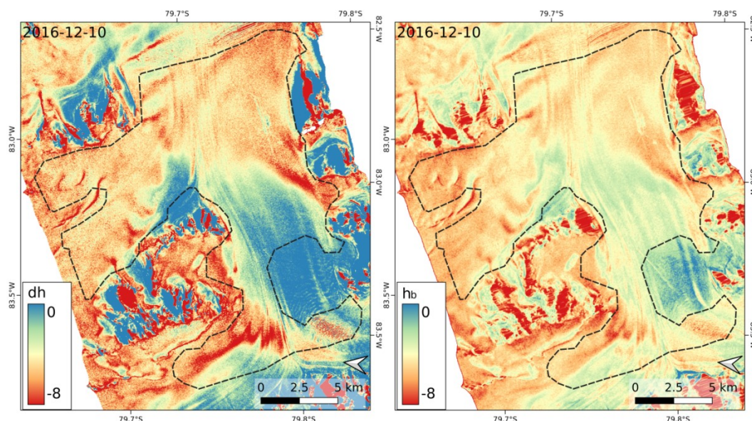
Figure 810. Elevation difference ( dh ) TDM DEM – REMA and elevation bias ( h_{bInv} ) by inversion of \gamma_{Vol} for the TDM scene 10 December 2016 ( \theta_i = 21.6^\circ ), based on HH and VV polarized data.
