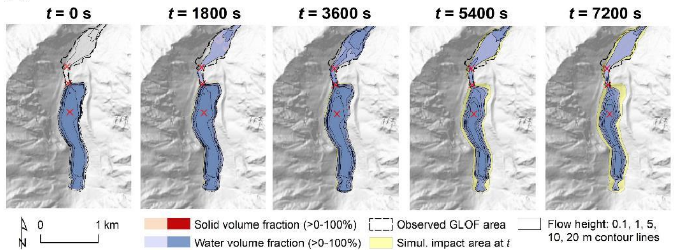
Figure 10. Evolution of flow height and GLOF impact area as well as solid and water volume fractions during the first two hours of the event, as simulated with r.avaflow for (a) Scenario A and (b) Scenario B. Only the section until the floodplain immediately downstream from the moraine dam is considered in these simulations. Base map is shaded relief map based on the DEM generated from Ziyuan-3 stereoscopic pairs and the simulation results.
