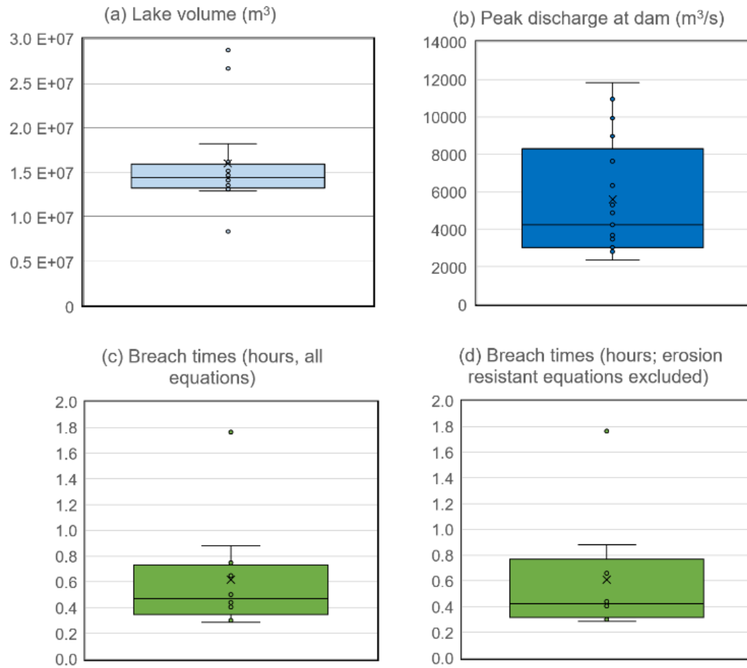
Figure 8. Lake, dam breach and flood parameters, derived from sets of published empirical relationships. (a) Volume of Jinwuco. (b) Peak discharge at the dam. (c) Breach time, considering all available equations. (d) Breach time, considering only those equations derived for easily erodible dams (an assumption we consider likely to hold for the dam of Jinwuco).
