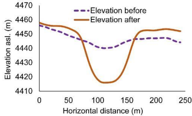
Figure 6. Breach of the moraine dam of Jinwucu. (a) Situation before and after the event of 26 June 2020, with difference in elevation between the DEMs derived before and after the event. (b) Cross section along the profile P (see (a)) before and after the event. Topographic base map is based on the DEM generated from Ziyuan-3 stereoscopic pairs.
