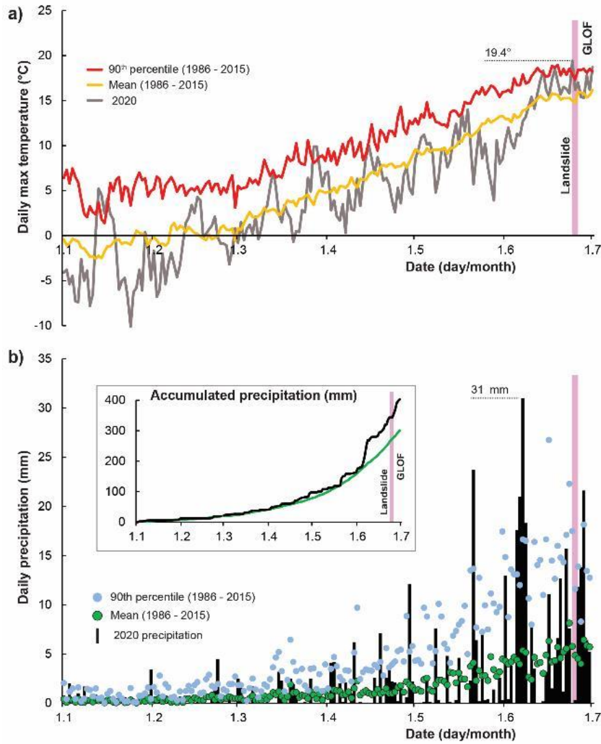
315 Figure 7. Meteorological conditions from January - June 2020, measured at the Lhari weather station, compared to the longer-term climatology (1986–2015).
