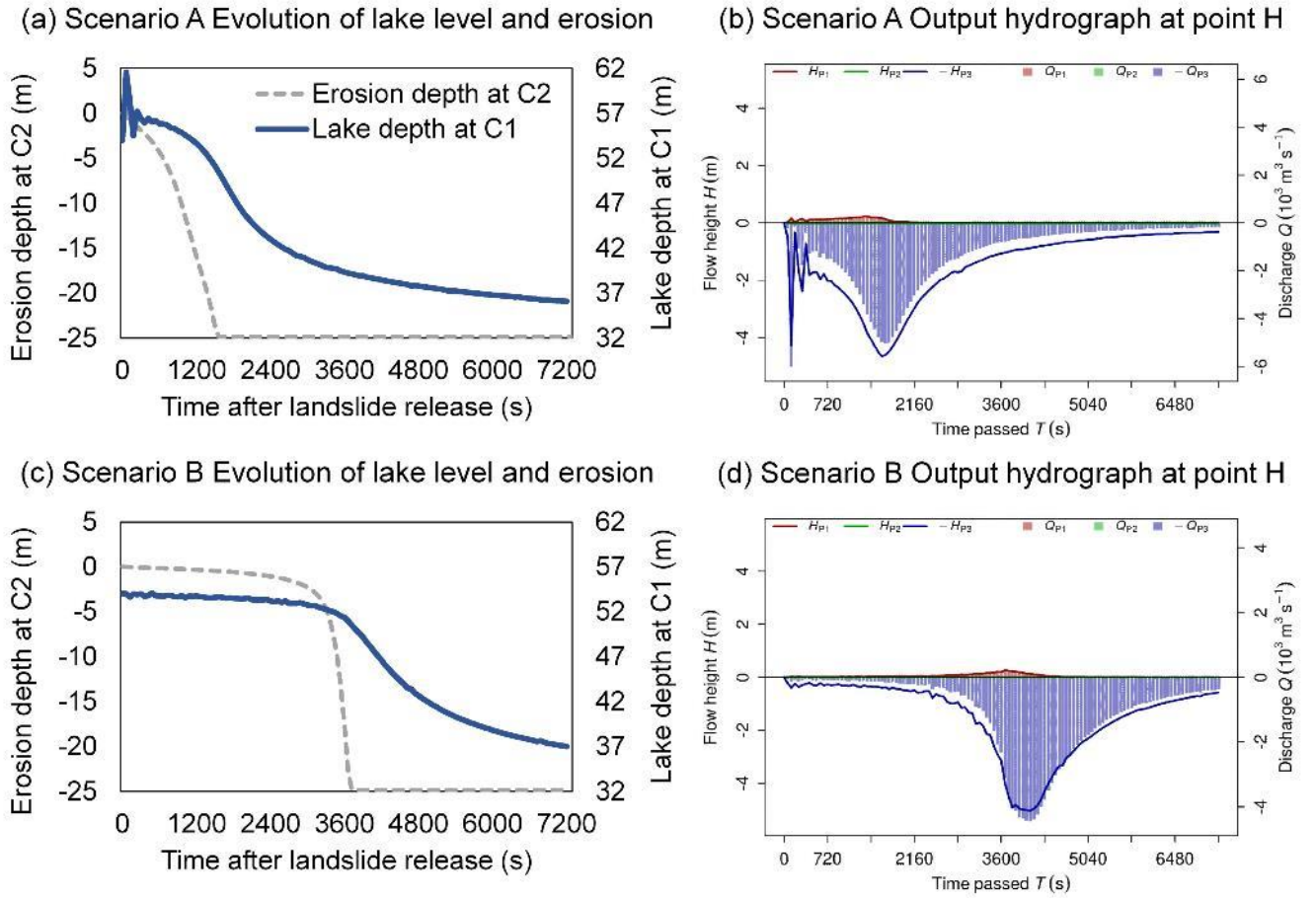
Figure 9. Dam breach as simulated with r.avaflow. (a) Scenario A, evolution of lake level and the erosion channel. (b) Scenario A, output hydrograph. (c) Scenario B, evolution of lake level and the erosion channel. (d) Scenario B, output hydrograph. Locations of the points C1, C2, and H are indicated in Figure 5 and Figure 11. In the output hydrographs, H means flow height, and Q means discharge. The subscript P1 refers to phase 1 (rock), P2 to phase 2 (not existent in this case), and P3 to phase 3 (water). Fluid discharge and flow height are plotted in negative direction for better readability.
