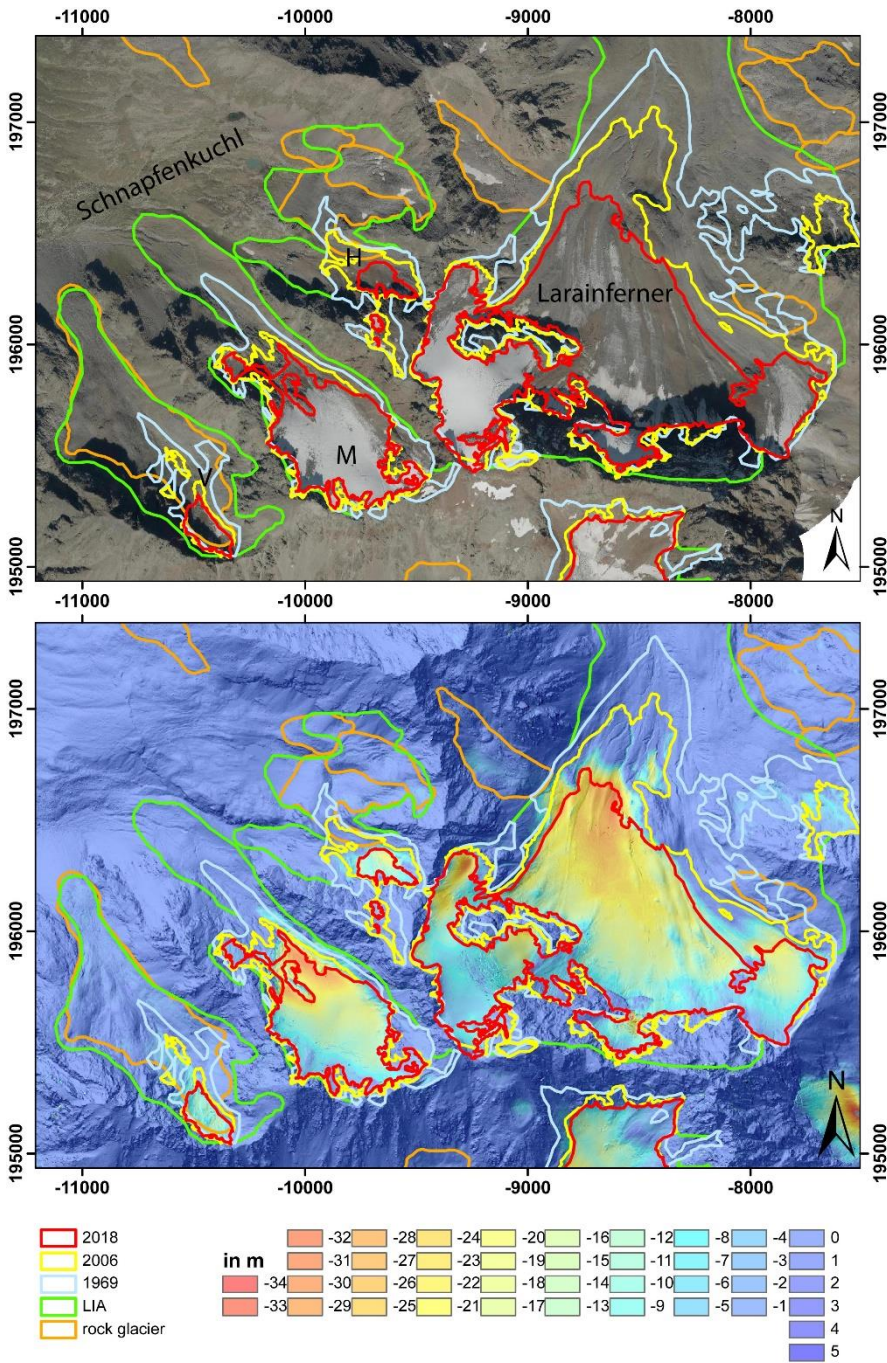
Figure 9: Final glacier outline 2018 and volume changes 2006-2018 for the Schnapfenkuchl glaciers V, M and H and Larainferner displayed on (A) the orthophoto from 2020 and (B) the elevation changes from 2006-2018 superimposed on the hillshade of 2018. Source orthophoto: CC 4.0 https://www.data.gv.at/katalog/en/dataset/orthofoto .
