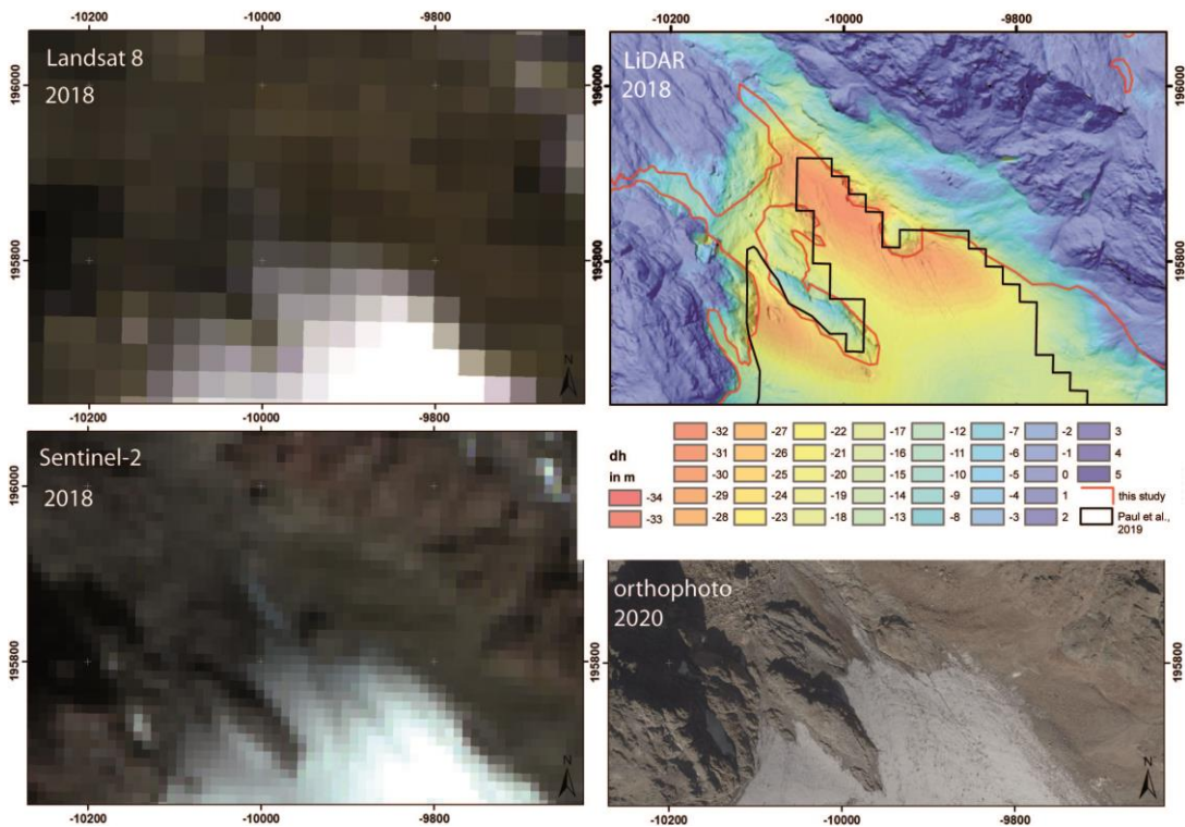
360 Figure 10: The comparison of the Landsat 8, Sentinel-2, LiDAR (hillshade and volume change 200620018, colour map as for Figure 9), all dating from 2018, and the orthophoto (2020) illustrate the different representation of the glacier in the various spatial resolutions for the snout of Schnapfenkuchl M. For glaciers with bare ice, glacier margins are clear at all scales of resolutions.
