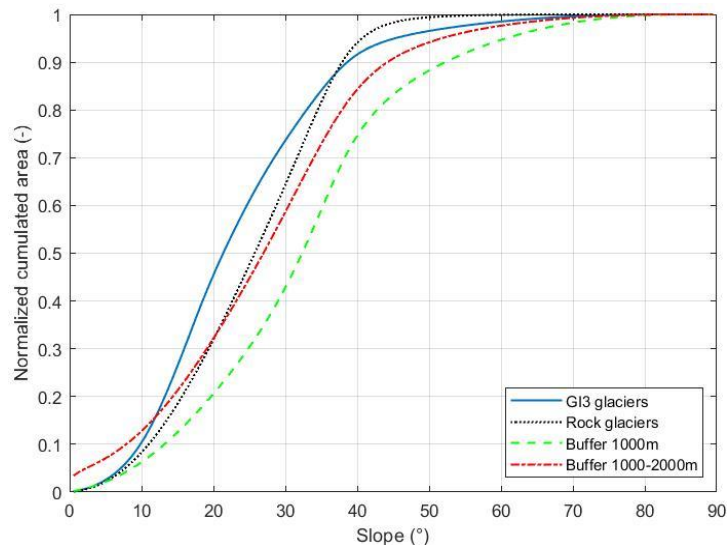
195 Figure 6: Distribution of slopes for glaciers, rock glaciers and the two buffer areas used for validation. The buffer regions are steeper than the glaciers, so that the elevation difference in the stable buffer zones can be considered an upper limit for the uncertainty.
