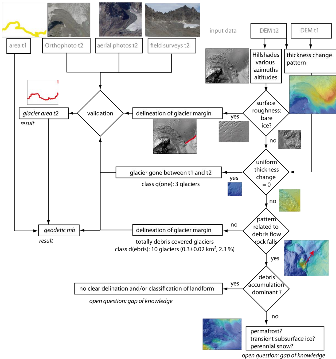
Figure 12: Summary of the workflow for high-resolution glacier mapping and mass balance calculation as applied in this study. The workflow does lead to quantitative results for most of the glaciers, but also shows up the need of scientific discussion where geomorphological processes other than ice melt contribute significantly to volume changes. See Figure 9 for the colour table of the volume change maps displayed.
