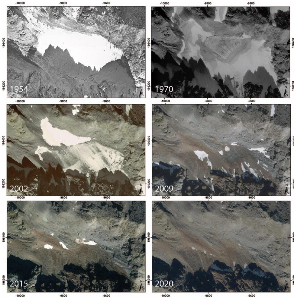
Figure 5: The evolution of Schnapfenkuchl glacier V in a time series of orthophotos from 1954 to 2020 illustrates that the evolution from a ‘classical glacier’ with crevasses as visible indicators of ice dynamics took just 20 years. In the orthophotos of 2009 and 2015, bare ice is still visible at the surface. Orthophotos: CC 4.0 https://www.data.gv.at/katalog/en/dataset/orthofoto
