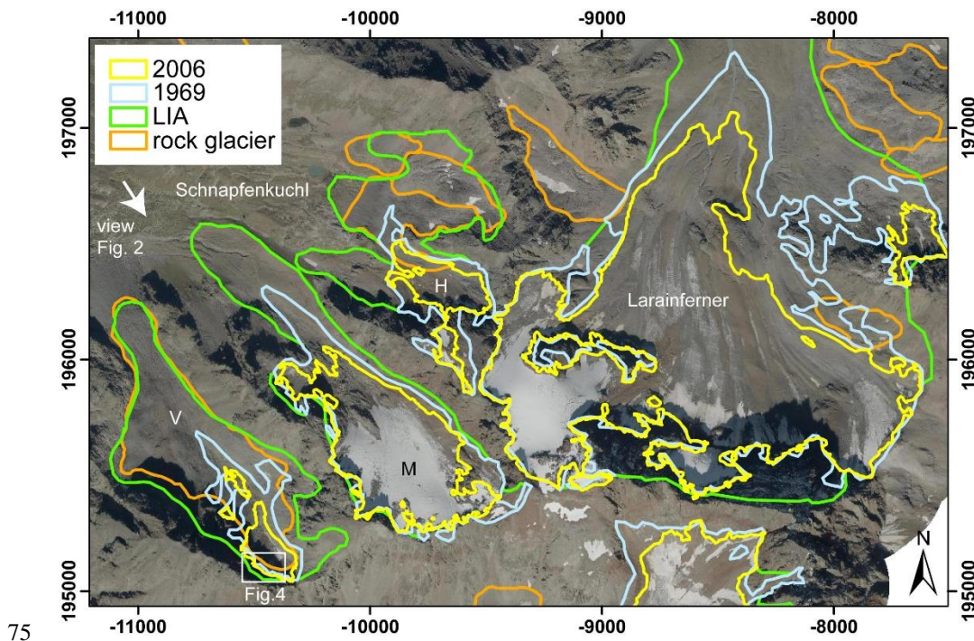
75 Figure 3: Overview of the Schnapfenkuchl glaciers V, M, and H in an orthophoto of 2020 with the information available prior to the new glacier inventory: the glacier margins of the former glacier inventories LIA, 1969 and 2006 and rock glacier margins (Krainer
