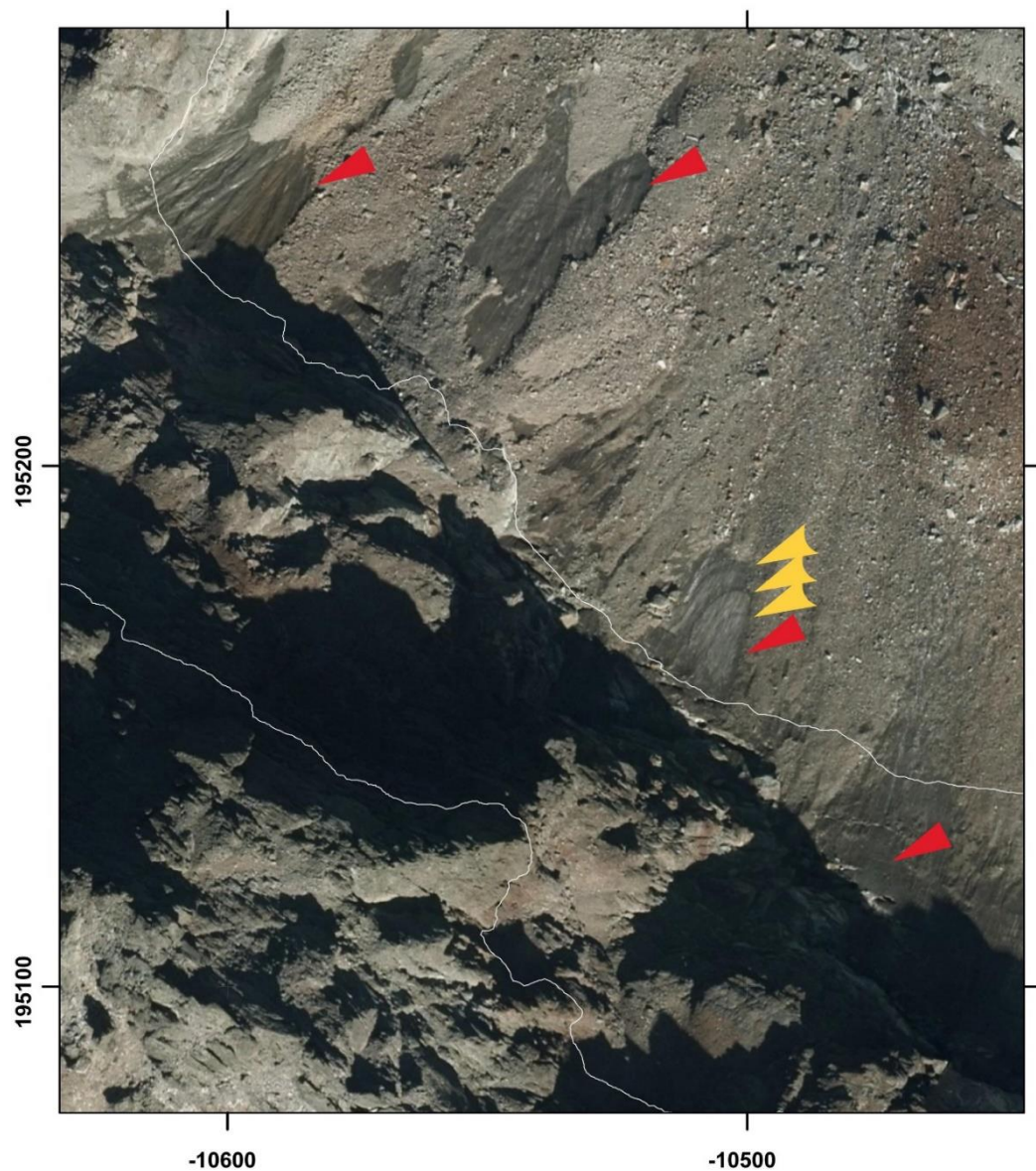
Figure 4: Bare ice exposed at Schnapfenkuchl glacier V in the orthophoto of 2015 (red arrows), with stratigraphic layers (yellow arrows) indicating sedimentary ice or firn. Orthophotos: CC 4.0 https://www.data.gv.at/katalog/en/dataset/orthofoto
