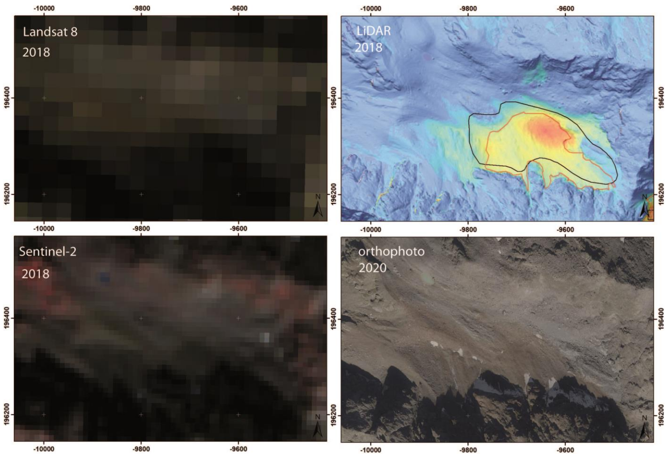
Figure 11: Representation of the debris-covered glacier Schnapfenkuchl H in the Landsat 8, Sentinel-2, LiDAR images 365 (hillshade and volume change 200620018, colour map as for Figure 9) and the orthophoto. The manual delineation of glacier outlines (red: based on LiDAR, black: based on Sentinel-2, Paul et al., 2019) is consistent for both methods.
