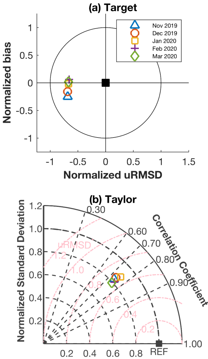
940 Figure 6. Target diagram (a) of normalised bias and normalized unbiased root-mean-square difference (uRMSD) and Taylor 945 diagram (b) of normalised standard deviation and correlation between the RASM sea ice thickness simulations and 950 CryoSat2/SMOS data from November 2019 to March 2020. The square marker indicates the reference (REF) value, i.e., perfect model.
