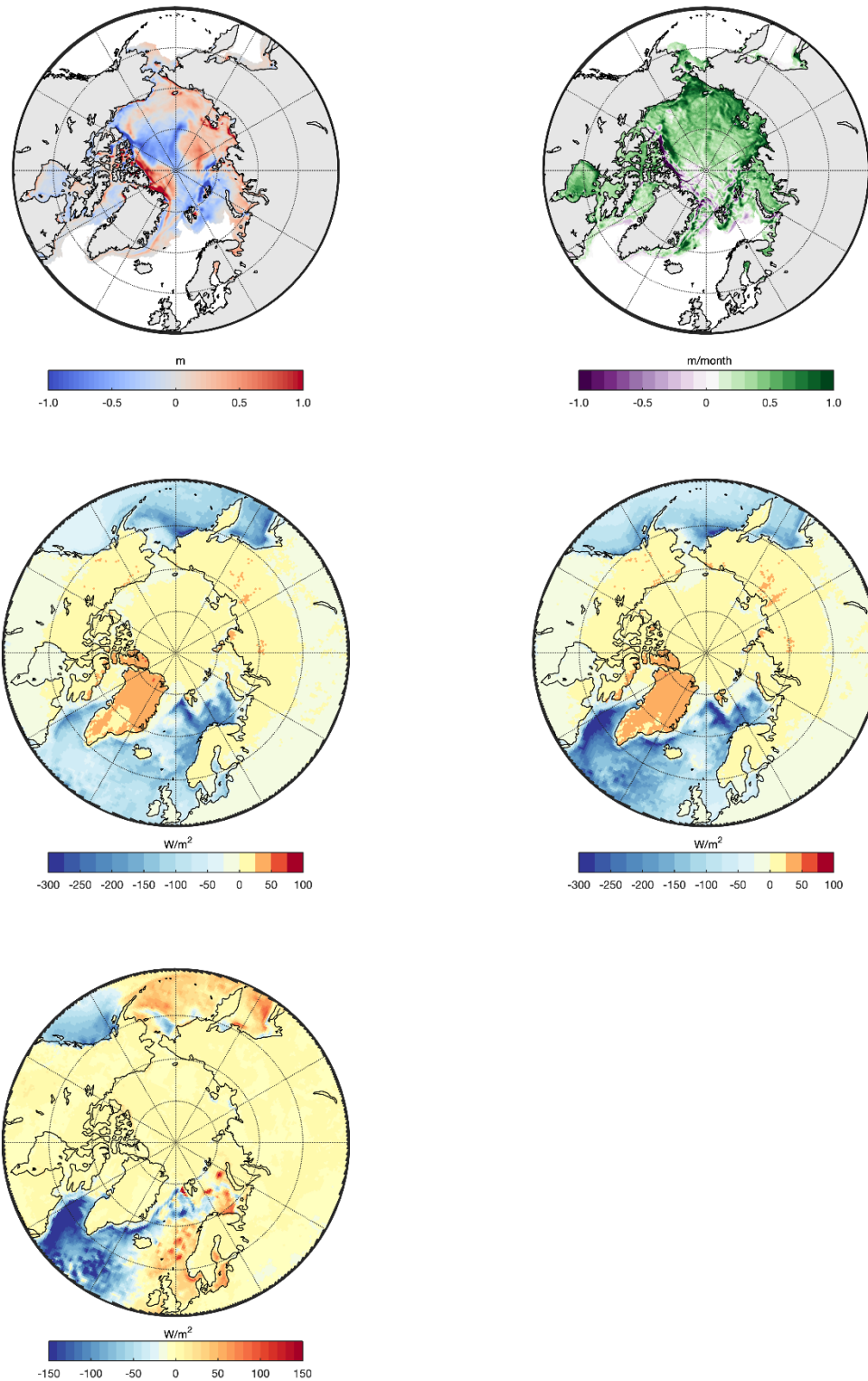
Figure 16. The differences of SIT (upper row, left) and total volume tendencies (upper row, right) “JFM 2010 minus JFM 1045 2020” and the mean combined sensible and latent heat fluxes ( W/m^2 ) for JFM 2010 (middle row, left) and for JFM 2020 (middle row, right) and the differences of the surface heat fluxes “JFM2020 minus JFM 2010” (lower row) from the RASM hindcast simulation. Note that the flux convention means, that negative fluxes are from the ocean into the atmosphere.
