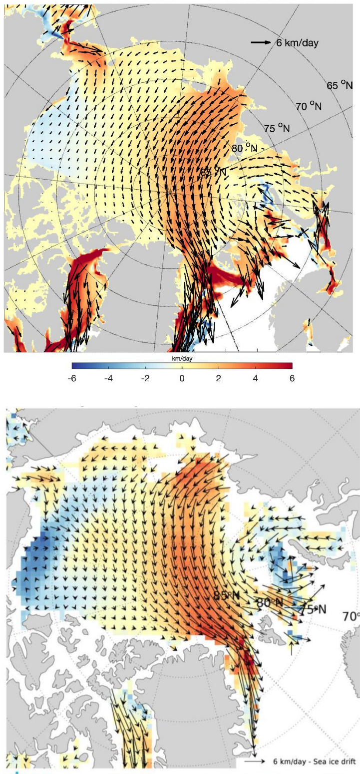
Figure 11. RASM simulations of sea ice velocity anomaly (top) and satellite derived sea ice velocity anomaly (km/day) (bottom) for January 2020-March 2020 compared to the climate mean 2010-2019.
