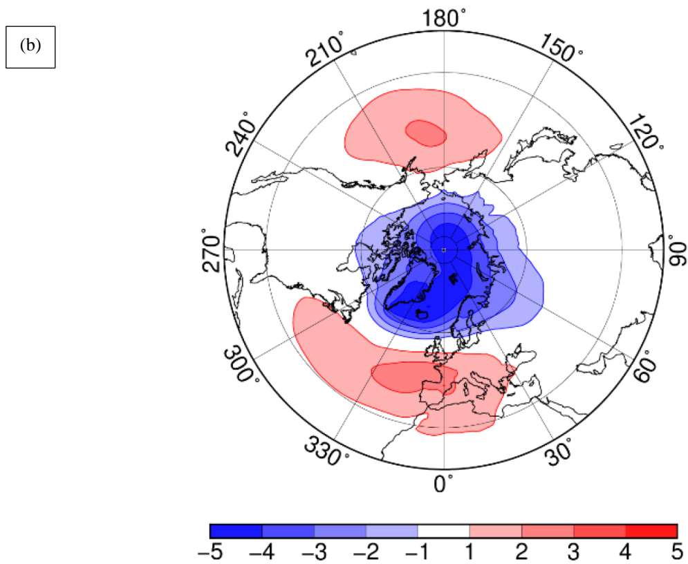
900 Figure 1: (a) Time series of daily values of the AO index from October 2019 to April 2020 (black line) with 7-day running mean (red line) and (b) the spatial AO pattern from 1979-2000 based on ERA5.
