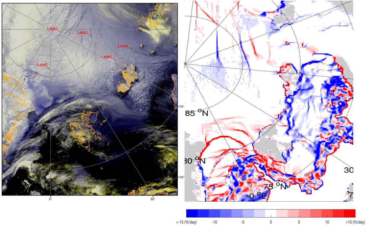
975 Figure 9. Sea ice lead structures in data from infrared channel 5 of the NOAA-20 satellite with the highest possible resolution (375 m) on 5th March 2020 with identification of leads. These data were obtained using the VIIRS instrument (Visible / Infrared Imager Radiometer Suite), installed on board the NOAA-20 satellite (left). Daily mean sea ice divergence (%/day) on 5 th March 2020 in the RASM simulation (right). No data manipulation was done except the daily averaging.
