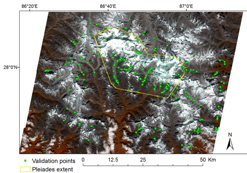
Fig. 2 The Khumbu test region in Nepal showing the RapidEye image of Oct 9, 2015 (bands 5, 4 and 3) and the Pleiades image of Oct 7, 19 and 20, 2015 (bands 4, 3 and 2) (yellow dotted outline). Vegetation appears in dark red; ponds display various shades of turquoise. Green dots represent the ground truth points digitized on the high-resolution images and used for the accuracy assessment of the linear spectral unmixing.
