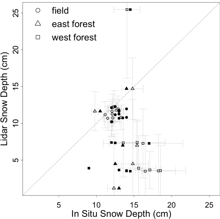
275 Figure 3. Comparison between the magnaprobe (gray fill) and snow tube (black fill) versus the lidar snow depth measurements by location. The mean and 95% confidence intervals were calculated using the five magnaprobe snow depths and the lidar snow depths, equation 1, averaged over a 0.4 x 0.4 m grid cell. Single snow tube snow depth measurements are shown without confidence intervals.
