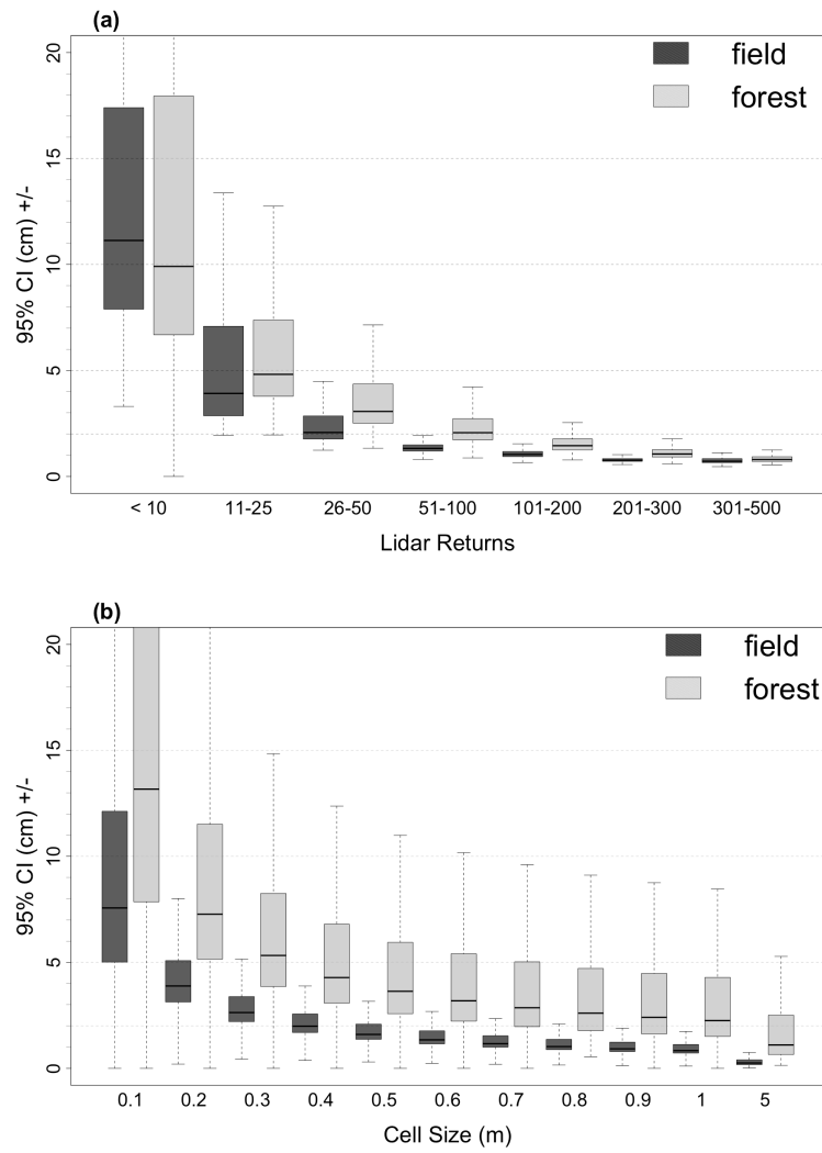
340 Figure 7. One sided confidence intervals of the mean snow depth values in the field and forest at Thompson Farm, Durham, NH on January 23, 2019 from the individual cells for 1 m 2 cells by land cover and point cloud density (a) and for grid resolutions ranging 0.1 to 5 m (b). Boxplots show the lower quartile, median, upper quartile, and whiskers.
