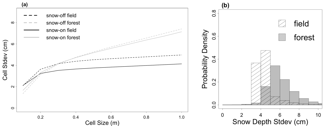
Figure 8. Lidar surface elevation standard deviations by (a) cell size and land cover. Cell standard deviations are the average of the individual cells standard deviation values calculated for cells with side dimensions ranging from 0.1 to 1.0 m. (b) Probability density function of the pooled snow depth standard deviation for each 1 m 2 cell in the forest (gray) and field (hashed).
