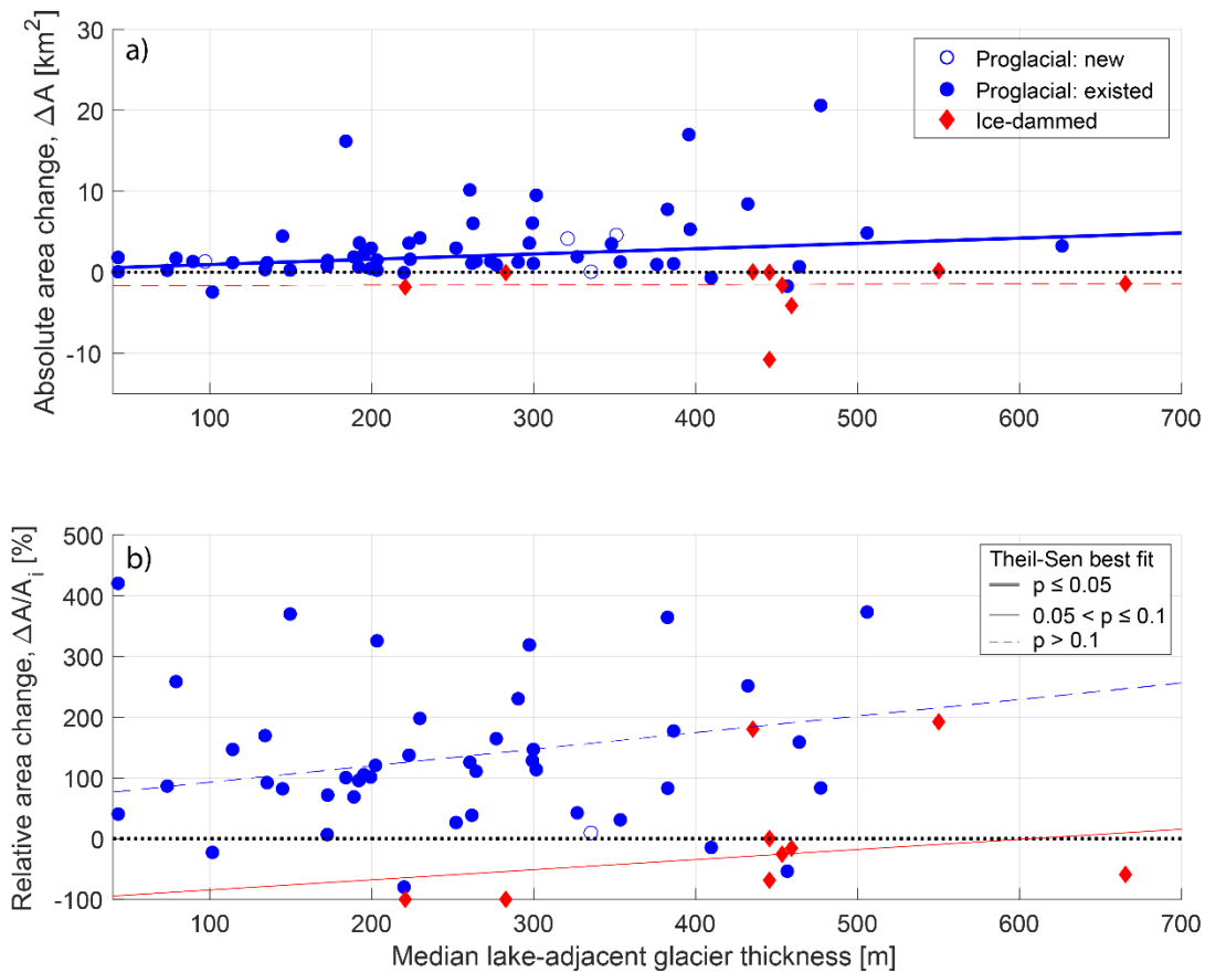
460 Figure 6. (a) Absolute and (b) relative lake area change as a function of median lake-adjacent glacier ice thickness (see Section 2.3) for proglacial (blue circle) and ice-dammed (red diamond) lakes. On both panels, lines show the linear fit to proglacial (blue) and ice-dammed (red) lakes as estimated to by the non-parametric Theil-Sen robust line. Thick solid lines show relationships that are significant at the p \leq 0.05 level, thin solid lines show 0.05 < p \leq 0.1 relationships, and thin dashed lines show p > 0.1 relationships. All significance values are estimated by the Kendall rank correlation test. The black dotted line shows zero lake area change. Unfilled symbols indicate lakes that appeared during the study period.
