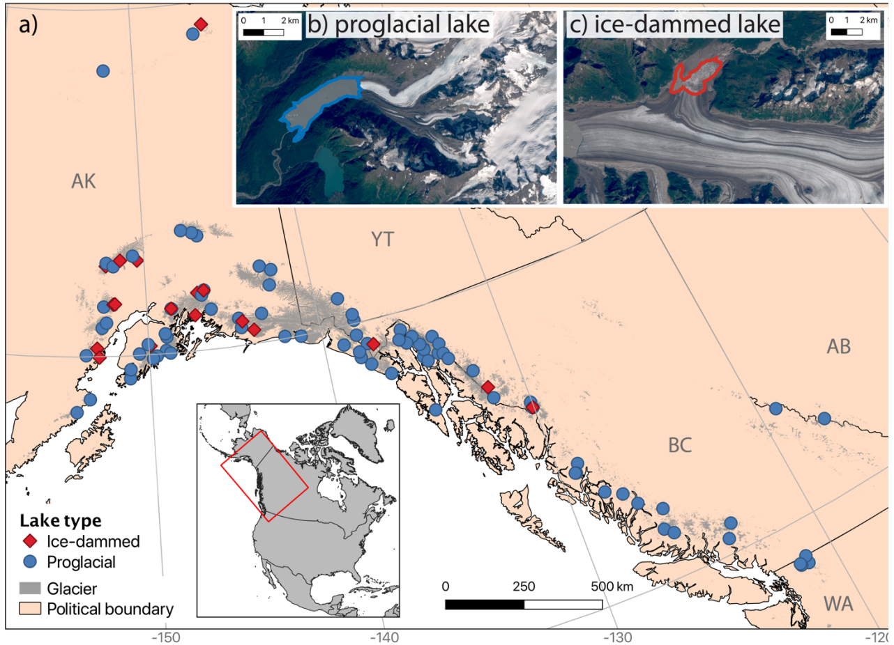
140 Figure 1. a) Map of study region showing sampled proglacial (blue circles) and ice-dammed (red diamonds) lakes. Glacier extent is shown as gray fill (RGI, 2017) and black lines indicate political boundaries. Two-letter state and province abbreviations are given in gray text. The inset map shows the location of the study area (red box) in northwestern North America. Examples are shown of b) a proglacial lake (Unnamed lake downstream from Twentymile Glacier; 60.94 N, -148.78 E) and c) an ice-dammed lake (Van Cleve Lake dammed by Miles Glacier; 60.70 N, -144.41 E). Background imagery in b) and c) is from Landsat 8.
