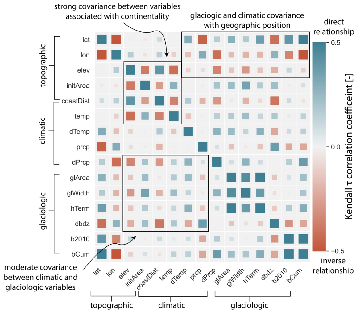
550 Figure 10. Correlation matrix showing interrelatedness of the topographic, climatic, and glaciologic variables used for lake area change correlations (Table 2). Symbol color scales with the Kendall tau correlation coefficient between the environmental variables associated with that point's row and column. Symbol size scales with the absolute value of the correlation coefficient. Black boxes highlight covarying environmental variables that are discussed in the text. Meanings for variable names are as follows: lat = latitude; lon = longitude; elev = lake elevation; initArea = lake initial area; coastDist = distance from the open ocean; temp = JJA temperature; dTemp = change in JJA temperature; prcp = DJF precipitation; 555 dPrpc = change in DJF precipitation; glArea = area of the lake-adjacent glacier; glWidth = width of that glacier; hTerm = lake adjacent median ice thickness; dbdz = mass balance gradient; b2010 = average annual mass balance for 2010 – 2016; bCum = cumulative mass balance for 1980 – 2016.
