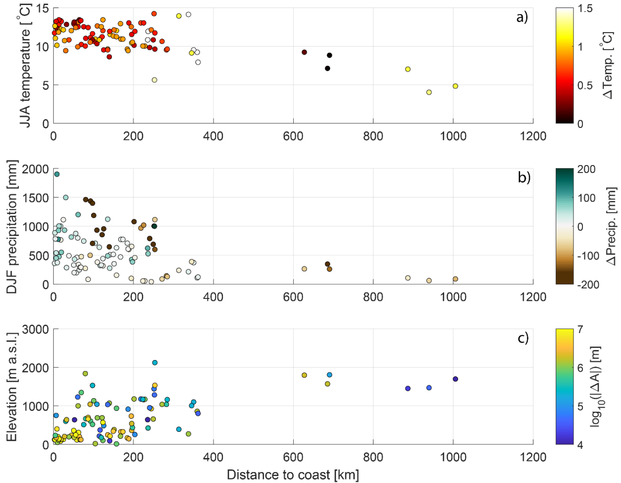
525 Figure 9. Variation in climatic and topographic variables as a function of a lake’s distance from the open ocean. (a) Summer air temperature (y axis) and its change (colors) between the 1960s and 2000s. (b) Winter precipitation (y axis) and its change between the 1960s and 2000s. (c) Lake elevation (y axis) and absolute lake area change between the 1984 and 2018.
