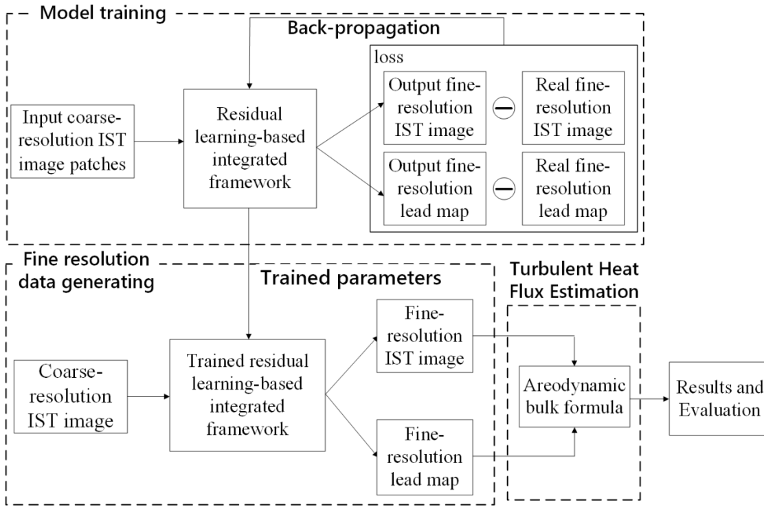
Figure 4. The flowchart of the subpixel-scale TXF estimation using the proposed deep residual convolutional neural network-based framework. Note: IST denotes the ice surface temperature.
