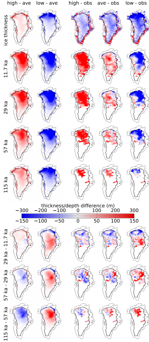
Figure A1. Composite ice thickness and isochrone depth for simulations with high ( -0.1 to -0.05 \text{m yr}^{-1} ) and low ( 0.15 to 0.2 \text{m yr}^{-1} ) values of \Delta P_{\text{hoi}} , compared to the ensemble average and observations. A thin black line marks the 1000 m surface elevation.
