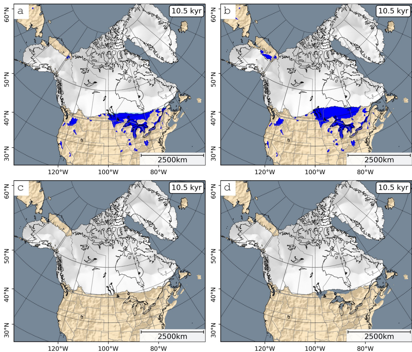
Figure S21: Overview map at 10500 kyr for the different experiments: a) LCC, b) LNS, c) Ctrl and d) Def.
