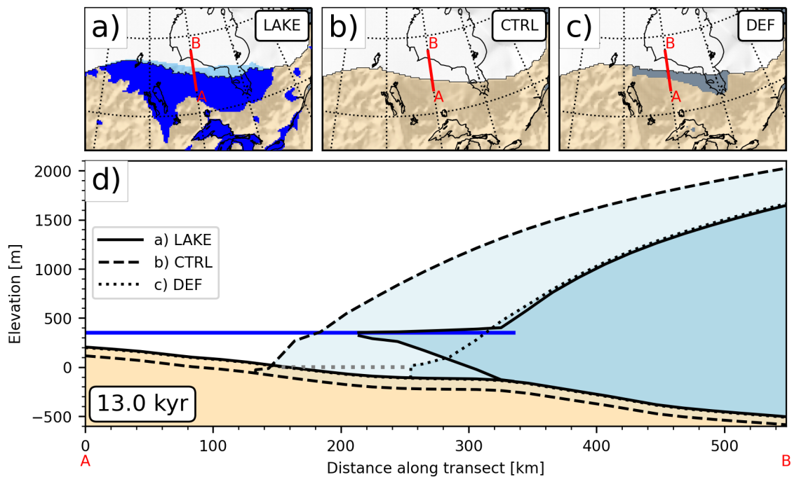
Figure 9. Profiles of the ice sheets of the (a) standard lake (LCC) LAKE , (b) standard no lake (Ctrl) CTRL and (c) PISM default (Def) DEF experiments at 13 kyr. The transects shown in (d) are along 90^{\circ}\text{W} , between 53^{\circ}\text{N} (A) and 58^{\circ}\text{N} (B) and are marked in the upper panels by a red line. In panels (a) - (c) ice shelves are shown in light blue, lakes in blue, and ocean in gray. The blue line in panel (d) marks the lake level elevation in the LAKE experiment, while the gray line marks the sea level elevation of the DEF experiment.
