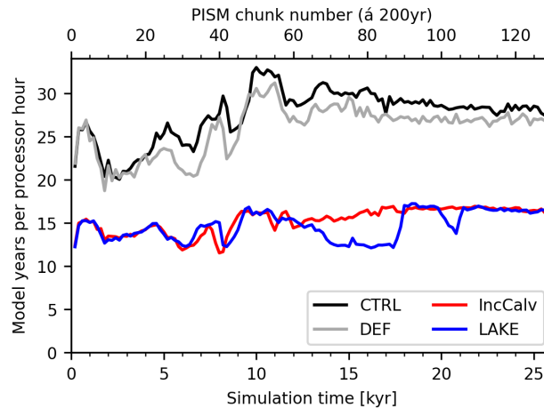
Figure C1. The plot shows the efficiency of PISM in model years per processor hour averaged over 200 yr chunks for the different experiments: Ctrl CTRL – no lakes but with the SL2DCC model to prevent inland ocean basins; Def DEF – PISM default, no lakes, no advanced ocean treatment; LCC LAKE – standard lake experiment; LNS IncCalv – lakes, but strong-increased strongly-increased calving to-reduce-threshold-such-that to-reduce-threshold-such-that ice shelf-formations shelves are effectively removed (for more details see supplementary material) . variability Variability is mainly due to the adaptive time stepping mechanism of PISM which hits especially hard when big ice shelves are present. A maximum time step of 0.25 yr is used for all experiments.
