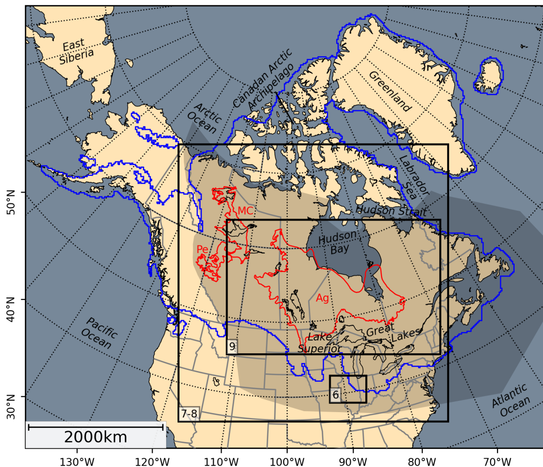
Figure 3. Map giving an overview of the experiment domain of the current study. Present day coastline and the major North American lakes are shown in black, whereas Canadian and U.S. American states political boundaries are gray. The outlines of selected palaeo proglacial lakes are shown in red: Ag — Lake Agassiz/Ojibway (Teller and Leverington, 2004), MC — Lake McConnell (Smith, 1994) and Pe — Lake Peace (Mathews, 1980; Hickin et al., 2015). Initial ice extent at LGM (Gowan et al., 2016) is shown in blue. Black rectangles visualize the map sections discussed in the text (the numbers refer to the respective figures). The shaded area shows the regions attributed to the (continental) Laurentide Ice Sheet (LIS) in this study.
