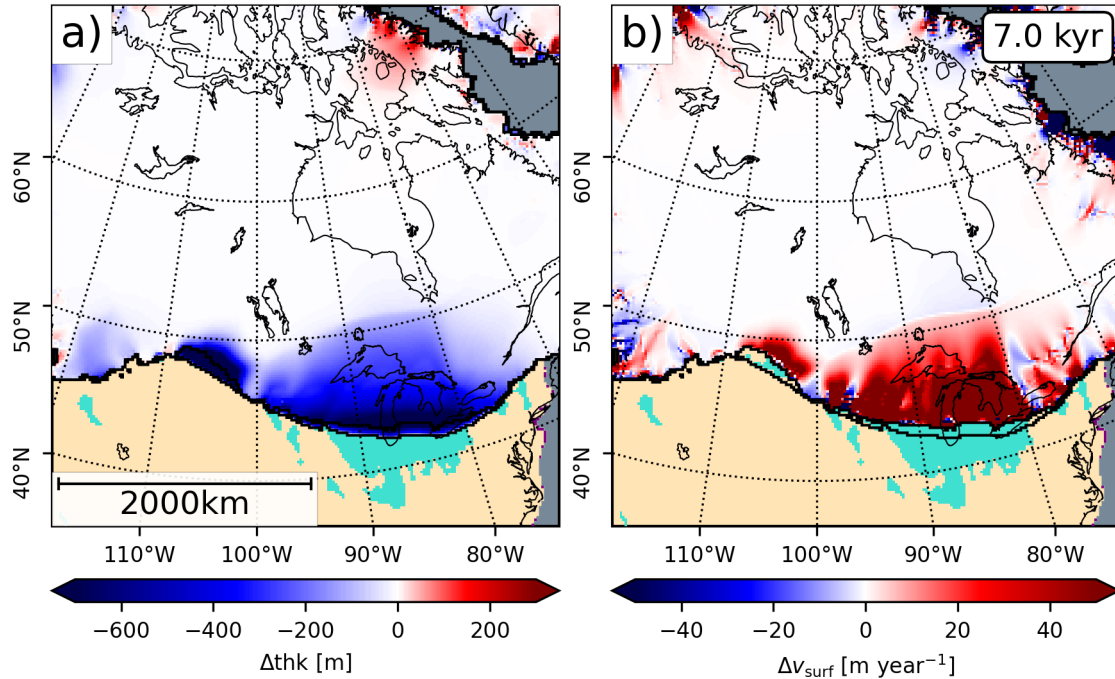
Figure 7. Comparison of the standard-lake (LCC)-LAKE and no-lake (Ctrl)-CTRL experiments at 7 kyr. Both plots show anomalies ( LCC LAKE - CtrlCTRL ) of (a) ice thickness and (b) surface velocity. Formation-Acceleration of ice streams-flow at the proglacial lake boundaries and the resulting impact on ice geometry can clearly be seen. Ice margins of both simulations are shown in black.
