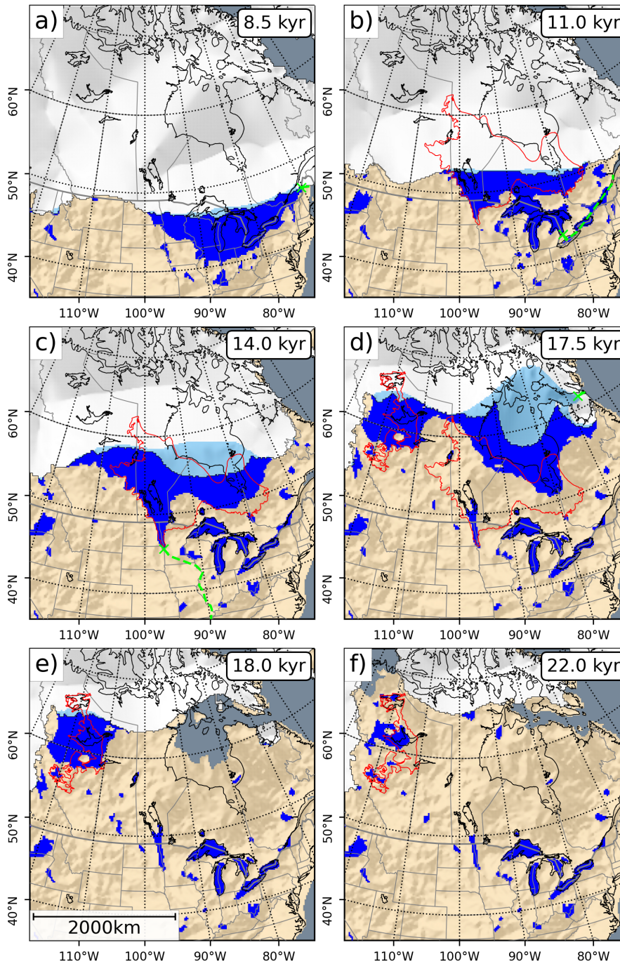
Figure 8. Snapshots for different stages of the lake-LAKE experiment (LCC). Ice-Lacustrine ice shelves are shown in light blue. The red outlines show the maximum extent of selected palaeo lakes (Fig. 3). Modeled spill point and drainage routes for Lake Agassiz are shown in green in panels a-d.
