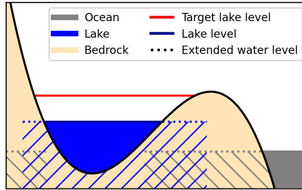
Figure 1. Sketch of the PISM LakeCC and SL2DCC models. The target water level indicates the maximum water height of a lake basin before it overflows into the ocean . The actual lake level, as it is seen from the rest of the ice model, is slowly raised (or lowered) towards the target level. The dotted lines and hatched areas indicate where the respective water levels extend into the bedrock ground . To prevent the formation of inland ocean basins, the SL2DCC model sets the sea level in those basins to invalid. Note that lake level and the gap in the sea level field are extended by one cell, respectively. For details on this the reader is referred to the main text.
